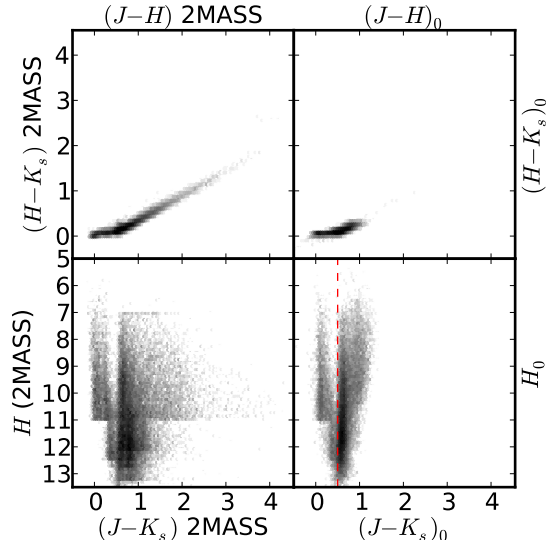
Figure 8. Two-dimensional histogram of the APOGEE DR10 stars in (top) 2MASS JHK_s color space; and (bottom) 2MASS H vs. J - K_s . The left column shows observed magnitudes and colors from 2MASS, while the right column has been dereddened based on H - 4.5 \mu\text{m} color as in Zasowski et al. (2013). The vertical dashed line at (J - K_s)_0 = 0.5 shows the selection of the main APOGEE red giant sample; bluer objects include telluric calibration stars, data taken during commissioning, and ancillary program targets. The grey scale is logarithmic in number of stars.
