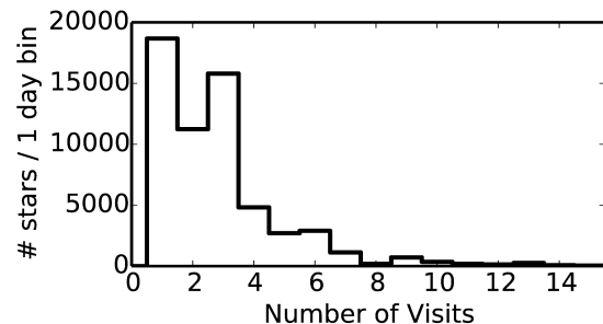
Figure 4. The distribution of number of spectroscopic visits for APOGEE stars included in DR10. While the bulk of stars have three or fewer visits, they may have reached our spectral S/N requirement if they are bright enough; see Figure 7.
