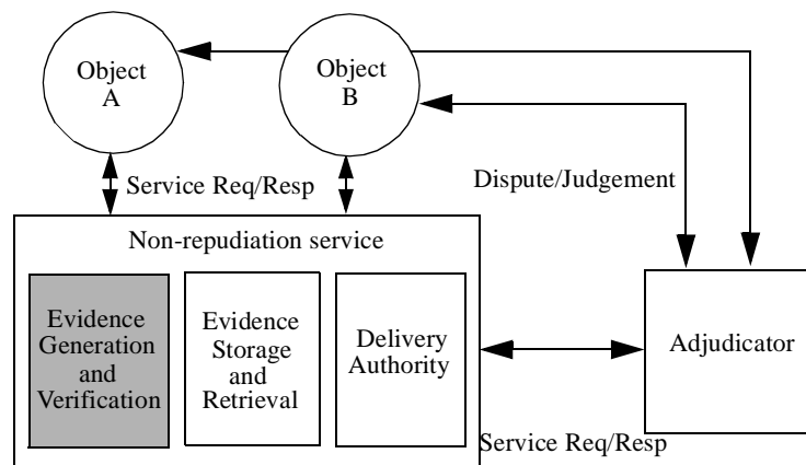
Figure 2-15 Non-repudiation Services
