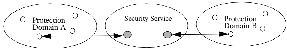
Figure 2-27 Object Encapsulation
