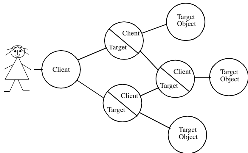
Figure 2-8 Delegation Model
