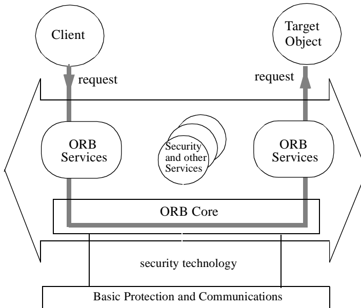
Figure 2-22 Structural Model
