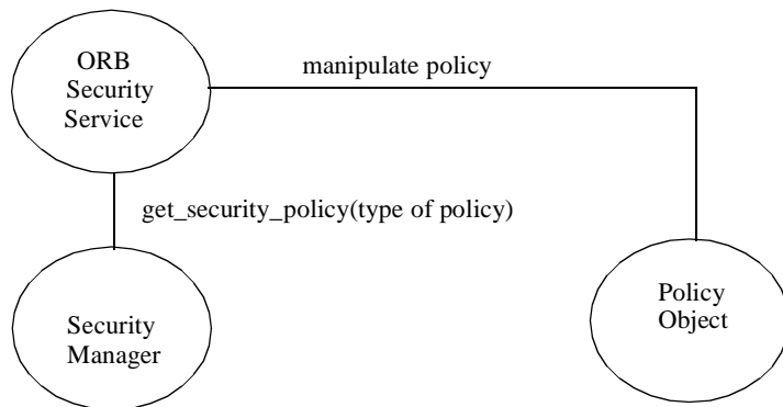
Figure 2-46 get_security_policy Operation
