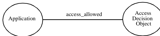
Figure 2-35 access_allowed Application
