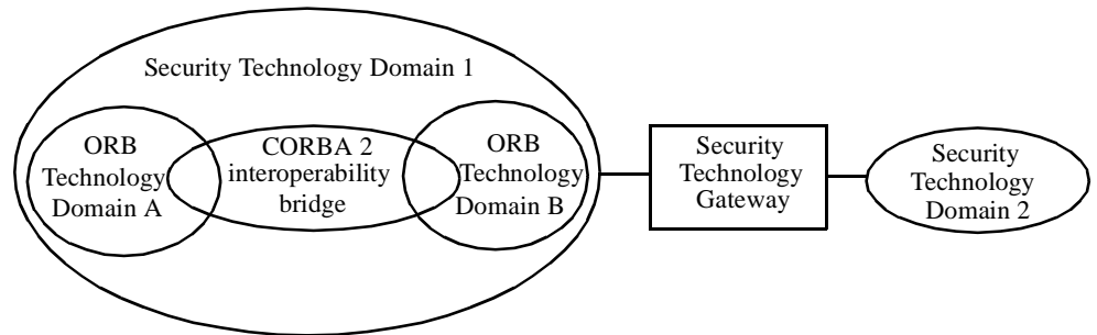
Figure 2-21 Framework of Domains
