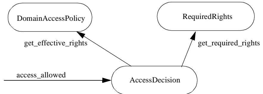
Figure F-1 Intended Use by AccessDecision
