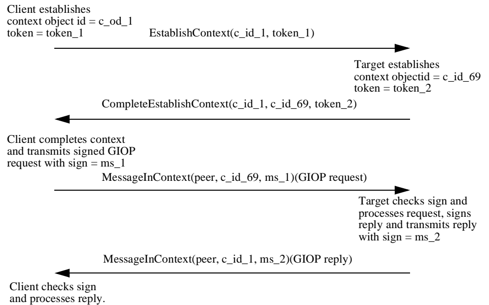
Figure G-1 Mutual Authentication
