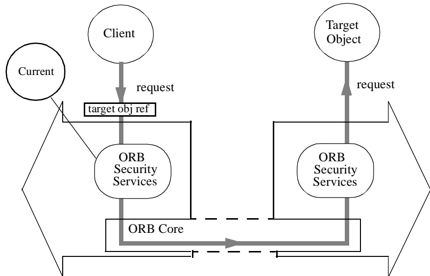
Figure 2-31 Making a Secure Invocation
