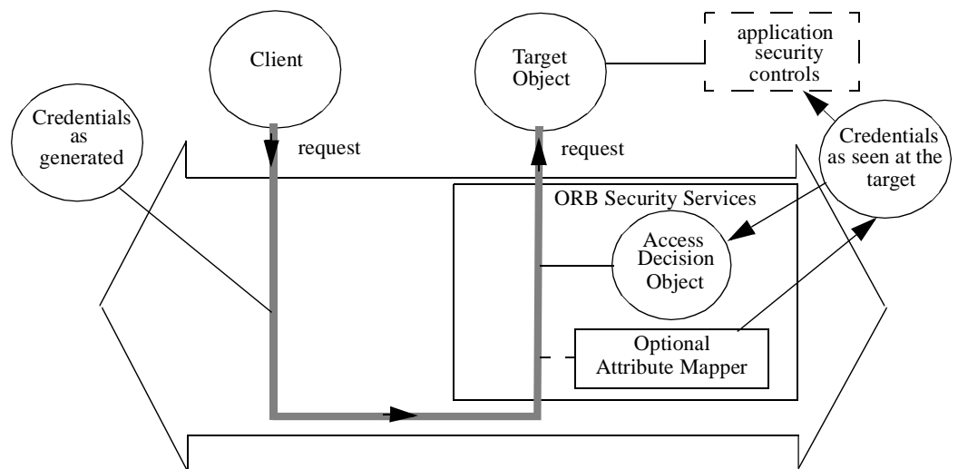
Figure 3-3 Attribute Mapper Diagram
