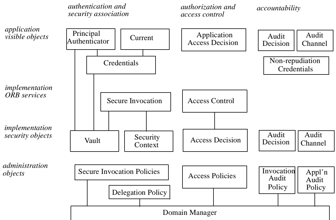
Figure 2-51 Relationship Between Main Objects
