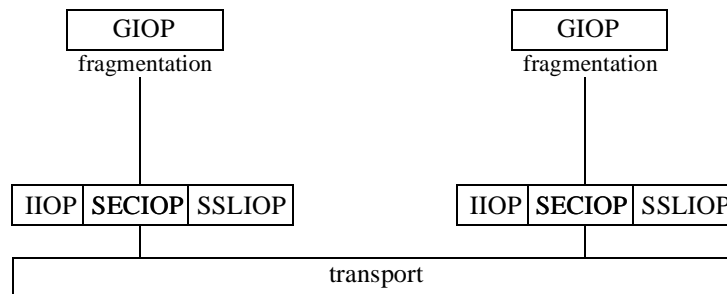
Figure 3-4 Position of SECIOP Protocol
