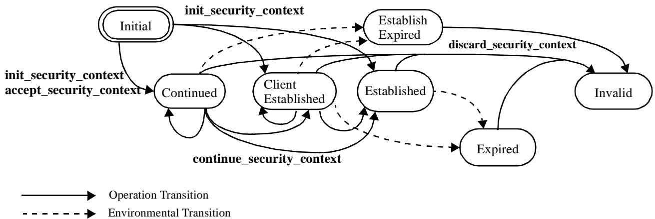
Figure 2-53 Security Context State Transition Diagram
