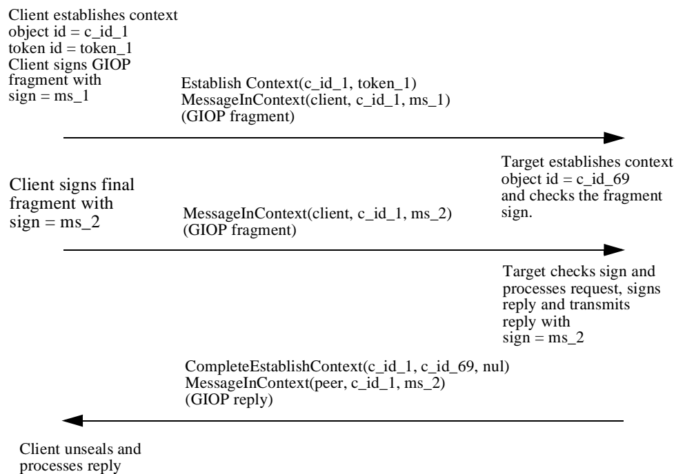
Figure G-3 Fragmented GIOP Request with Context Establishment
