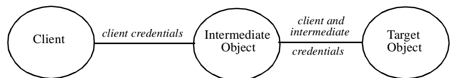
Figure 2-11 Composite Delegation
