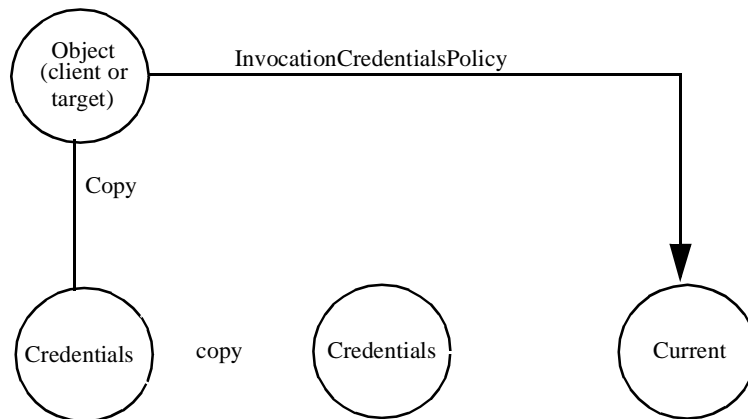
Figure 2-29 Multiple Credentials
