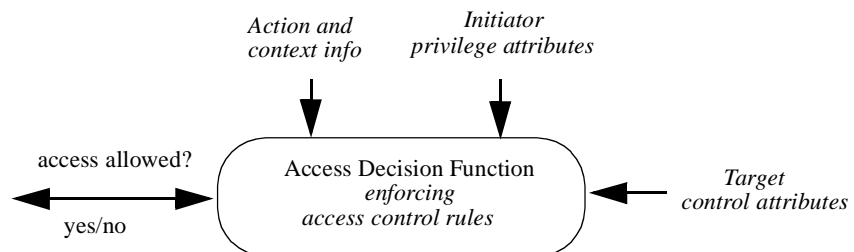
Figure 2-6 Authorization Model
