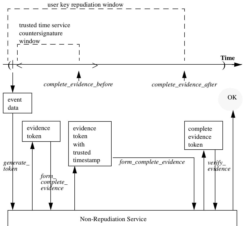
Figure 2-41 Non-repudiation Service
