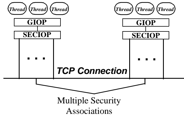
Figure 3-5 Architectural Assumptions
