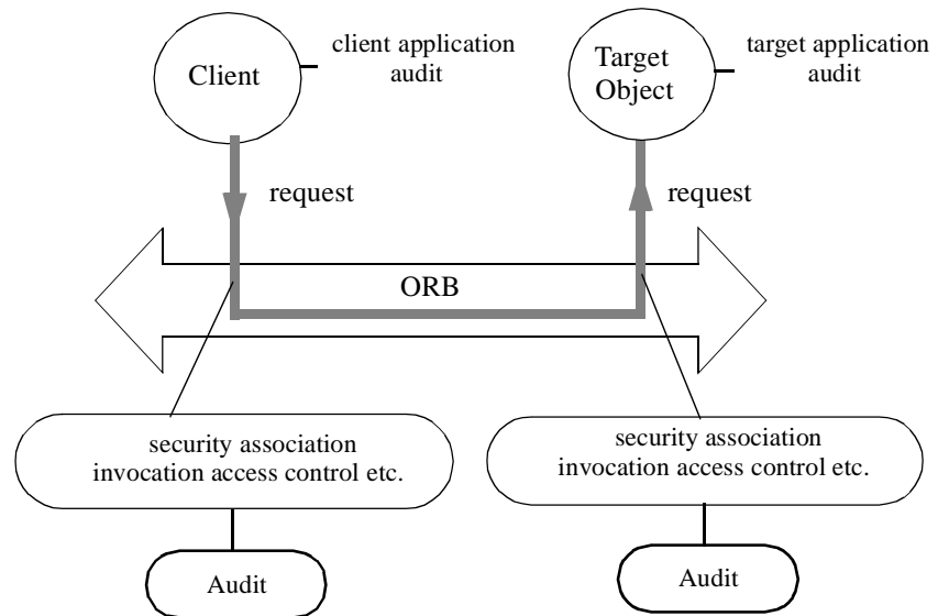
Figure 2-7 Auditing Model
