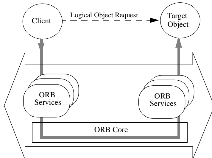
Figure 2-23 ORB Services
