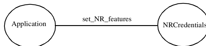
Figure 2-39 set_NR_features Operation
