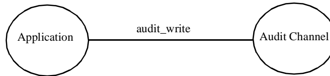
Figure 2-37 audit_write Application
