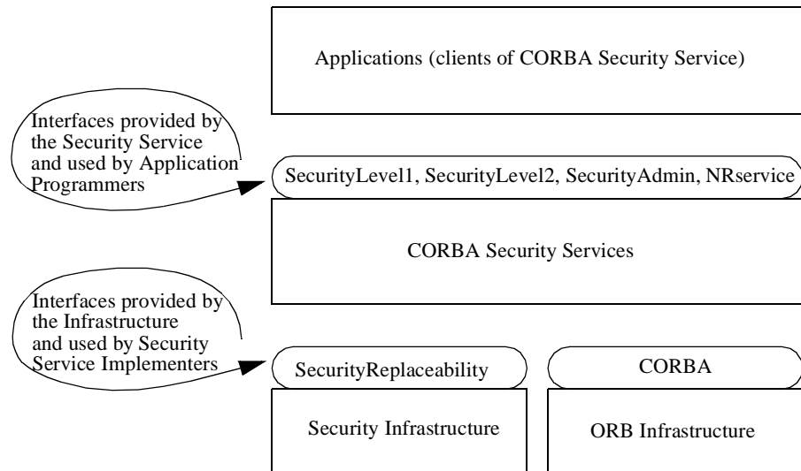
Figure 1-1 Modules and Their Relation to Layers of the Architecture
