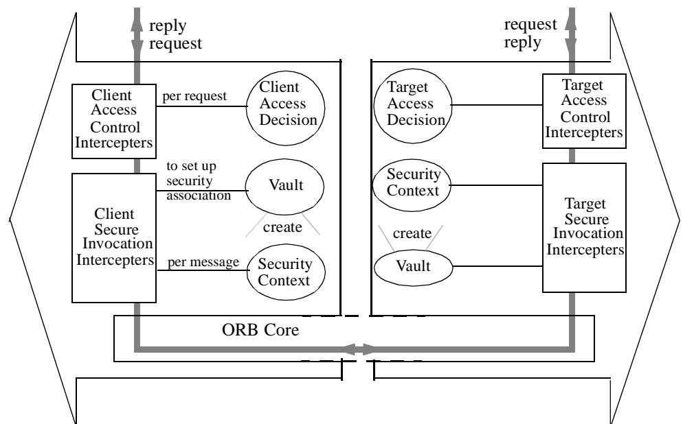
Figure 2-52 Security Functionality Implemented by Security Service Objects
