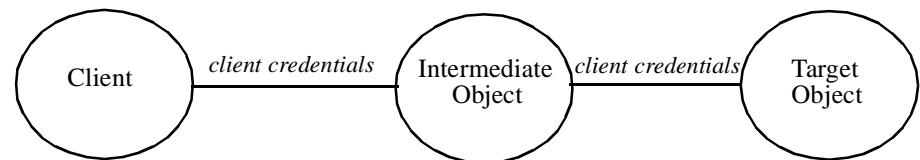
Figure 2-10 Simple Delegation
