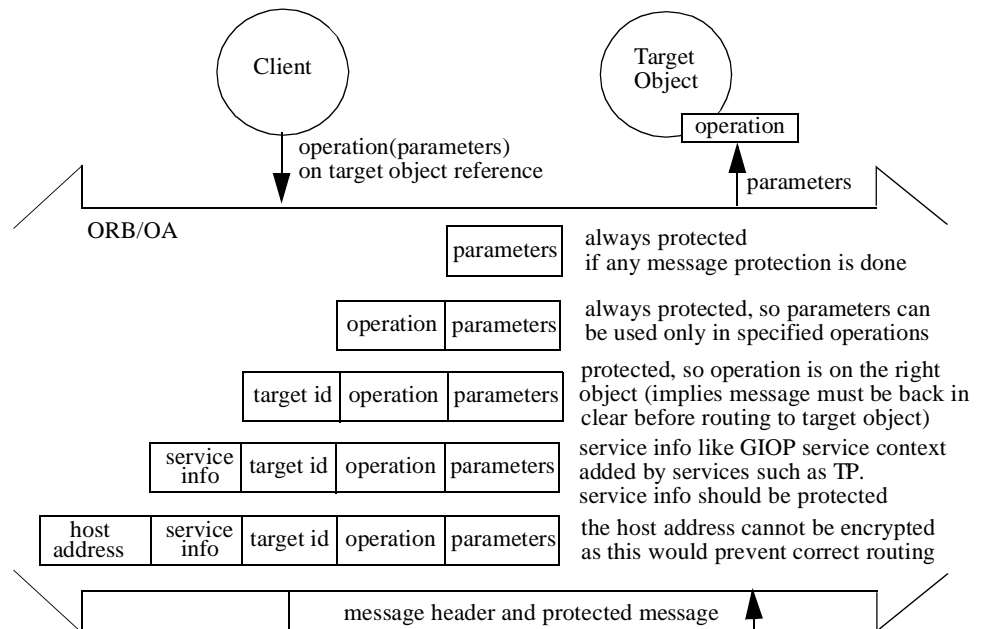
Figure 2-4 Message Protection
