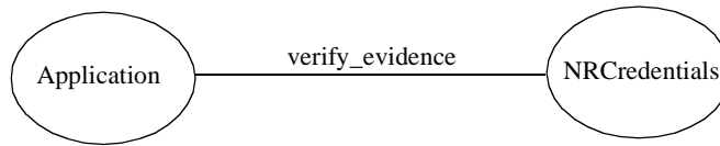
Figure 2-42 verify_evidence operation
