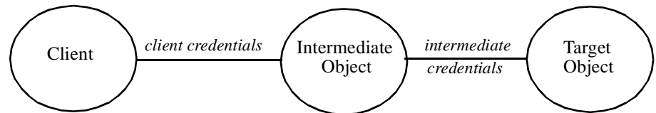
Figure 2-9 No Delegation
