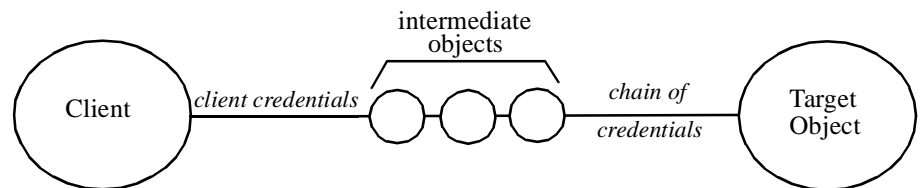
Figure 2-13 Traced Delegation
