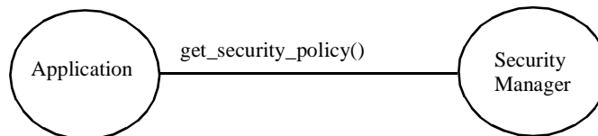
Figure 2-36 get_security_policy Application
