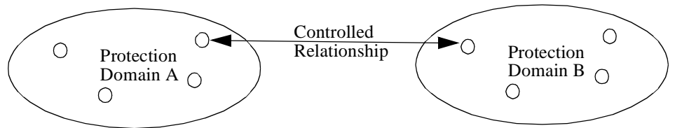
Figure 2-26 Controlled Relationship
