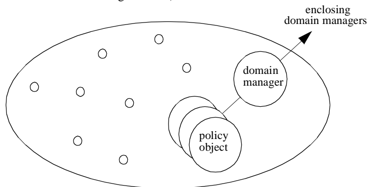
Figure 2-25 Domain Objects
