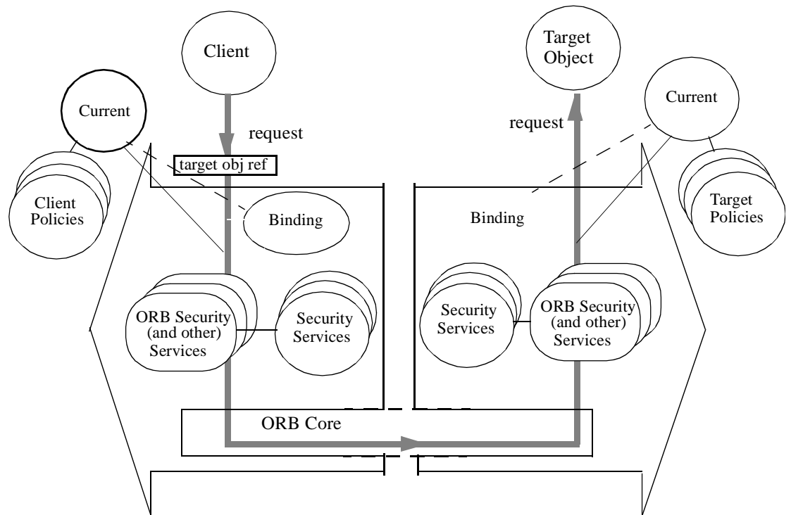
Figure 2-45 Securing Invocations
