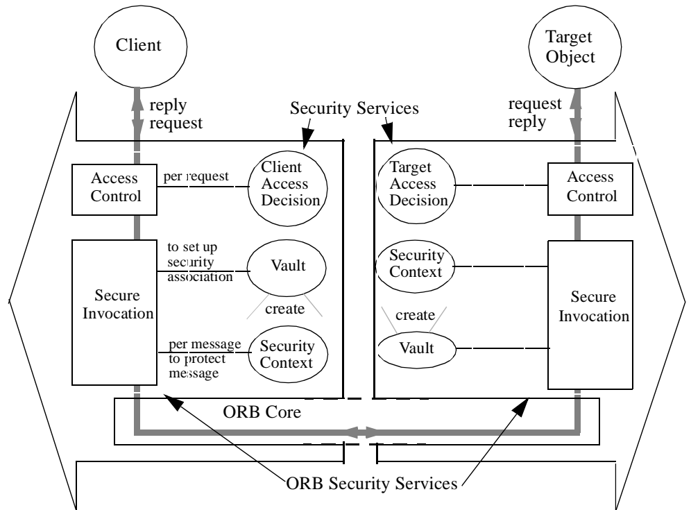
Figure 2-47 ORB Security Services
