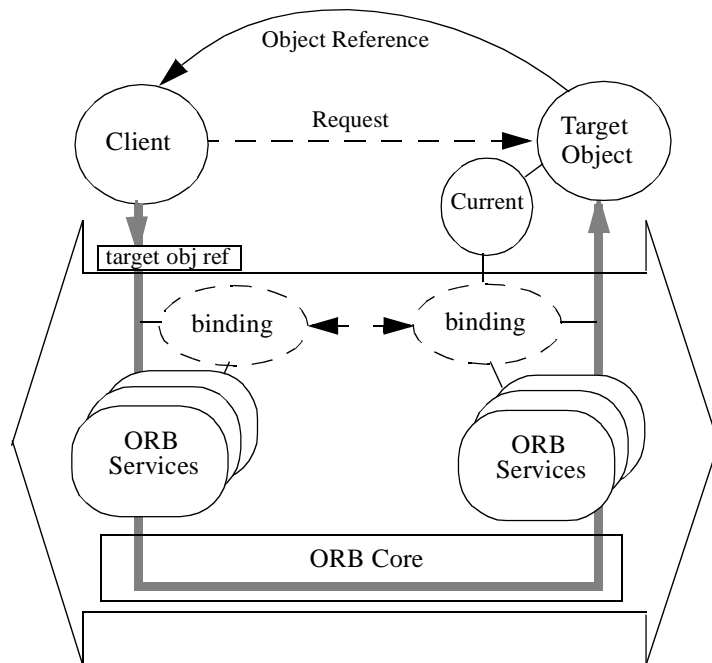
Figure 2-24 Object Reference
