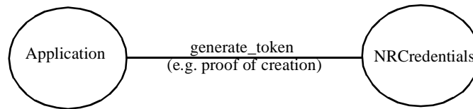
Figure 2-40 generate_token Operation
