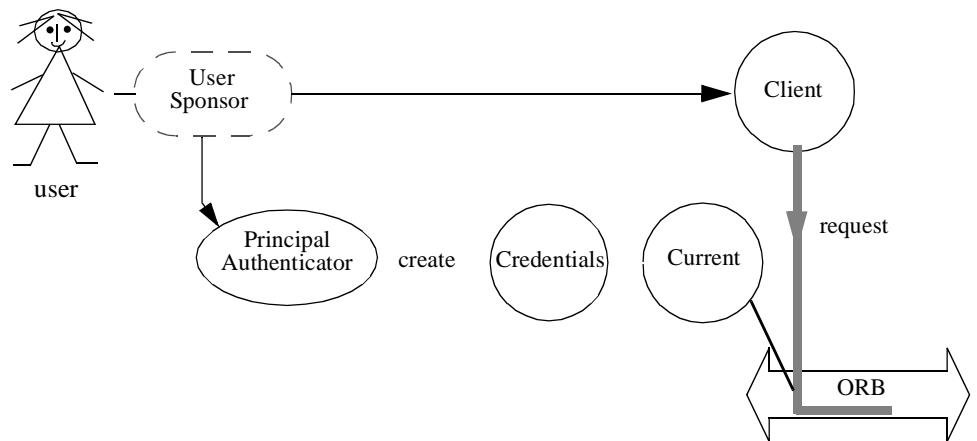
Figure 2-28 Authentication
