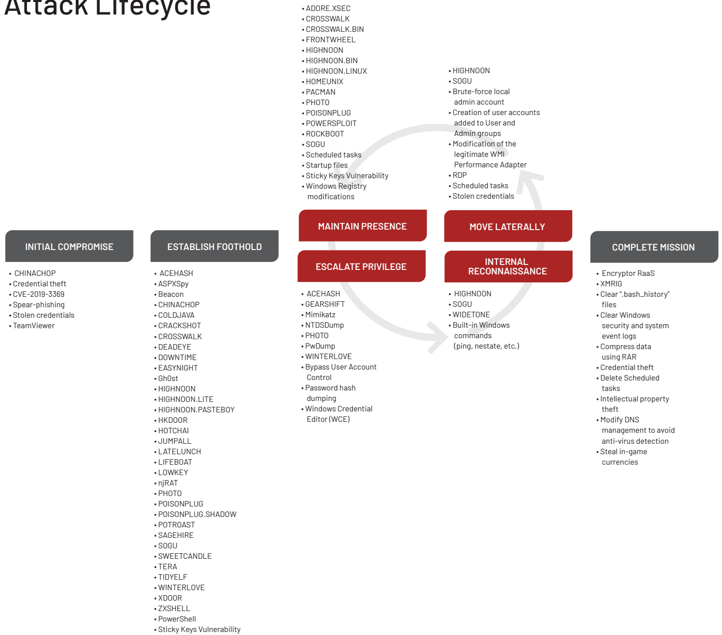
FIGURE 19. APT41 attack lifecycle.
