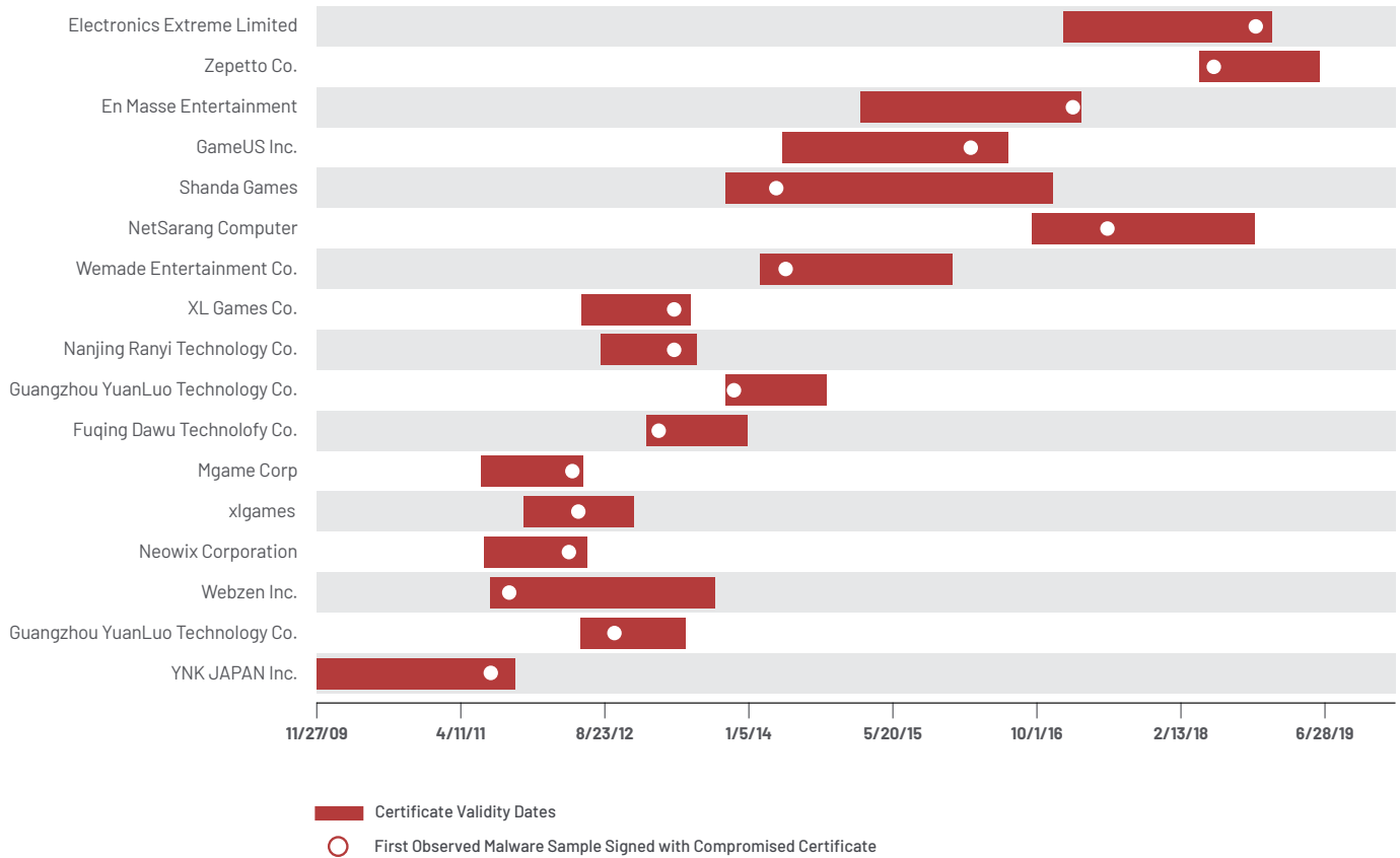
FIGURE 18. First observed malware samples signed with digital certificates (white) in relation to valid certificate dates (blue).
