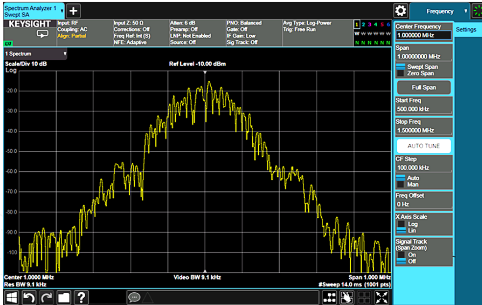
Figure 2-41. Spectrum of the GSM signal
