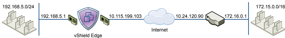
Figure 9-4. vShield Edge connecting to a remote VPN gateway
