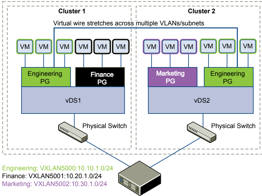
Figure 8-3. ACME Enterprise implements a VXLAN virtual wire
