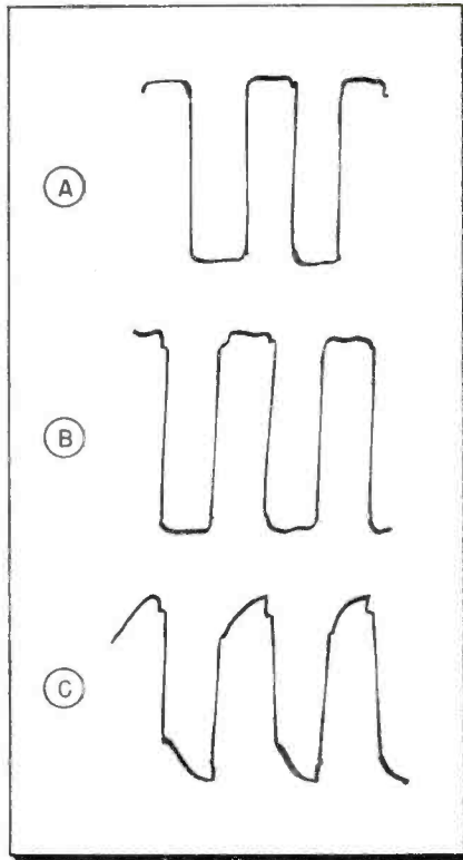
Fig. 4—The effects of attenuator adjustment; (A) the trace of a square wave fed directly to the deflection plates, (B) the trace of the same square wave when the attenuator is properly adjusted, and (C) the trace from an improperly adjusted attenuator.
