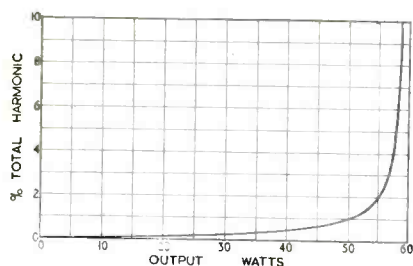
Fig. 1—Typical harmonic distortion curve.
