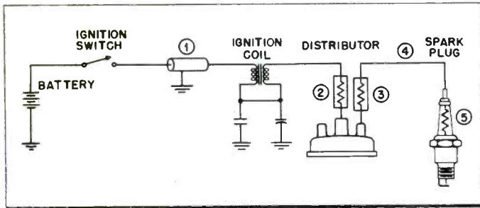
Ignition, and electrical-system noise-suppression remedies: 1. coaxial capacitor, .1 \mu\text{f} ; 2. resistor, 10,000 ohms; 3. resistor, 5,000 ohms;
