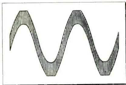
Fig. 2—High tone modulated by low tone.
