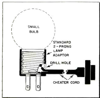
Cheater cord and line voltage indicator.
