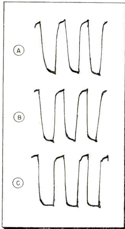
Fig. 2—Distortion of 20,000-cps square waves at various gain control settings; (A) shows the trace with near-zero gain, (B) at full gain, and (C) at the optimum position of the gain control.
