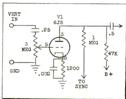
Fig. 1—Original vertical input circuit of author's scope. The simple potentiometer attenuator is frequency sensitive. See text.
