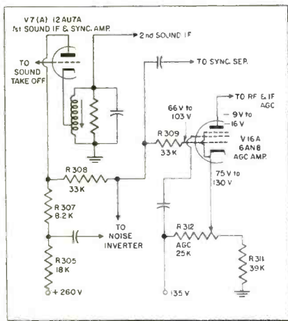
Sylvania model 1-533-1 chassis AGC circuit
