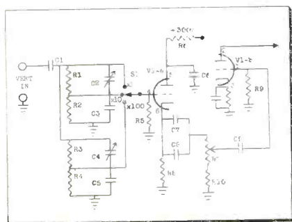
Fig. 3—Modified input circuit. V1-b replaces the original triode; rewire accordingly.
