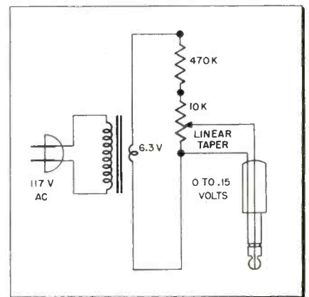
Fig. 1 Tape recorder head demagnetizer.
