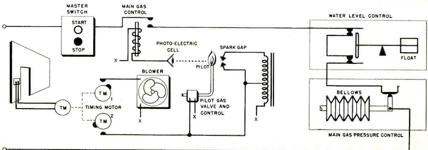
Fig. 1—The thermostat senses a demand for heat and starts the timing motor; which operates the blower and ignites the pilot light. A
