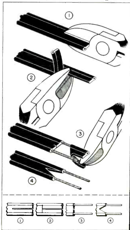
Diagonals used to strip transmission line.
