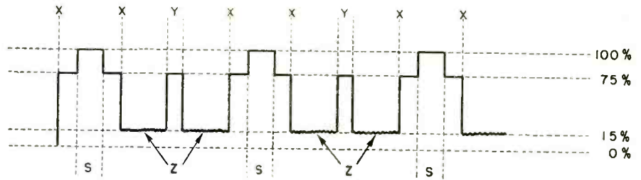
Fig. 1—Blanking bar, sync pulse and video.
