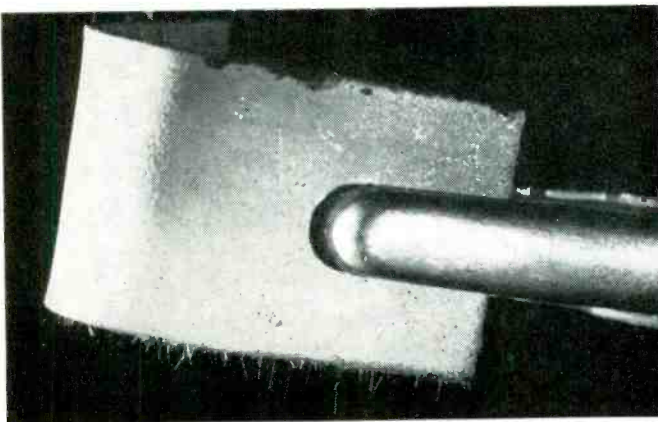
Whiskers which grew from tin-plated metal in a jar for three years at Bell Labs are type which cause telephone short circuits. Sample is 0.5" wide. Atomic radiation speeds up crystal whisker growing process.
