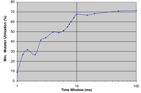
Figure 4: MMU versus time window size (SPECjbb2000)
