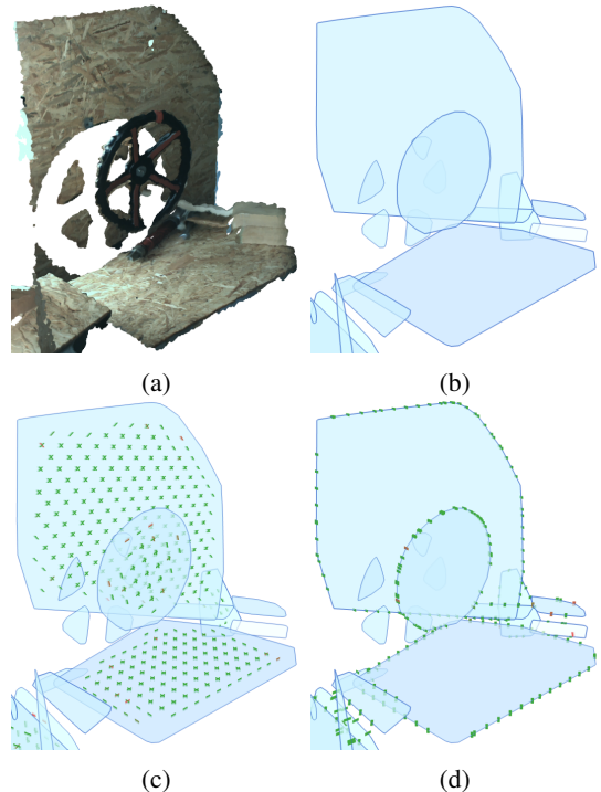
Fig. 3: The perceptual pipeline applied to an exemplary stereo vision point cloud showing an industrial valve, a large back plane and a horizontal table beneath the valve. The individual figures show (a) the raw point cloud, (b) the extracted planar primitives, (c) a visualization of the certainty function \Theta_{G-Pl} for platform grasps and (d) a visualization of the certainty function \Theta_{G-Pr} for prismatic grasps. The marker color refers to the affordance certainty at the respective end-effector pose. Green means high certainty, red low certainty and certainties of zero have been omitted.
