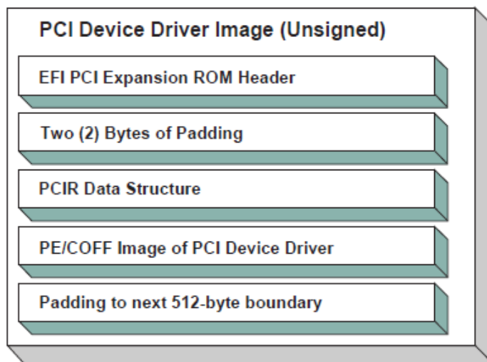
Fig. 14.15: Unsigned PCI Driver Image Layout
