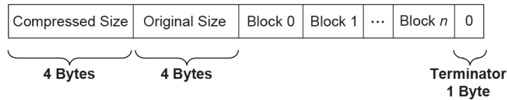
Fig. 19.2: Compressed Data Structure
