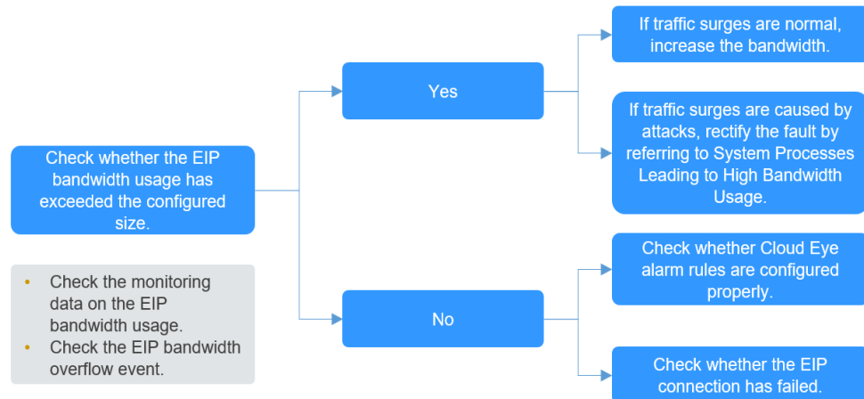
Figure 6-2 Troubleshooting procedure
