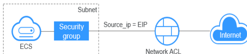
Figure 7-12 EIP network diagram
