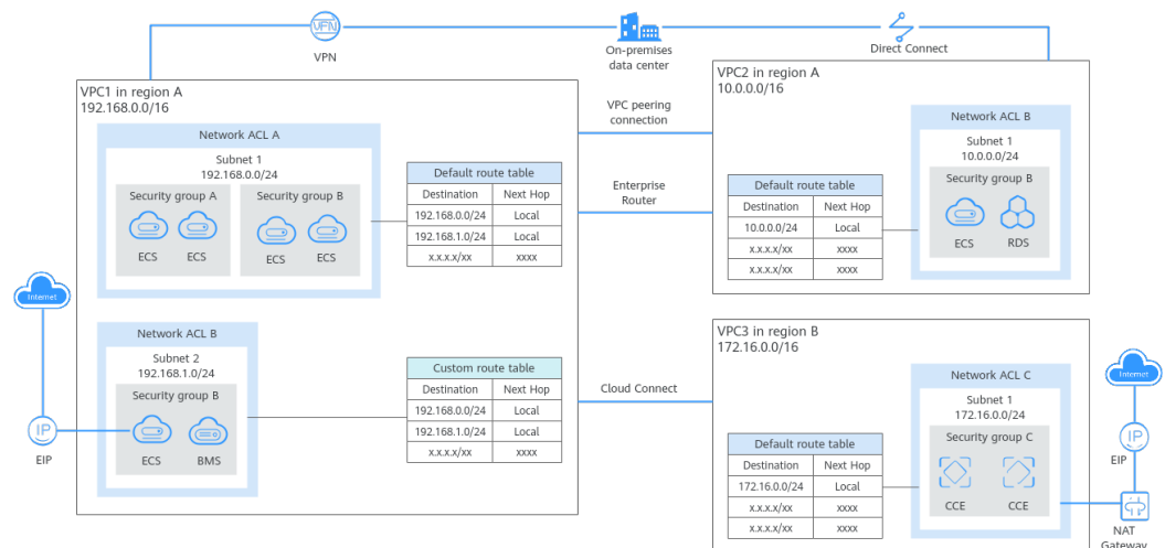
Figure 2-1 VPC architecture
