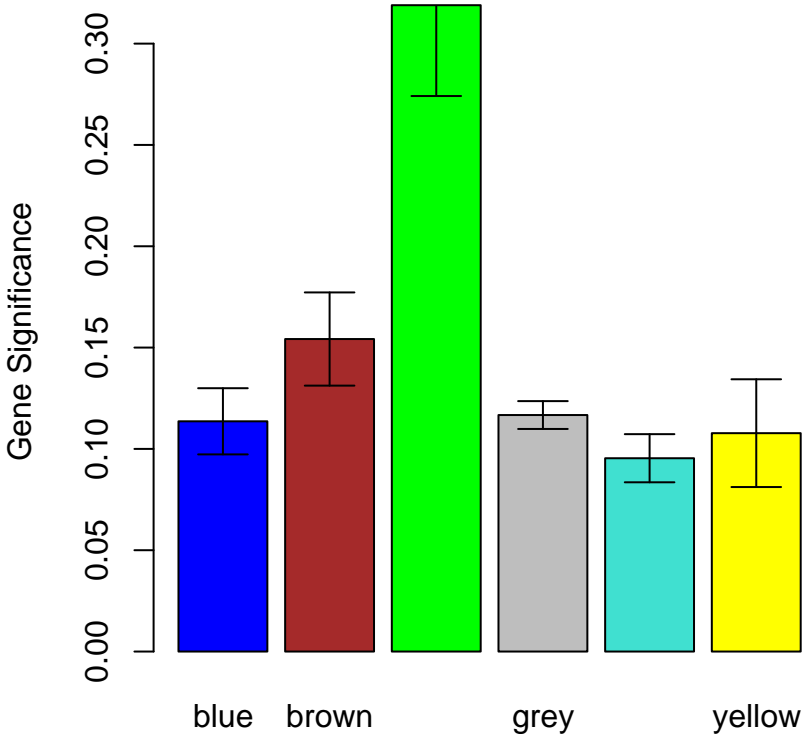
A. Gene significance across modules p-value=5.6e-13
