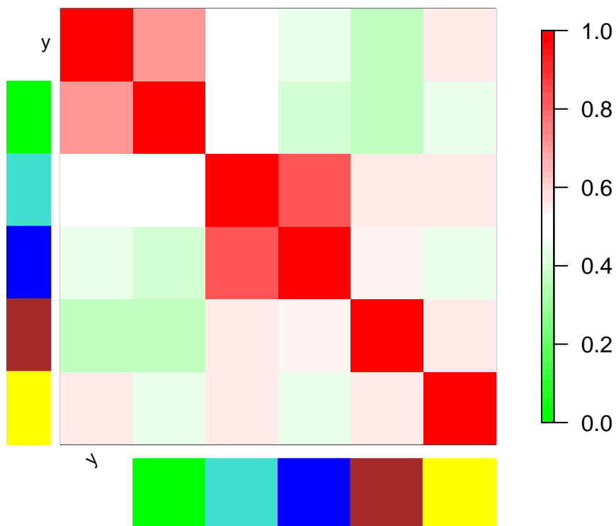
D. Eigengene network heatmap
