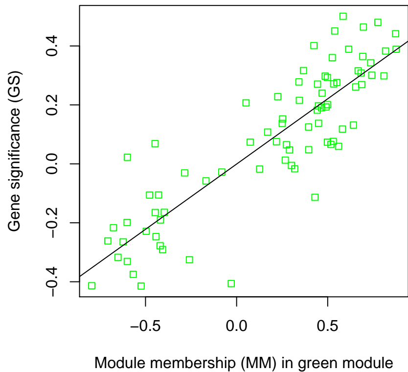
B. GS vs. MM, green module cor=0.87 p=<10 -20
