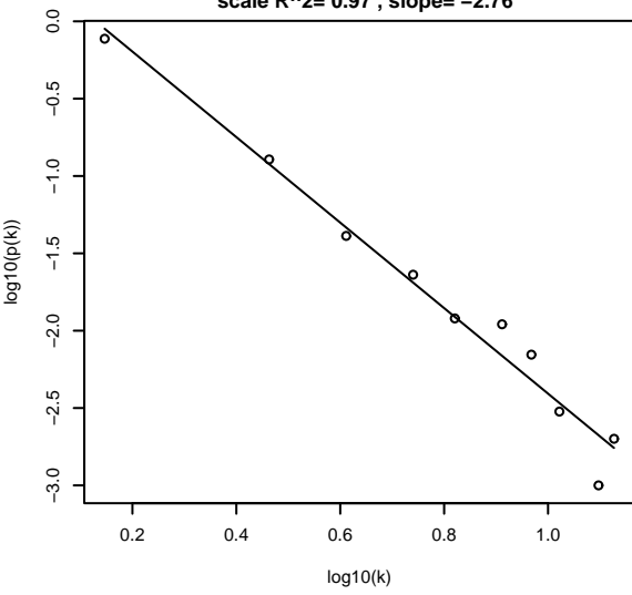
A. Check of scale free topology scale R^2= 0.97 , slope= -2.76
