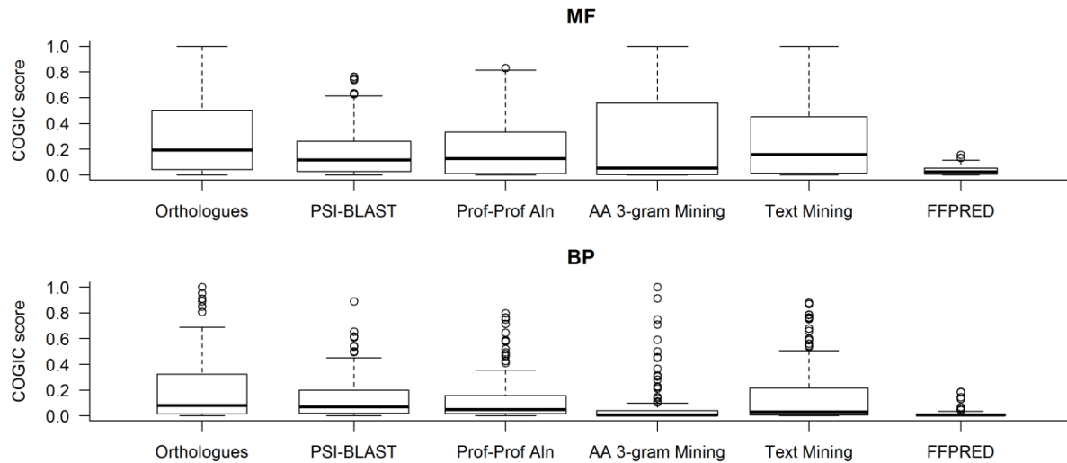
Additional figure 1: Supplementary comparisons of the COGIC score distributions. Individual predictors were contrasted on the subsets of the MF (upper panel) and BP (lower panel) benchmarks that were targeted by the Amino Acid Trigram Mining classifier. Each box spans from the first to the third quartile of the corresponding distribution; the median value is highlighted as a thick line, while putative outliers are plotted as empty circles. The width of each box is proportional to the coverage of the corresponding datasets. Groups are ordered as in Table 1 and some names shortened (“Orthologues” for Orthologous Groups, “Prof-Prof Aln” for Profile-Profile Alignment, “AA 3-gram Mining” for Amino Acid Trigram Mining and “Text Mining” for Swiss-Prot Text Mining).
