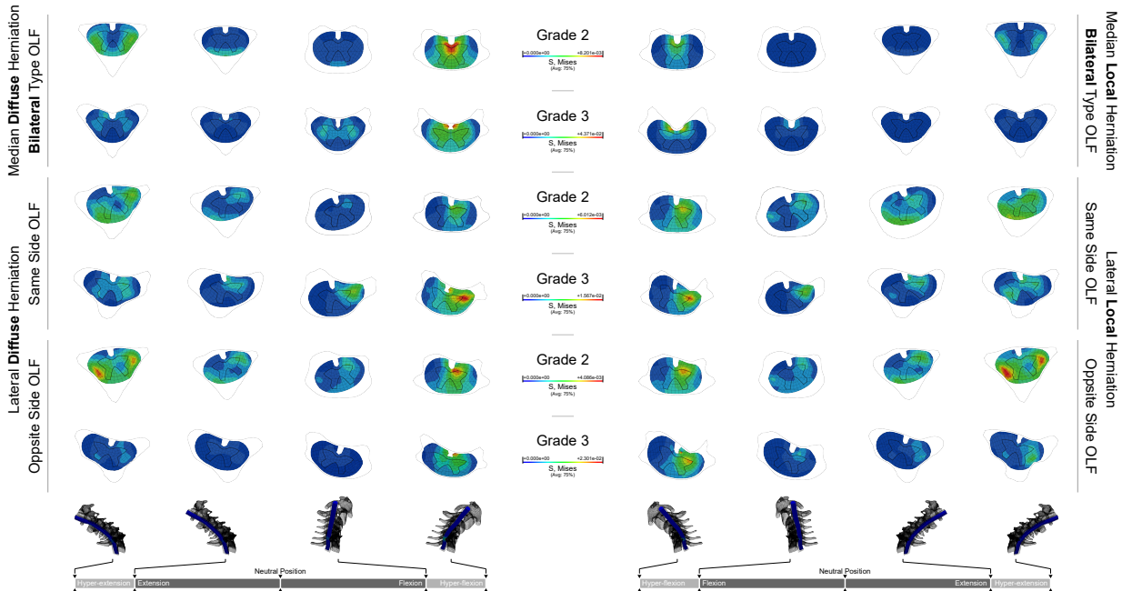
Von-Mises Stress in the Cord with both Disk Herniation and OLF (Pincer Effect)
