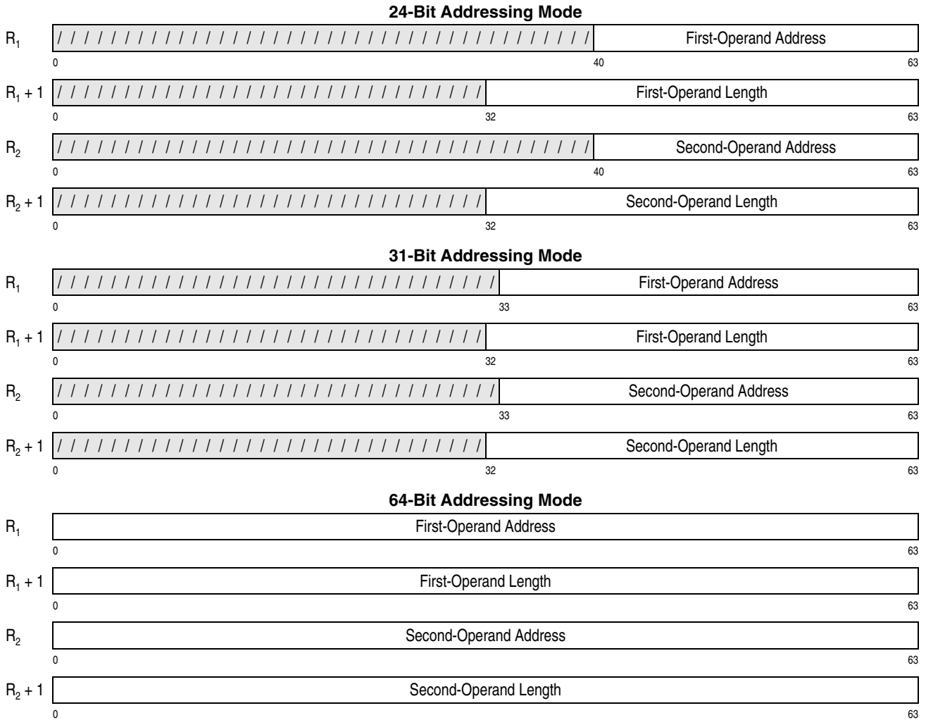
Figure 7-298. Register Contents for CONVERT UTF-8 TO UTF32
