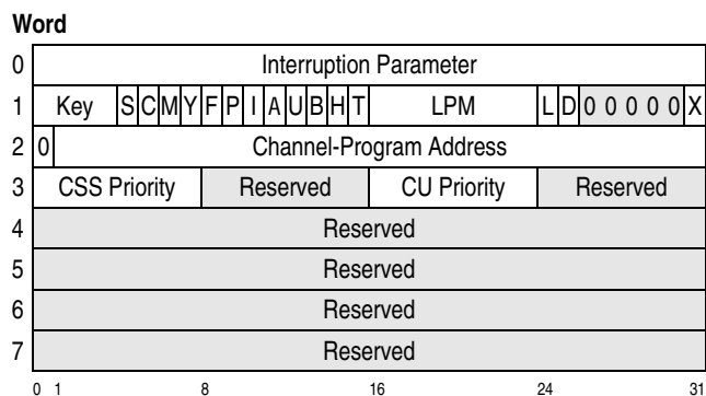
Figure 15-5. Command-Mode Operation-Request Block
