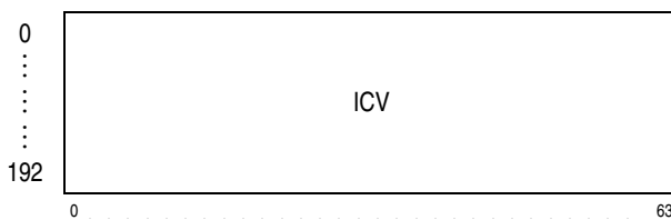
Figure 7-262. Parameter Block for KLMD-SHAKE-256
