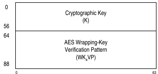
Figure 10-51. Parameter Block for PCKMO-Encrypt-ECC-Ed448-Key
