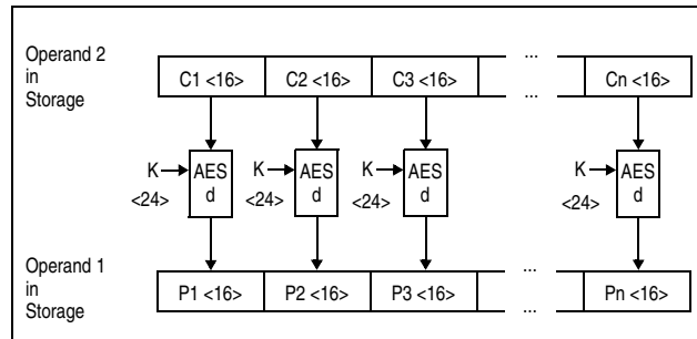
Figure 7-34. KM AES Decipher Operation Using 192-Bit Key
