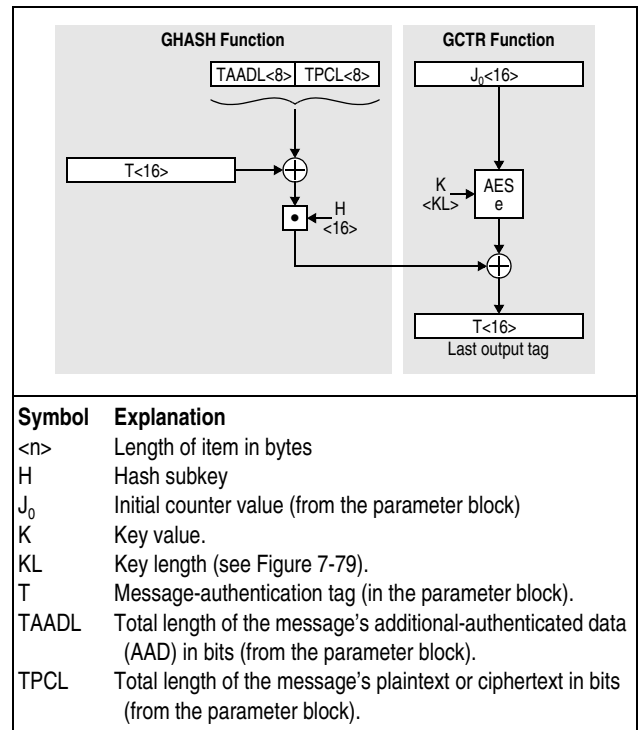
Figure 7-89. Hashing and Encrypting the Last Tag
