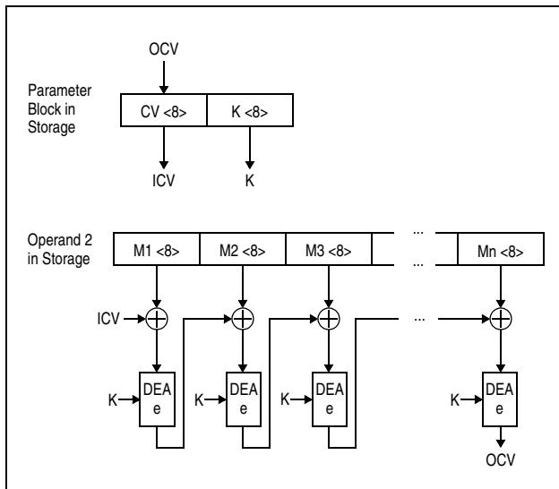
Figure 7-276. MAC Computation Using 64-bit DEA Key
