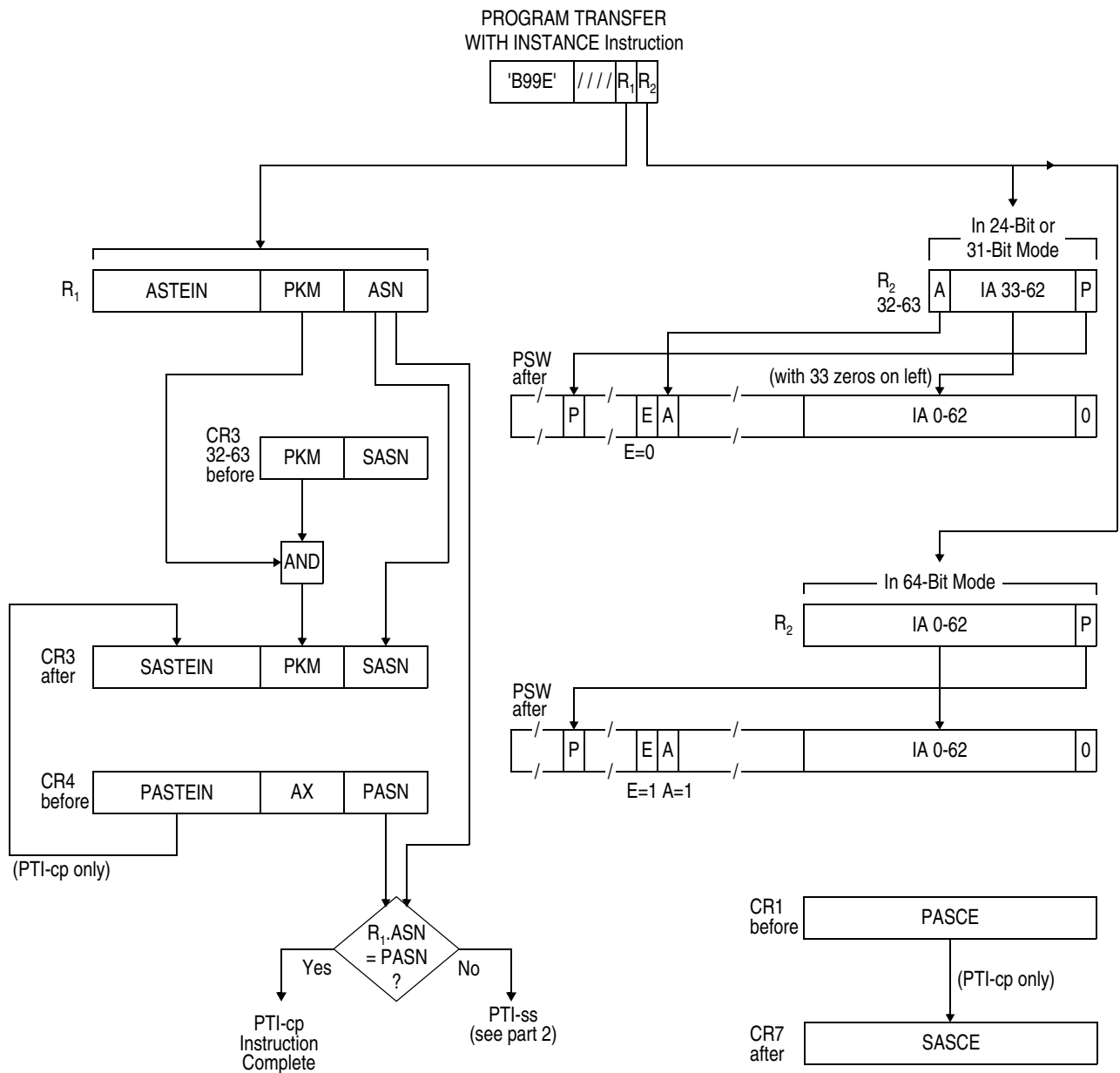
Figure 10-77. Execution of PROGRAM TRANSFER WITH INSTANCE (Part 1 of 2).
