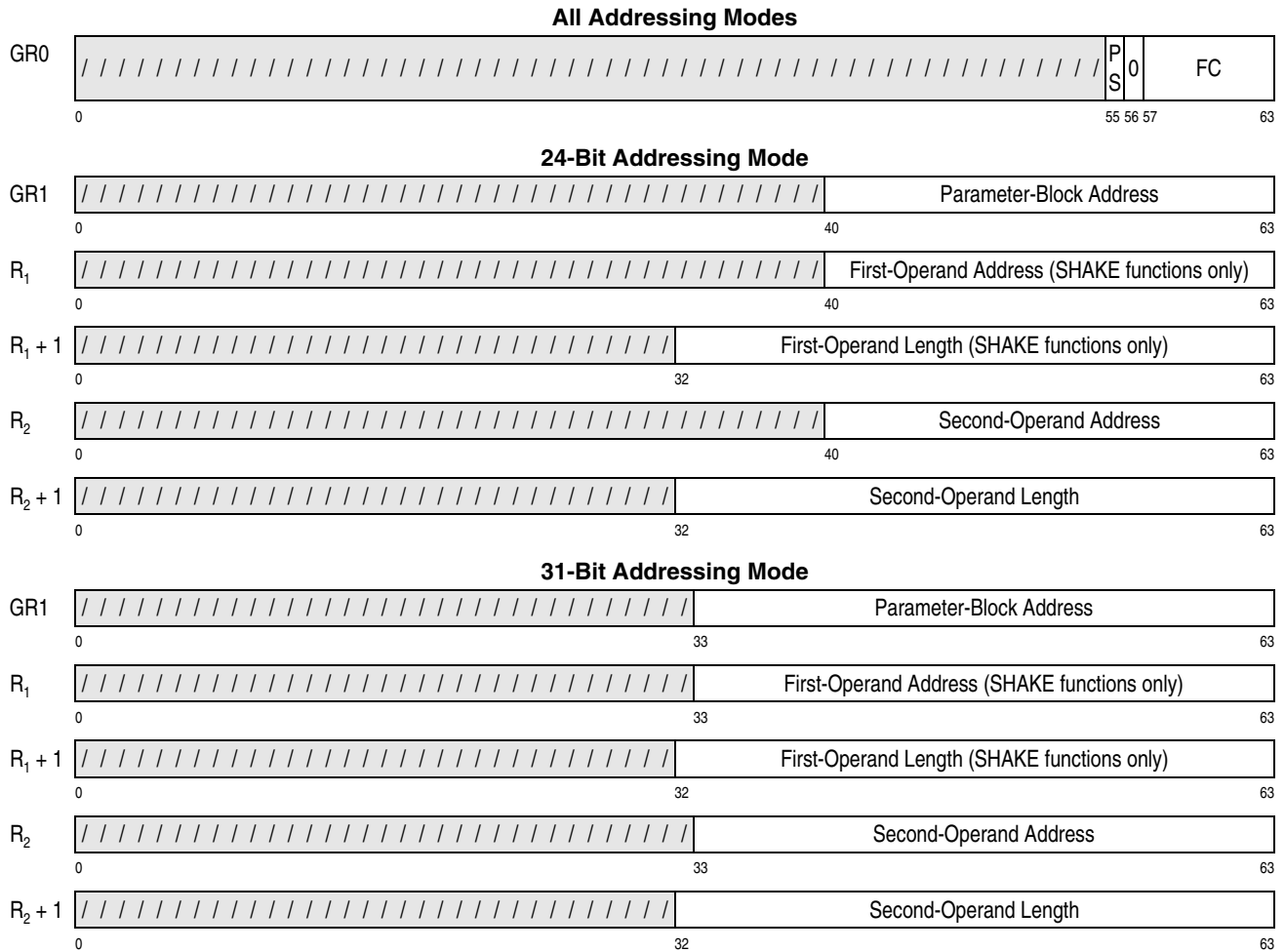
Figure 7-234. General Register Assignment for KLMD (Part 1 of 2)
