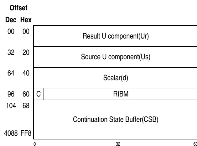
Figure 7-342. Parameter Block for PCC-Scalar-Multiply-X25519 Function
