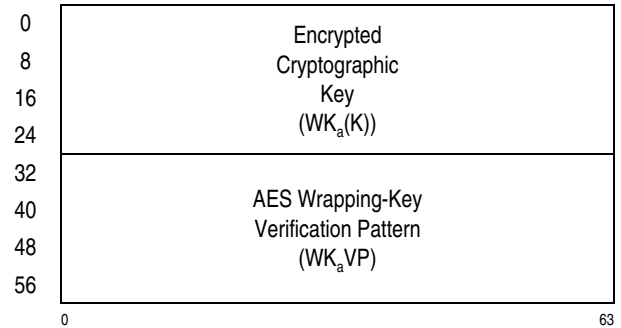
Figure 7-36. Parameter Block for KM-Encrypted-AES-256
