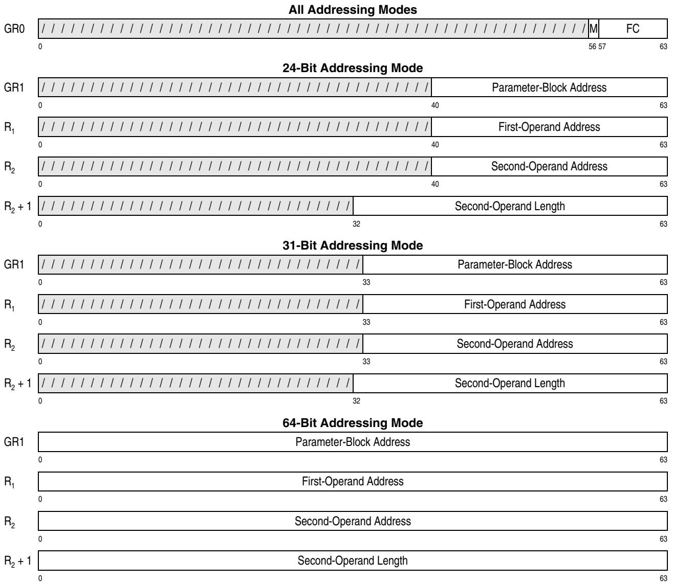
Figure 7-7. General Register Assignment for KM and KMC
