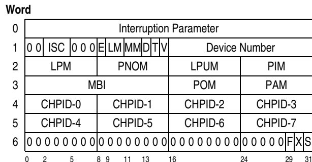
Figure 15-1. PMCW Format
