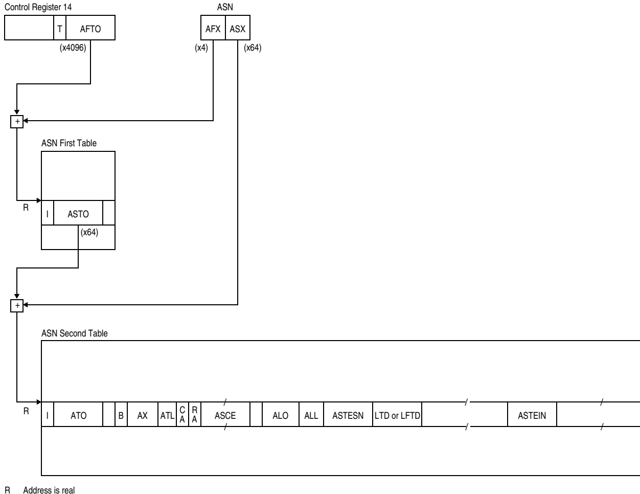
Figure 3-13. ASN Translation
