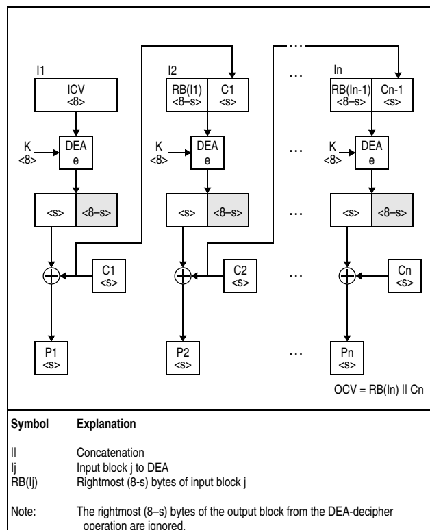
Figure 7-103. KMF-DEA Decipher Operation
