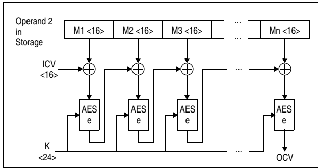
Figure 7-288. KMAC-AES-192
