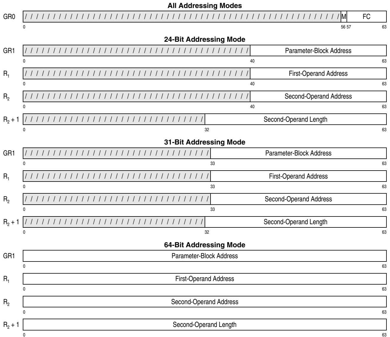
Figure 7-159. General Register Assignment for KMO
