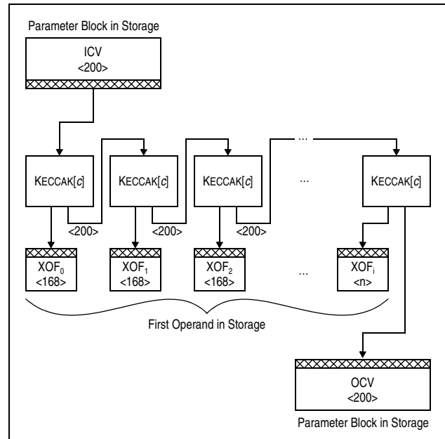
Figure 7-261. KLMD-SHAKE-128 Extended-Output-Function (XOF) Processing
