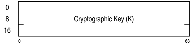
Figure 7-149. Parameter Block for KMCTR-AES-192
