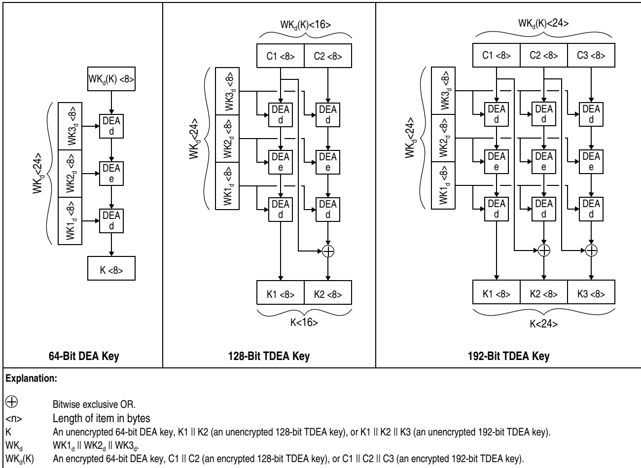
Figure 7-375. Decryption of DEA or TDEA Key Using WK d
