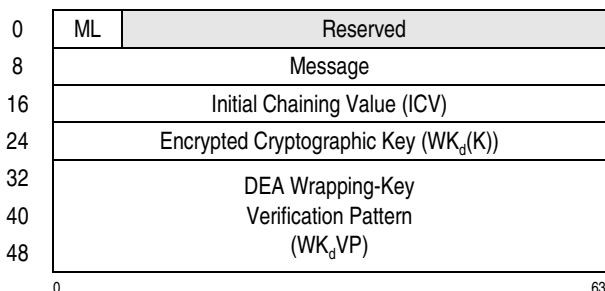
Figure 7-315. Parameter Block for PCC-Compute-Last-Block-CMAC-Using-Encrypted-DEA
