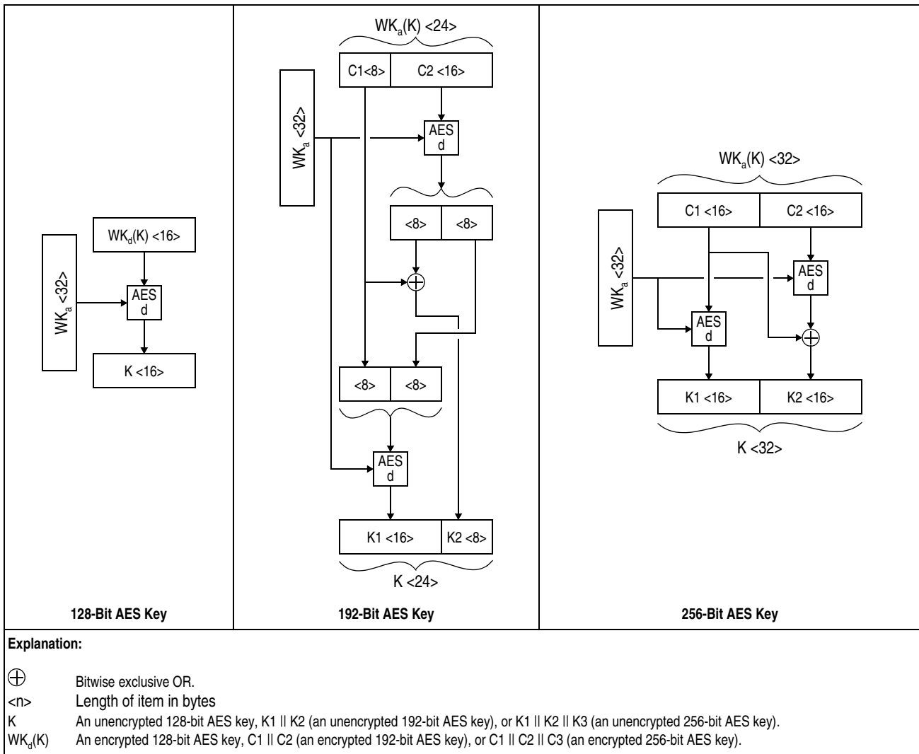
Figure 7-377. Decryption of AES Keys Using WK d
