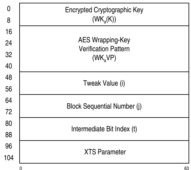
Figure 7-333. Parameter Block for PCC-Compute-XTS-Parameter-Using-Encrypted-AES-128
