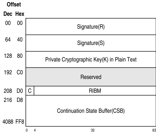
Figure 26-17. Parameter Block for KDSA-EdDSA-Sign-Ed448 Function
