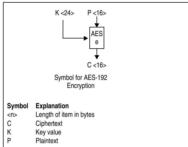
Figure 7-130. Symbols for AES-192 Encryption
