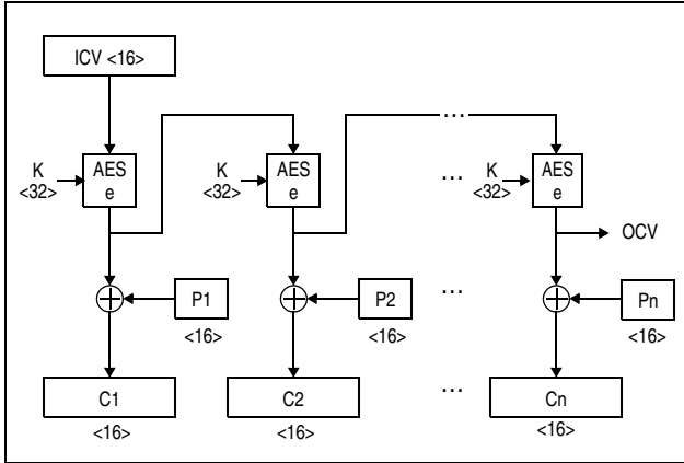
Figure 7-188. KMO-AES-256 Encipher Operation
