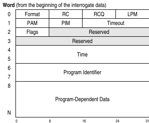
Figure 15-19. Interrogate Data
