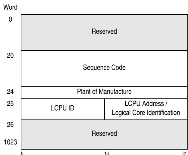
Figure 10-88. Format of the SYSIB 2.2.1
