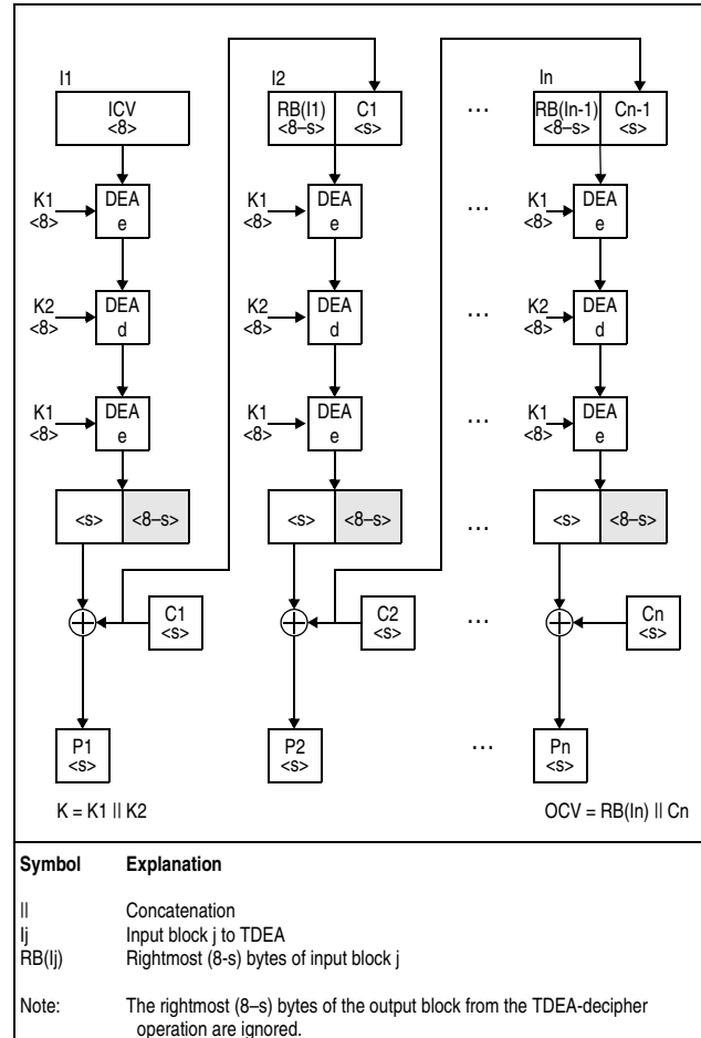
Figure 7-107. KMF-TDEA-128 Decipher Operation
