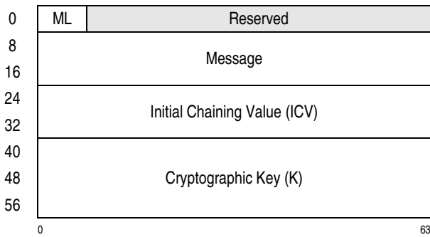
Figure 7-326. Parameter Block for PCC-Compute-Last-Block-CMAC-Using-AES-192
