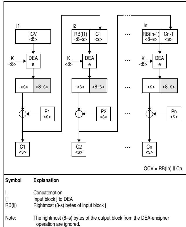
Figure 7-102. KMF-DEA Encipher Operation
