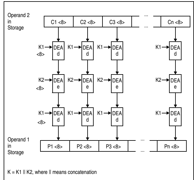
Figure 7-22. KM TDEA Decipher Operation Using 128-Bit Key
