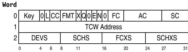
Figure 16-8. Transport-Mode SCSW Format
