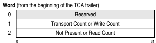
Figure 15-12. Transport-Command-Area Trailer (TCAT)
