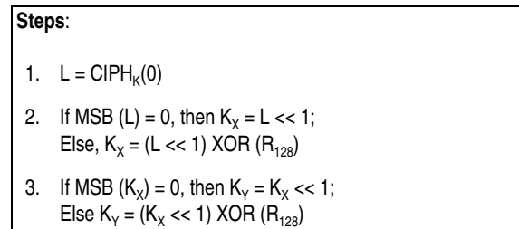
Figure 7-328. Subkey Generation Algorithm
