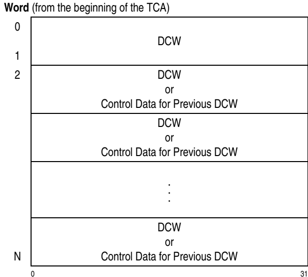
Figure 15-10. Transport-Command Area (TCA)
