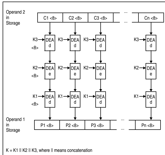
Figure 7-26. KM TDEA Decipher Operation Using 192-Bit Key
