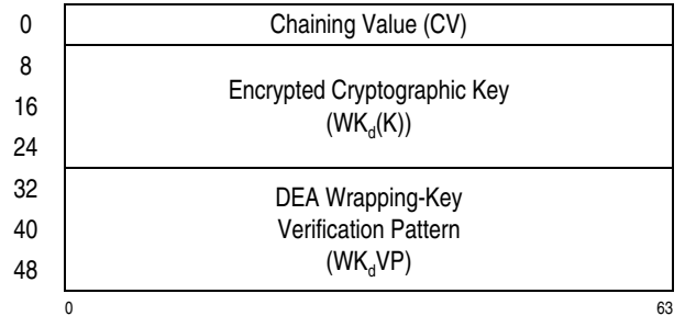
Figure 7-57. Parameter Block for KMC-Encrypted-TDEA-192
