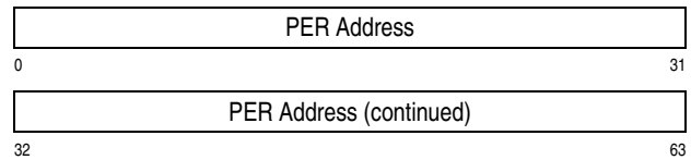
Figure 4-8. Locations 152-159 in the z/Architecture Architectural Mode
