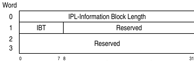
Figure 17-6. IPL-Information Block Header
