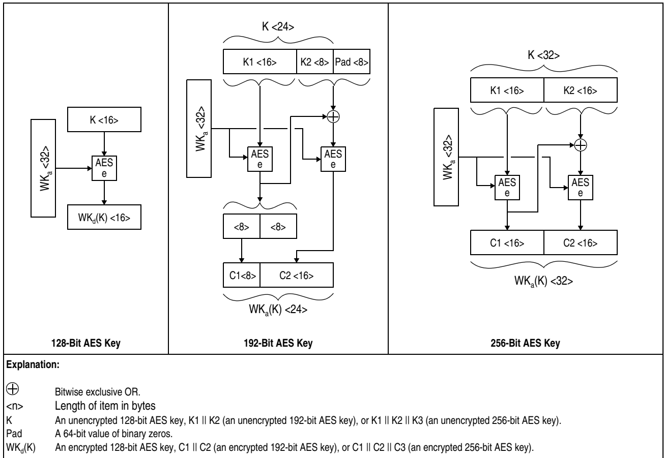
Figure 7-376. Encryption of AES Keys Using WK_a
