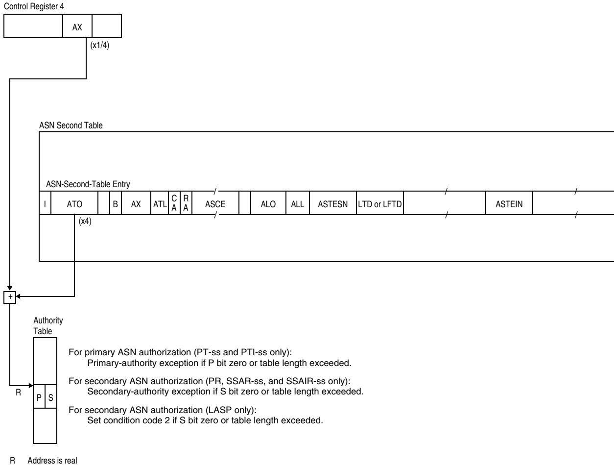
Figure 3-14. ASN Authorization
