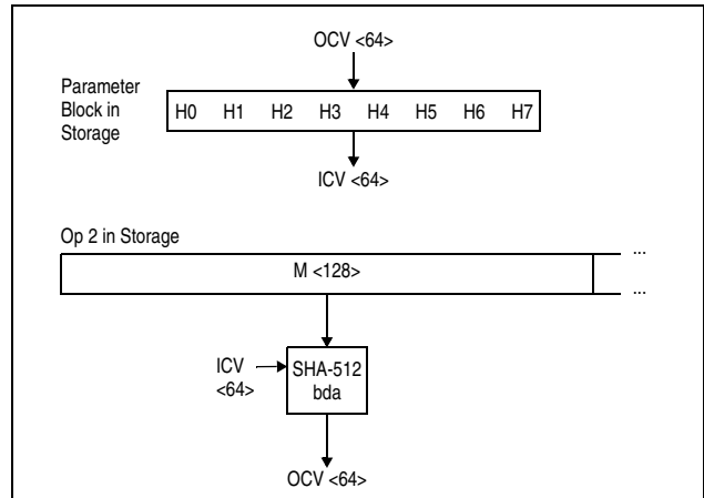
Figure 7-247. KLMD-SHA-512 Full Block (L ≥ 128)
