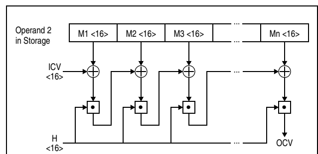
Figure 7-231. KIMD-GHASH
