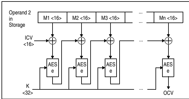
Figure 7-291. KMAC-AES-256
