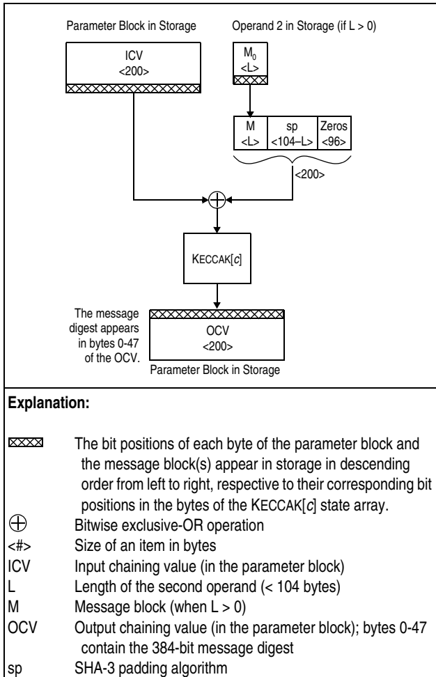
Figure 7-256. KLMD-SHA3-384 Processing (L < 104)
