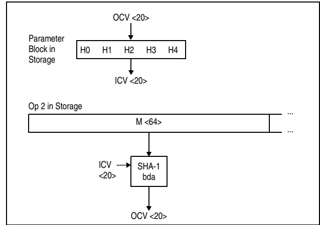
Figure 7-237. KLMD-SHA-1 Full Block ( L \geq 64 )
