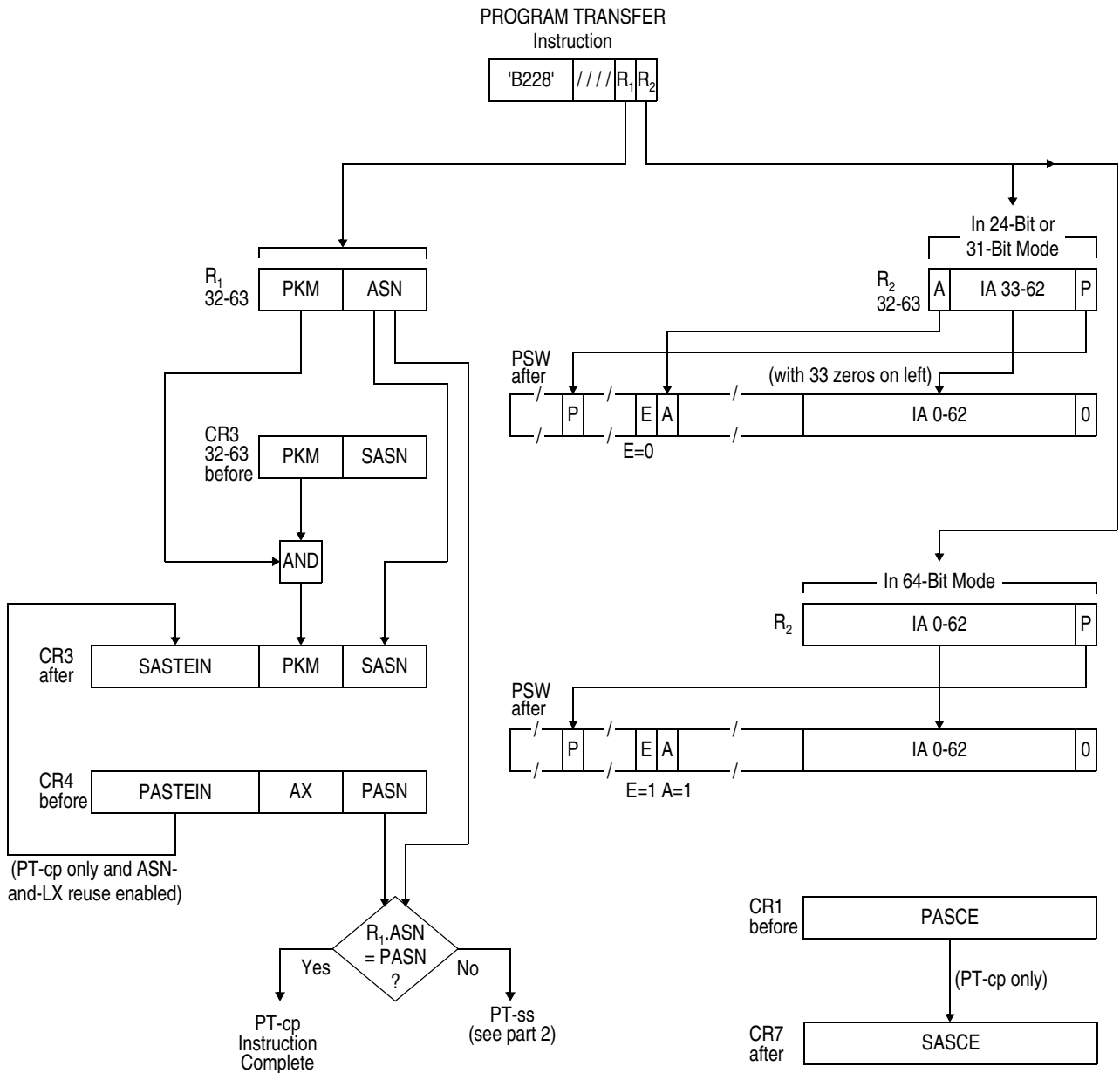
Figure 10-76. Execution of PROGRAM TRANSFER (Part 1 of 2).
