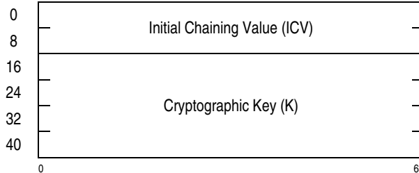
Figure 7-289. Parameter Block for KMAC-AES-256
