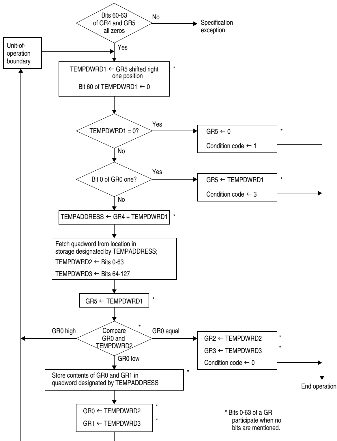
Figure 7-371. Execution of UPDATE TREE in the 64-Bit Addressing Mode
