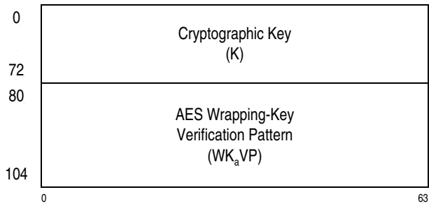
Figure 10-49. Parameter Block for PCKMO-Encrypt-ECC-P521-Key
