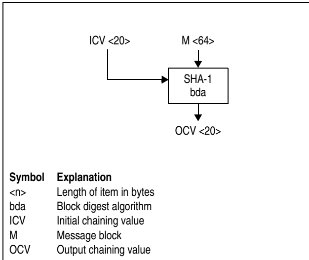
Figure 7-209. Symbol for SHA-1 Block Digest Algorithm
