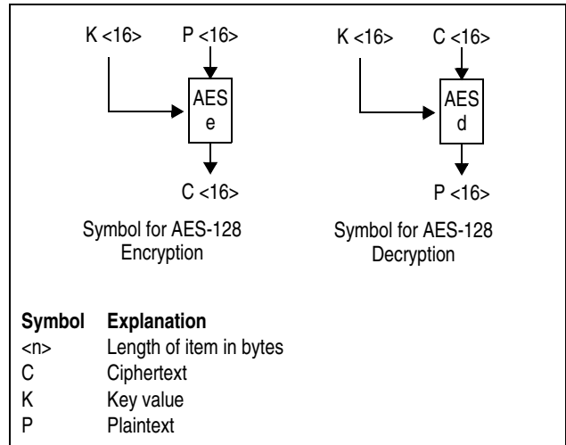
Figure 7-11. Symbols for AES-128 Encryption and Decryption
