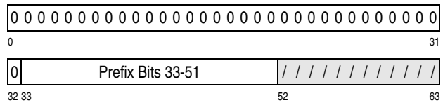
Figure 3-11. ESA/390-Compatibility Mode Prefix Register
