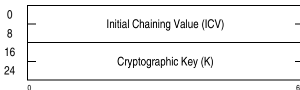
Figure 7-283. Parameter Block for KMAC-AES-128
