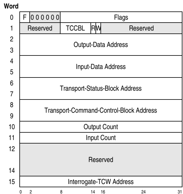
Figure 15-7. Transport-Control Word (TCW)
