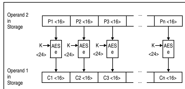
Figure 7-33. KM AES Encipher Operation Using 192-Bit Key
