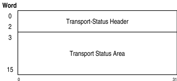
Figure 15-20. Transport-Status Block
