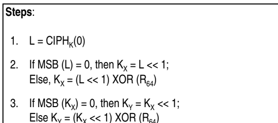
Figure 7-322. Subkey Generation Algorithm
