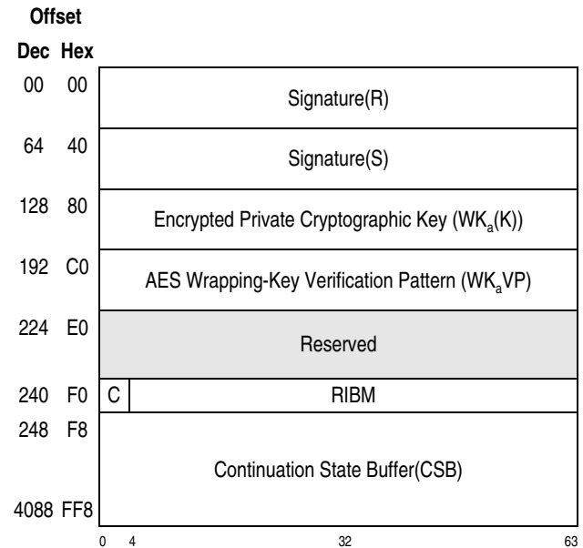
Figure 26-19. Parameter Block for KDSA-EdDSA-Sign-Ed448 Function
