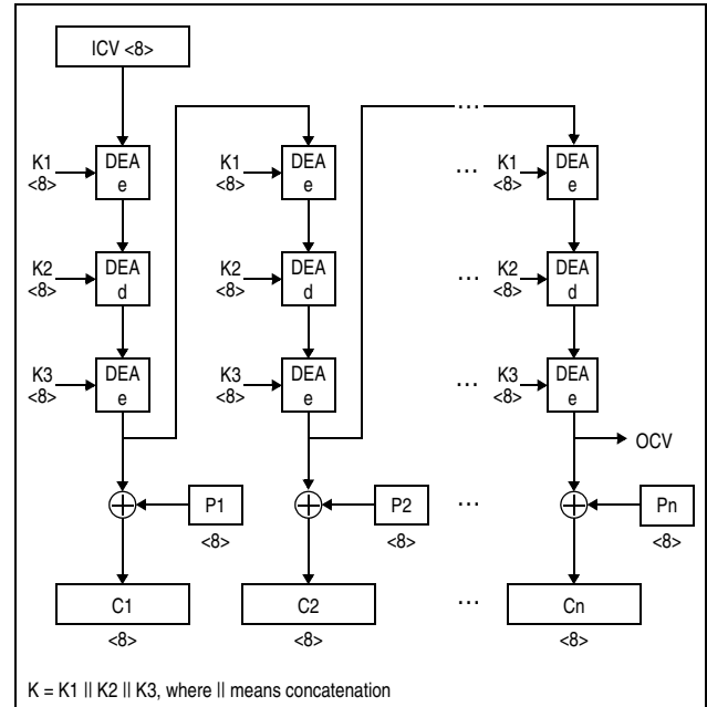
Figure 7-176. KMO-TDEA-192 Encipher Operation
