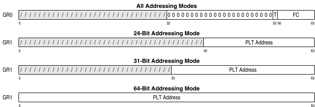
Figure 7-346. General Register Assignment for PLO
