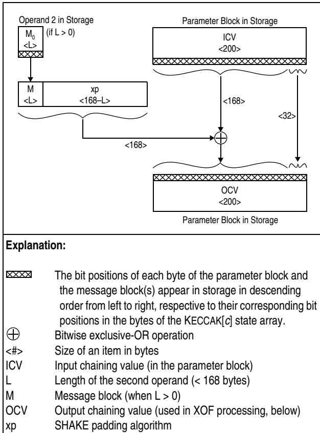
Figure 7-260. KLMD-SHAKE-128 Padding (L < 168)
