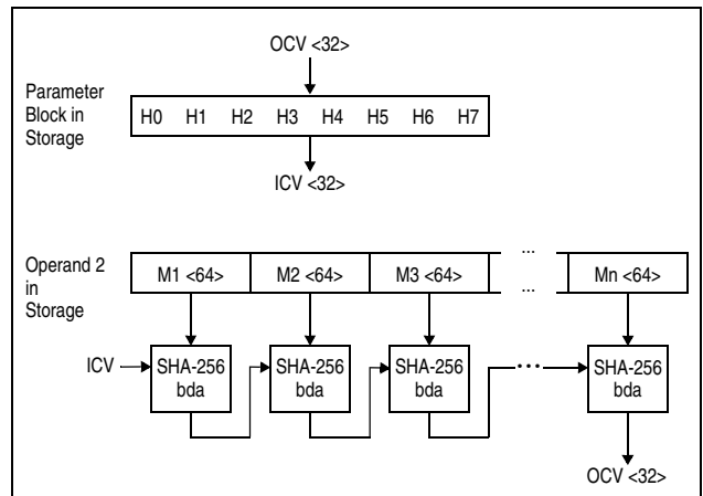
Figure 7-217. KIMD-SHA-256
