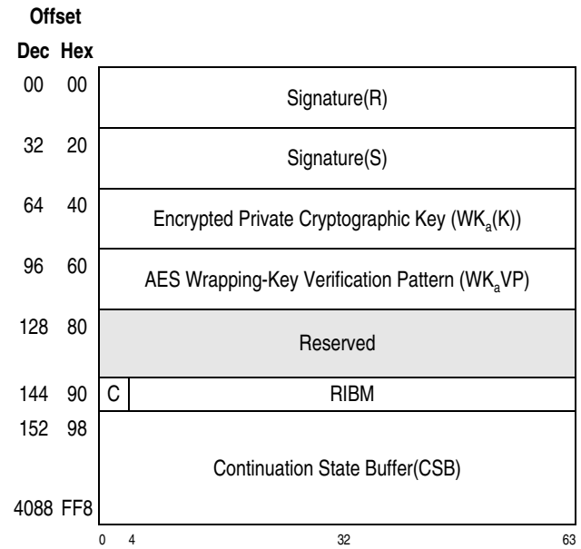
Figure 26-18. Parameter Block for KDSA-Encrypted-EdDSA-Sign-Ed25519 Function
