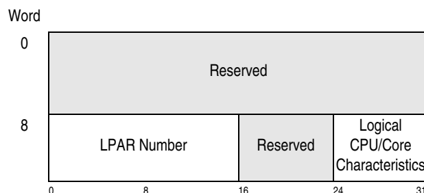
Figure 10-89. Format of the SYSIB 2.2.2 (Part 1 of 2)
