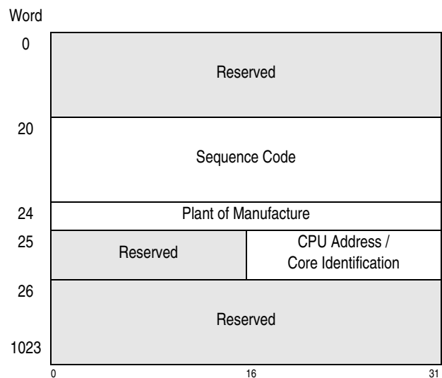
Figure 10-86. Format of the SYSIB 1.2.1
