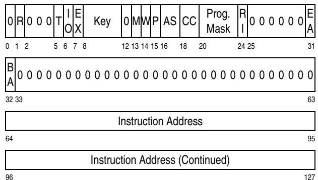
Figure 4-2. PSW Format
