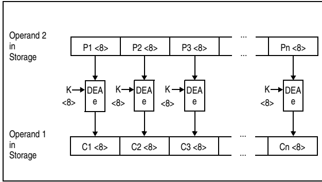
Figure 7-17. KM-DEA Encipher Operation Using 64-Bit Key
