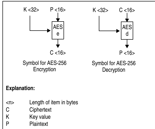
Figure 7-373. Symbols for AES-256 Encryption and Decryption
