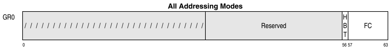
Figure 26-24. General Register Assignment for DFLTCC (Part 1 of 2)
