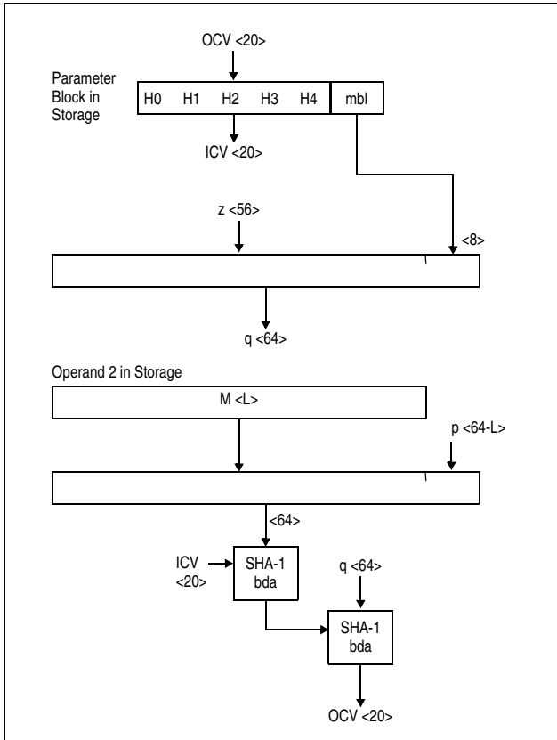
Figure 7-240. KLMD-SHA-1 Partial-Block Case 2 ( 56 \leq L \leq 63 )
