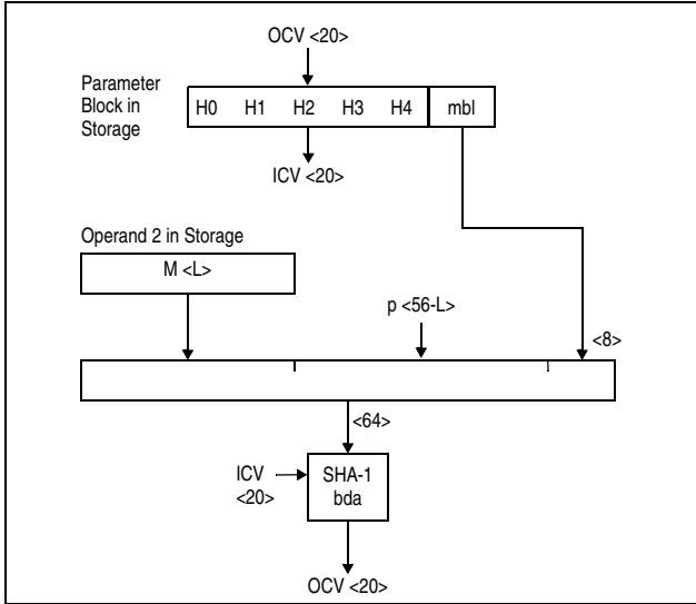
Figure 7-239. KLMD-SHA-1 Partial-Block Case 1 ( 1 \leq L \leq 55 )
