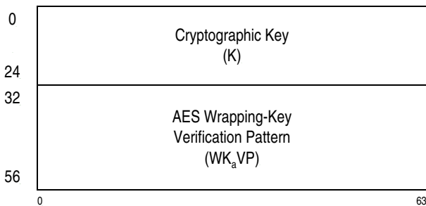
Figure 10-47. Parameter Block for PCKMO-Encrypt-ECC-P256-Key
