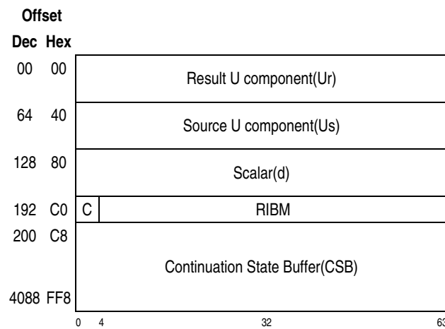
Figure 7-343. Parameter Block for PCC-Scalar-Multiply-X448 Function
