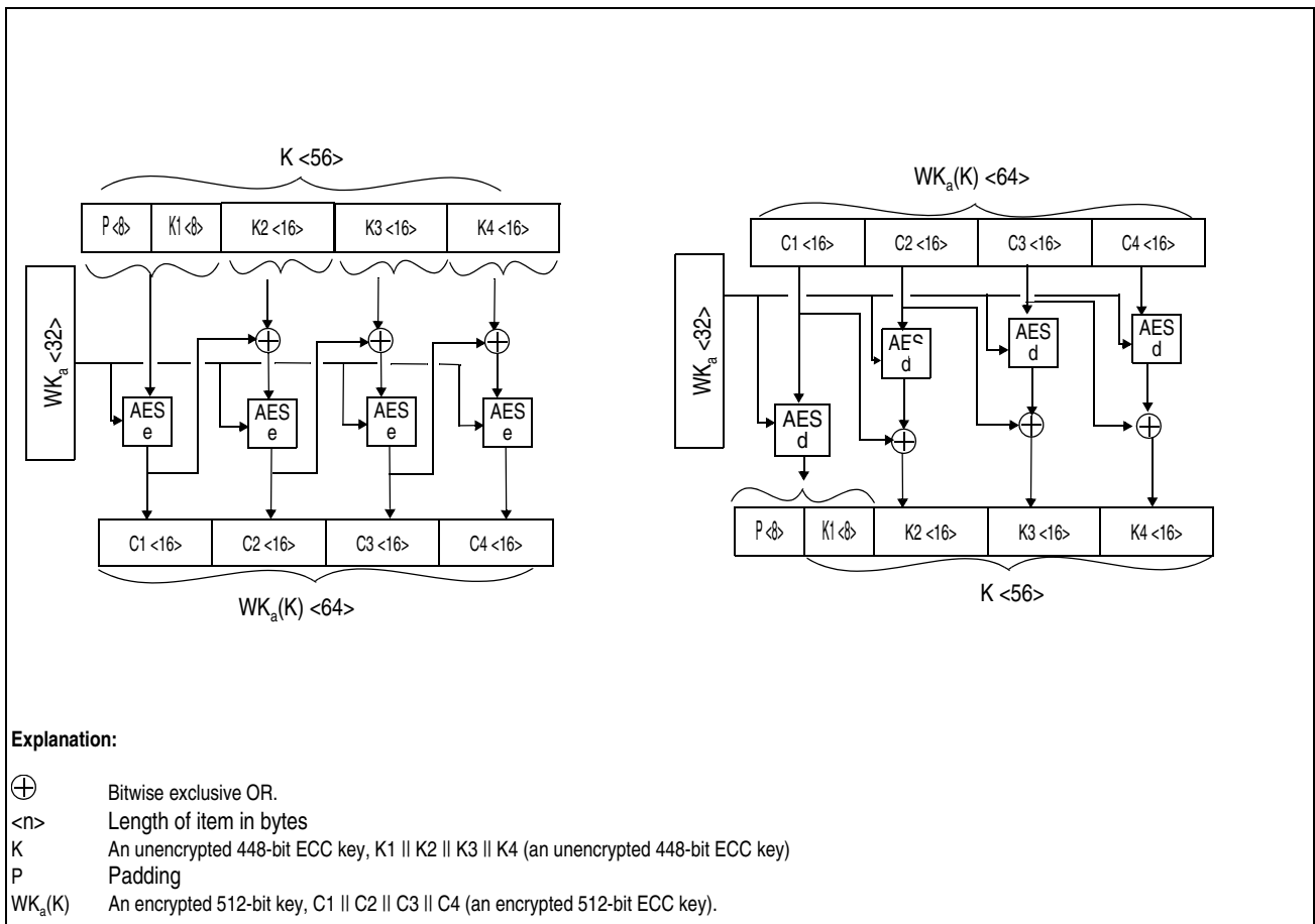
Figure 7-380. Encryption and Decryption of ECC Keys for Ed448 Using WK_a
