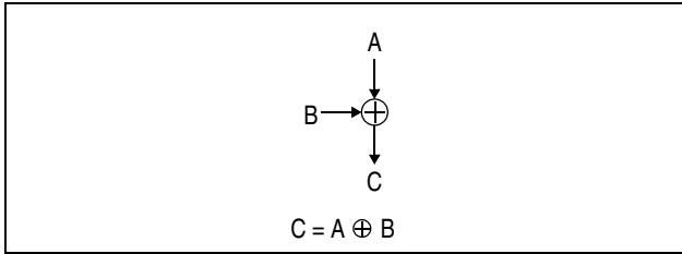
Figure 7-8. Symbol For Bit-Wise Exclusive OR
