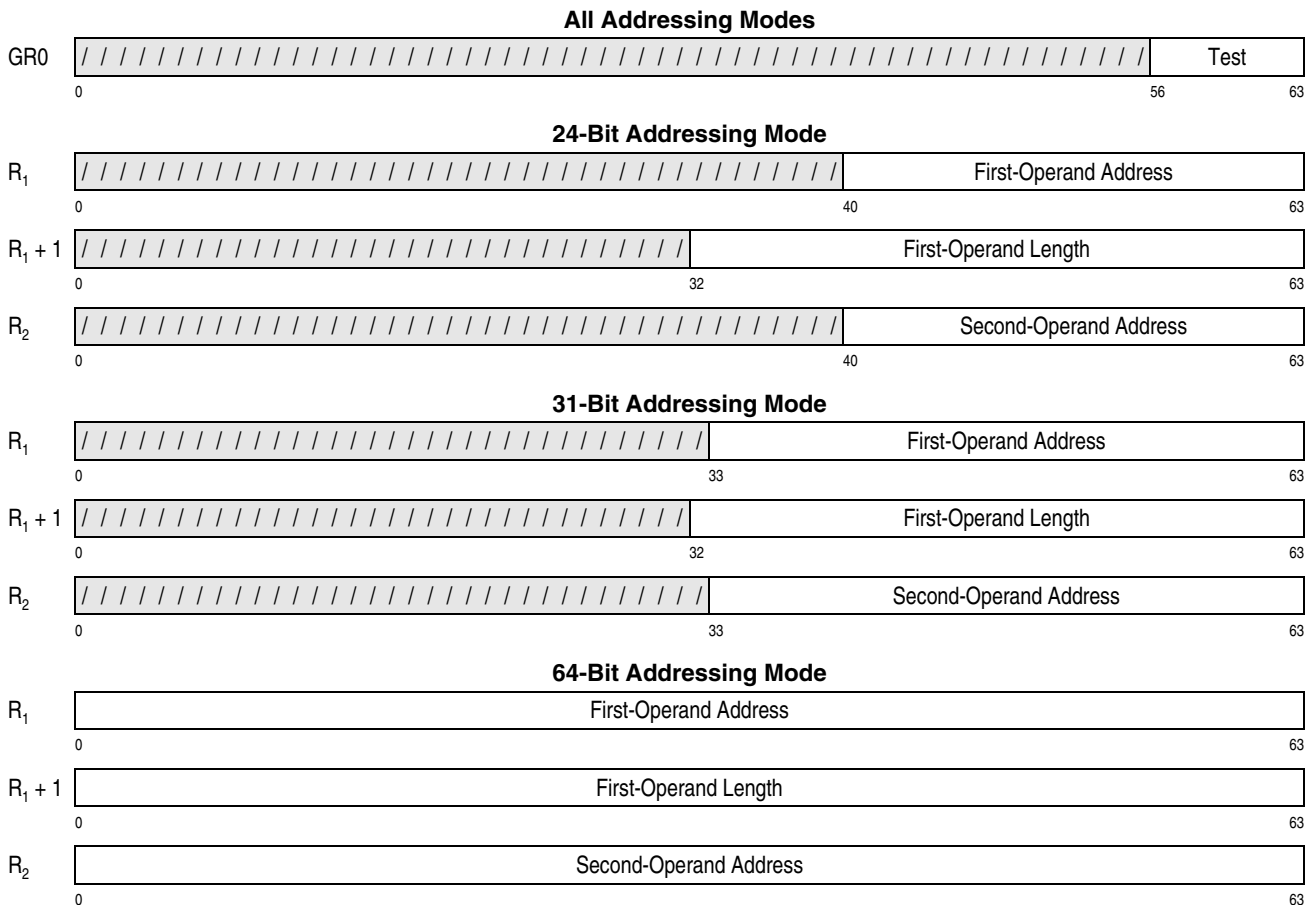
Figure 7-368. Register Contents for TRANSLATE EXTENDED
