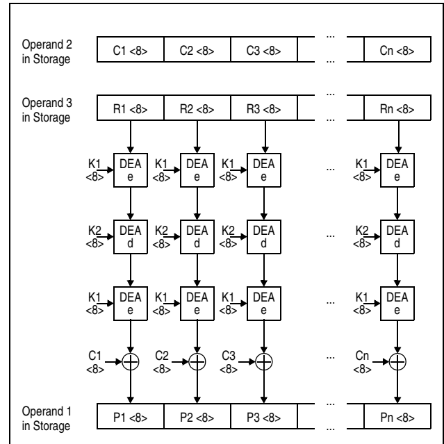
Figure 7-140. KMCTR TDEA Decipher Operation Using 128-Bit Key
