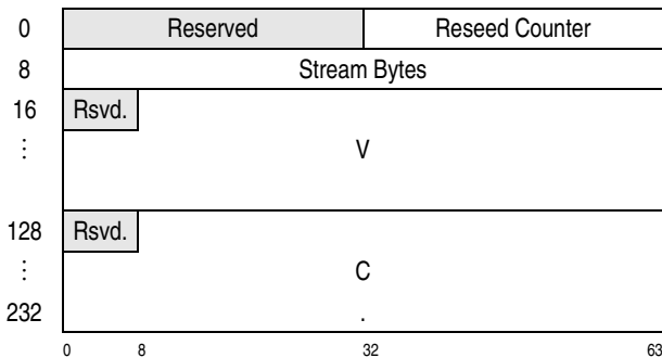
Figure 7-354. Parameter Block for PRNO-SHA-512-DRNG Function
