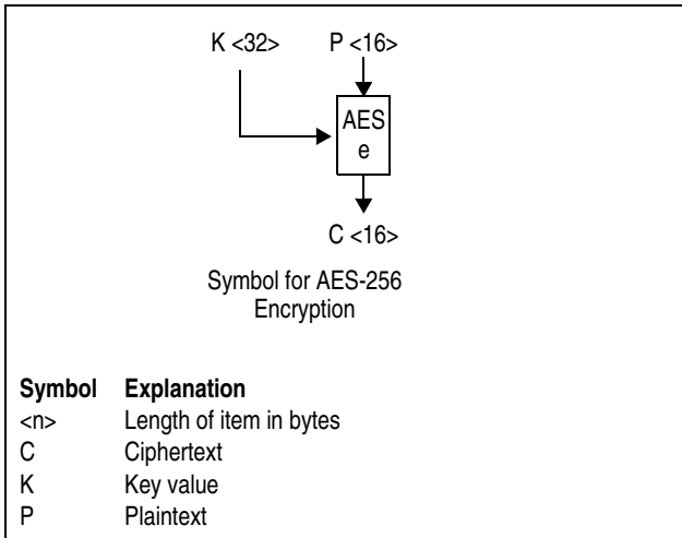
Figure 7-272. Symbols for AES-256 Encryption
