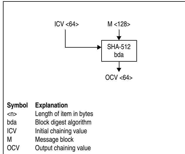
Figure 7-211. Symbol for SHA-512 Block Digest Algorithm
