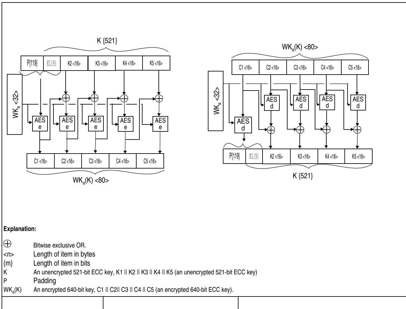
Figure 7-381. Encryption and Decryption of ECC Keys for P521 Using WK_a
