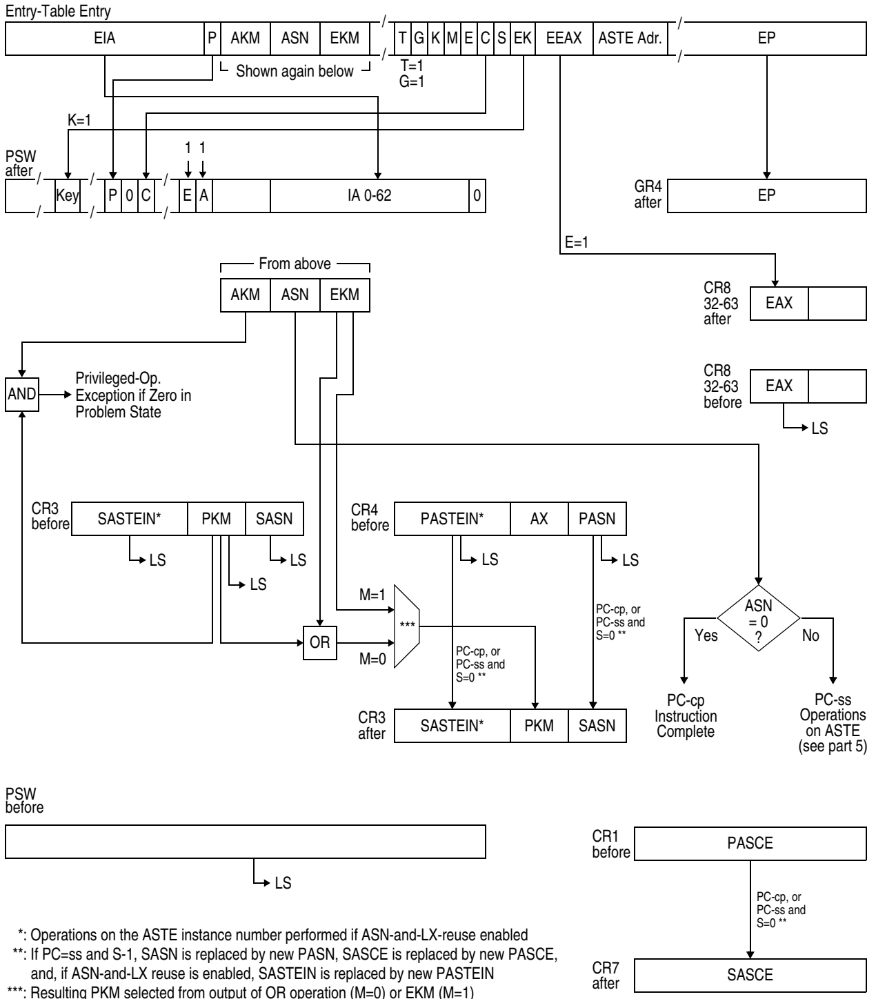
Figure 10-72. Execution of PROGRAM CALL (Part 3 of 5).
