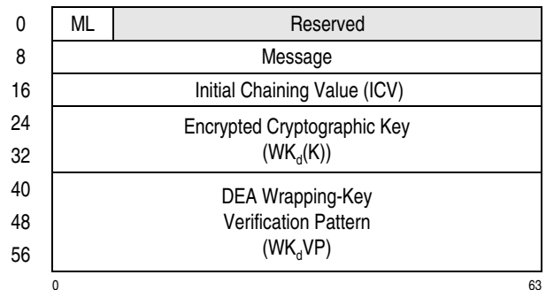
Figure 7-318. Parameter Block for PCC-Compute-Last-Block-CMAC-Using-Encrypted-TDEA-128
