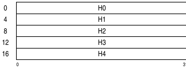
Figure 7-214. Parameter Block for KIMD-SHA-1
