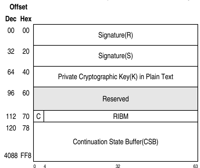
Figure 26-16. Parameter Block for KDSA-EdDSA-Sign-Ed25519 Functions
