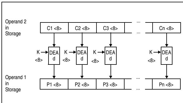
Figure 7-18. KM-DEA Decipher Operation Using 64-Bit Key
