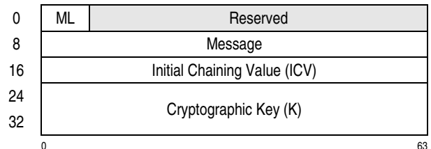
Figure 7-317. Parameter Block for PCC-Compute-Last-Block-CMAC-Using-TDEA-128
