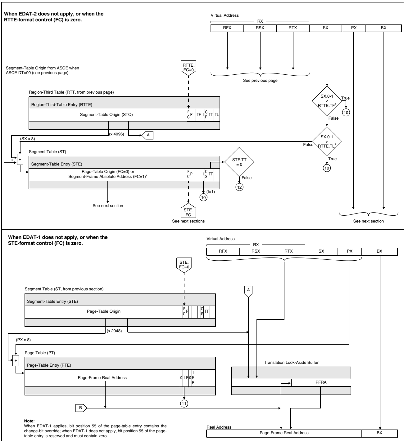
Figure 3-16. Translation Process (Part 2 of 3)
