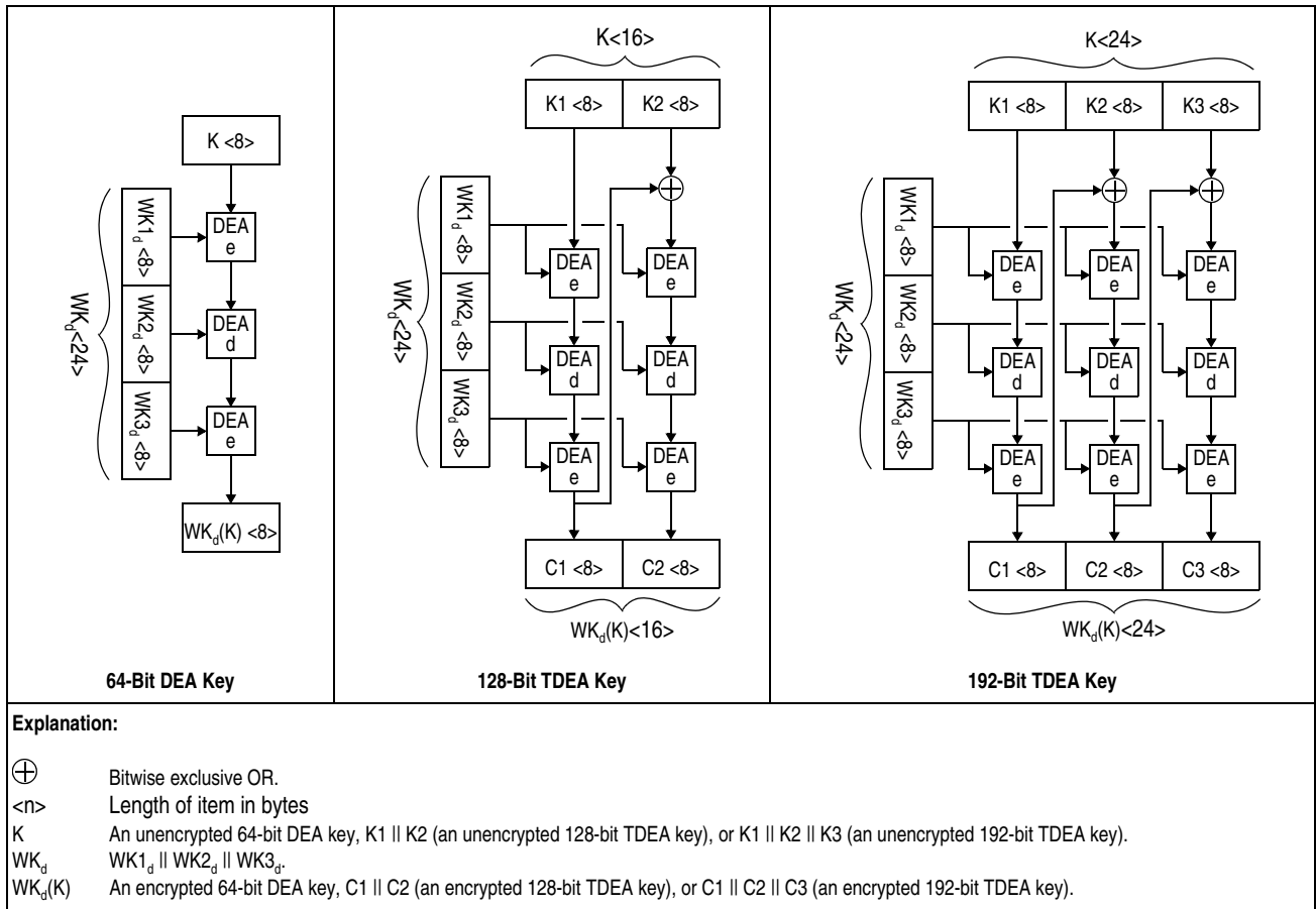
Figure 7-374. Encryption of DEA or TDEA Key Using WK_d
