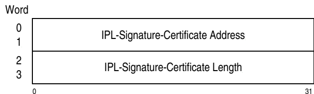
Figure 17-8. IPL-Signature-Certificate Entry
