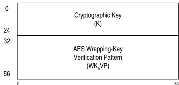
Figure 10-50. Parameter Block for PCKMO-Encrypt-ECC-Ed25519-Key
