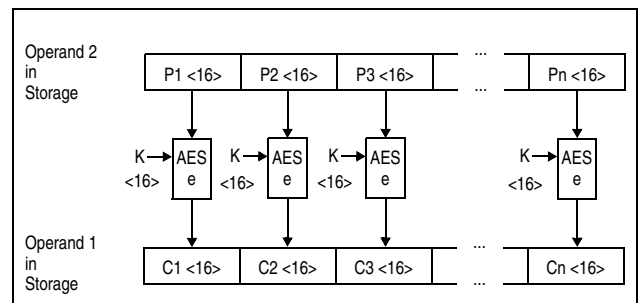
Figure 7-29. KM-AES Encipher Operation Using 128-Bit Key
