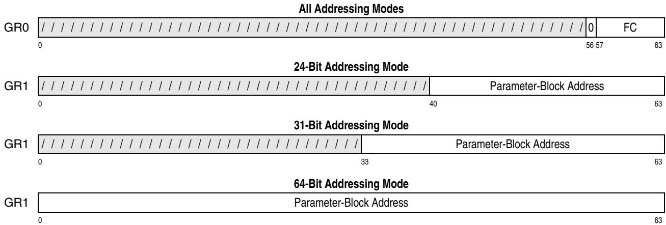
Figure 10-53. General Register Assignment for PERFORM TIMING FACILITY FUNCTION
