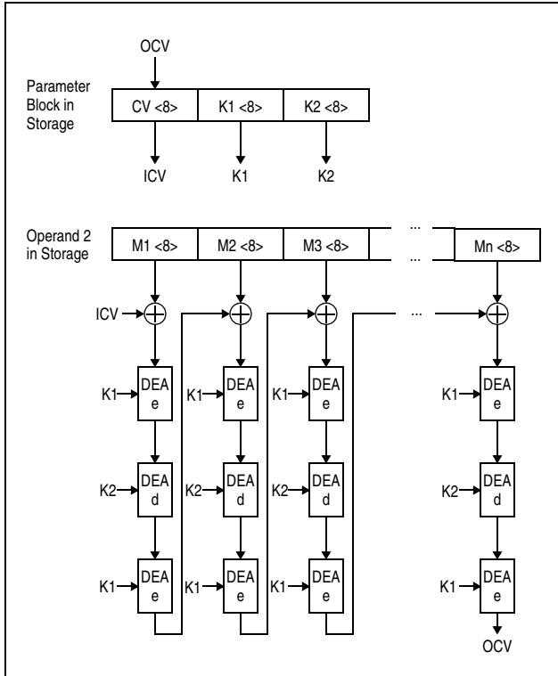
Figure 7-279. MAC Computation Using 128-bit TDEA Key
