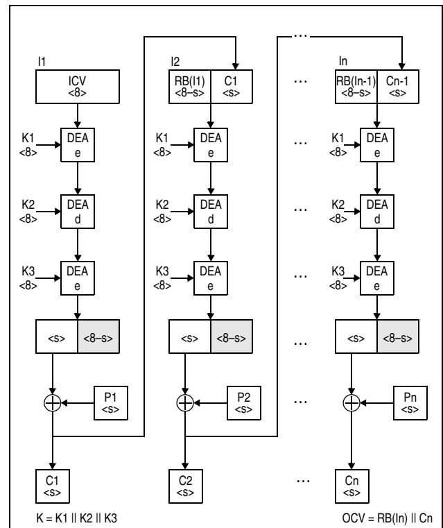
Figure 7-110. KMF-TDEA-192 Encipher Operation
