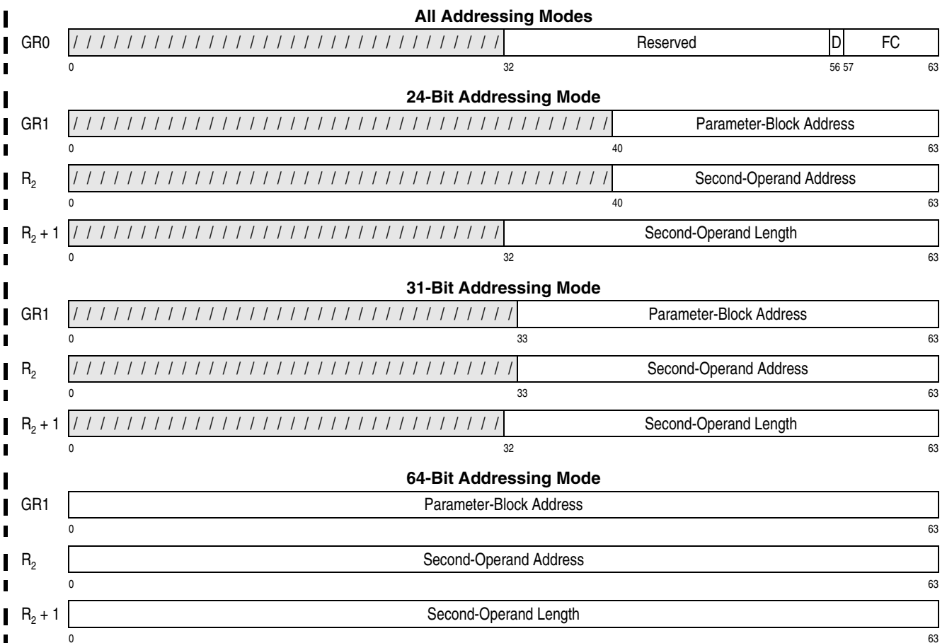
Figure 26-3. General Register Assignment for COMPUTE DIGITAL SIGNATURE AUTHENTICATION
