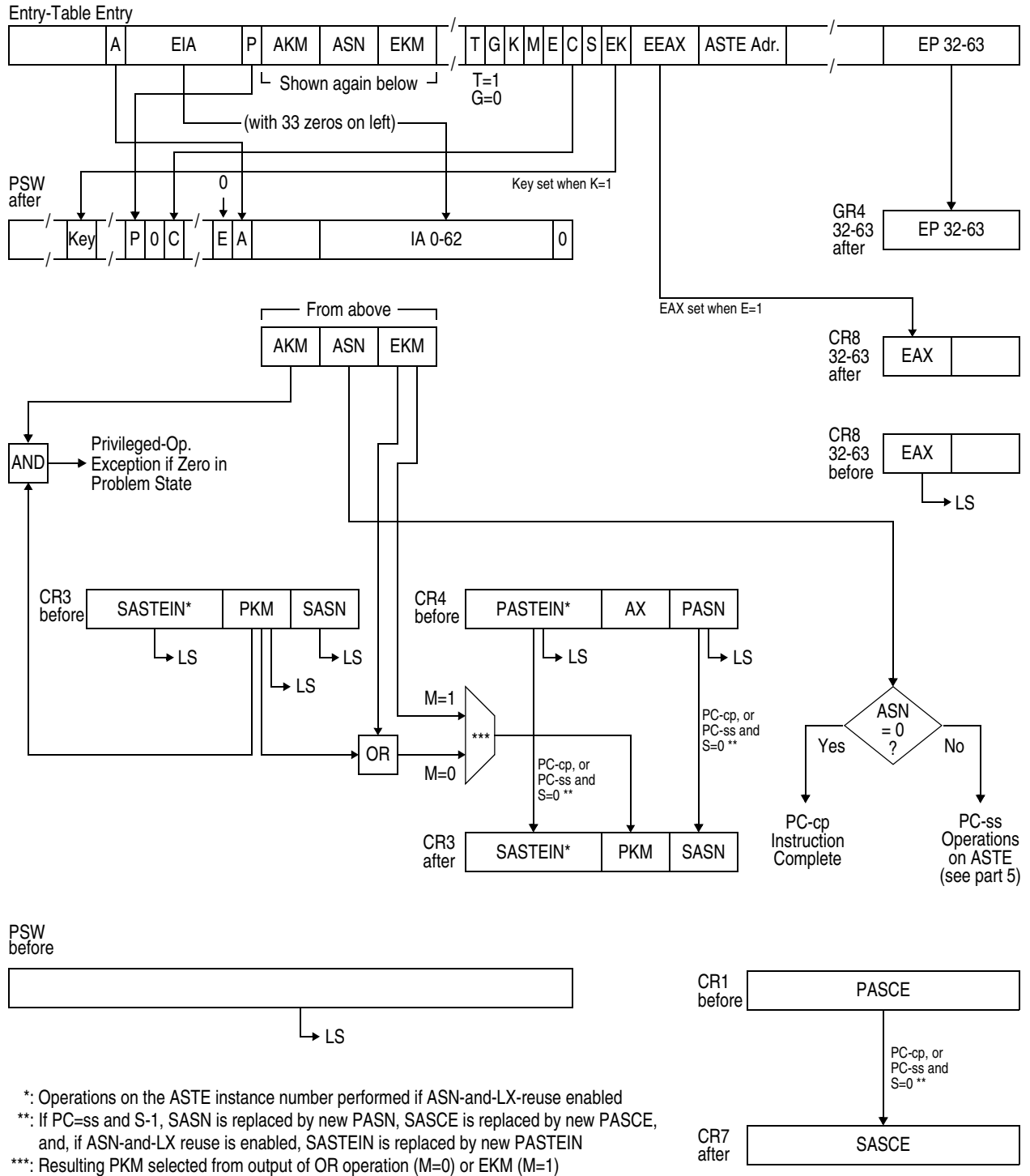
Figure 10-72. Execution of PROGRAM CALL (Part 4 of 5).
