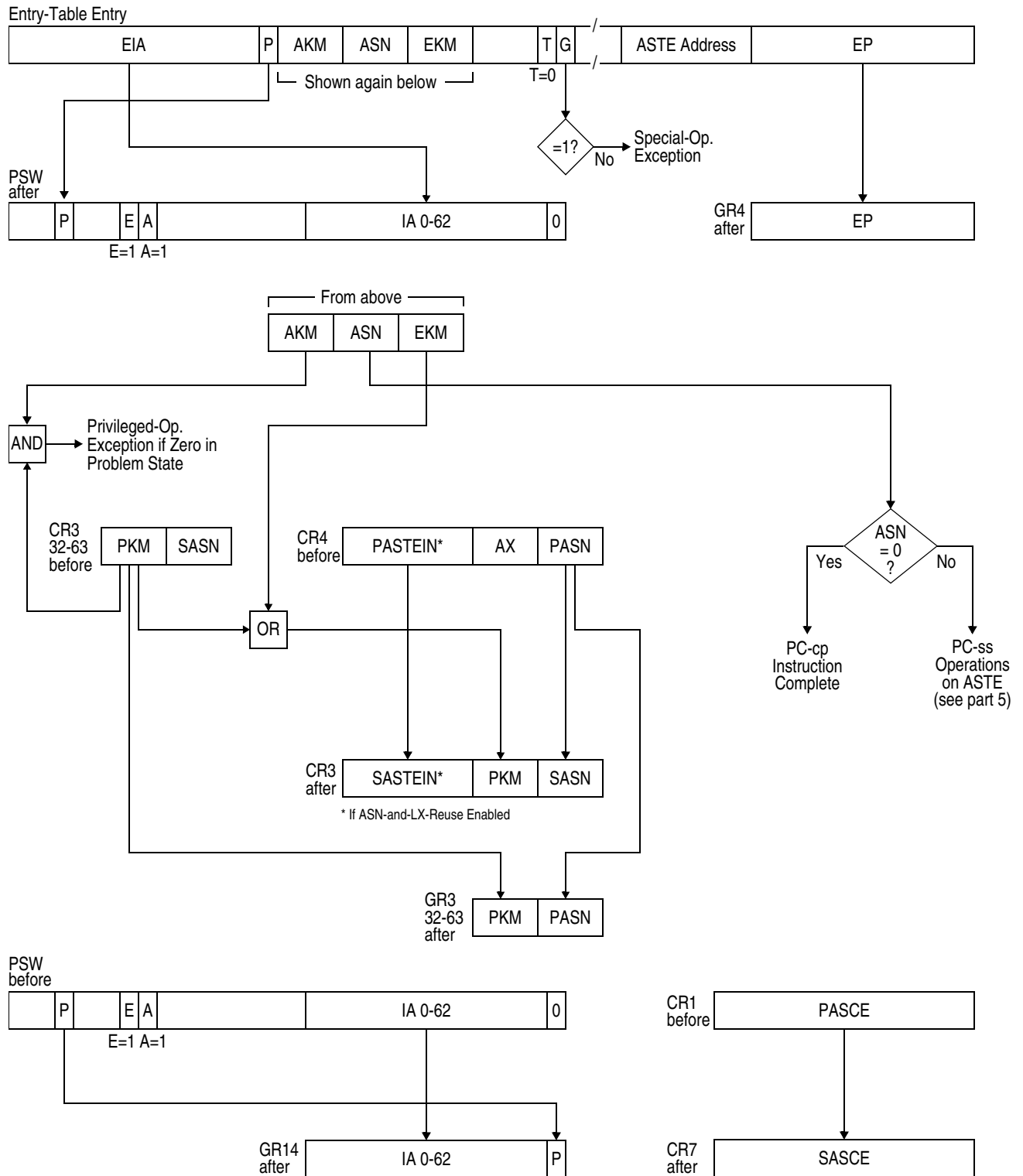
Figure 10-72. Execution of PROGRAM CALL (Part 2 of 5).
