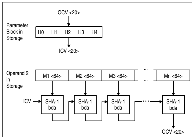
Figure 7-215. KIMD-SHA-1
