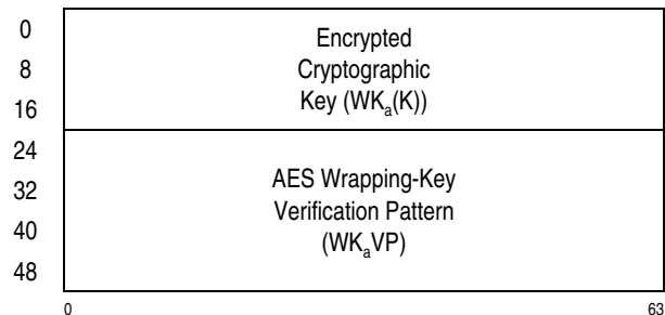
Figure 7-150. Parameter Block for KMCTR-Encrypted-AES-192
