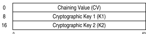
Figure 7-104. Parameter Block for KMF-TDEA-128
