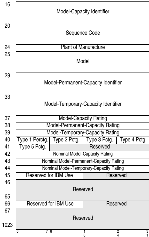
Figure 10-85. Format of the SYSIB 1.1.1 (Part 2 of 2)
