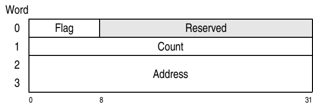
Figure 15-29. Transport-Indirect-Data-Address Word (TIDAW)
