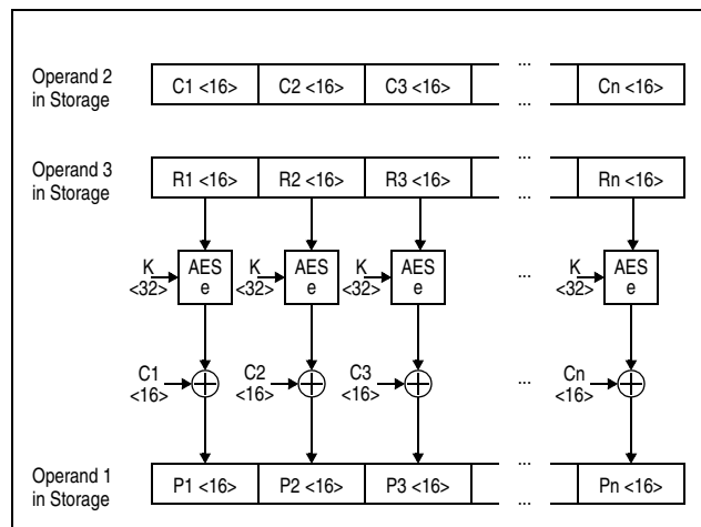
Figure 7-156. KMCTR AES Decipher Operation Using 256-Bit Key
