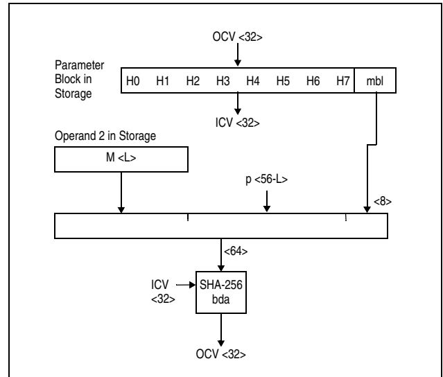
Figure 7-244. KLMD-SHA-256 Partial-Block Case 1 ( 1 \leq L \leq 55 )
