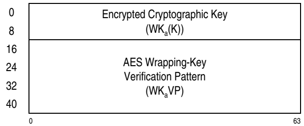
Figure 7-28. Parameter Block for KM-Encrypted-AES-128
