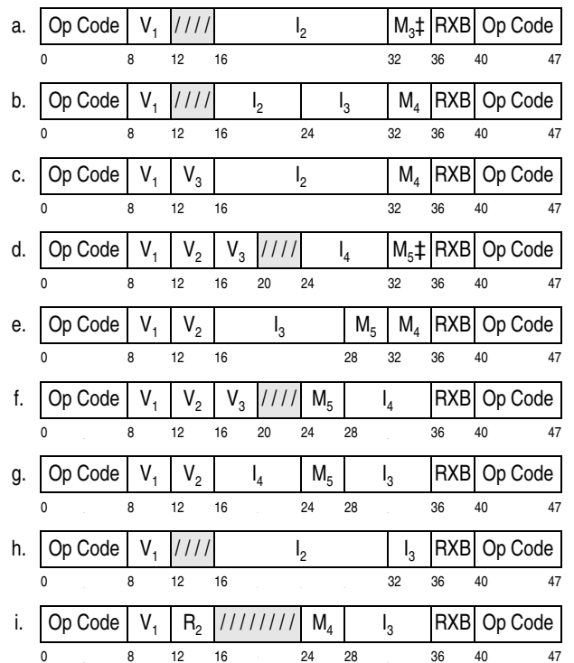
Figure 5-1. Basic Instruction Formats (Part 4 of 5)
