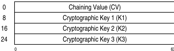
Figure 7-56. Parameter Block for KMC-TDEA-192
