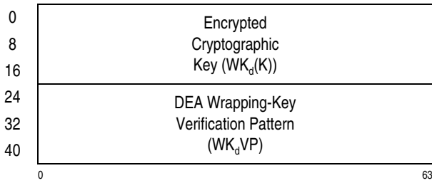
Figure 7-142. Parameter Block for KMCTR-Encrypted-TDEA-192
