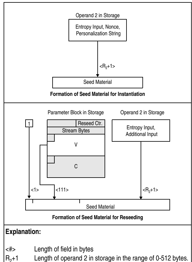
Figure 7-355. PRNO-SHA-512-DRNG Function's Seed Operation Generation of Seed Material
