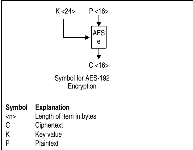
Figure 7-271. Symbols for AES-192 Encryption
