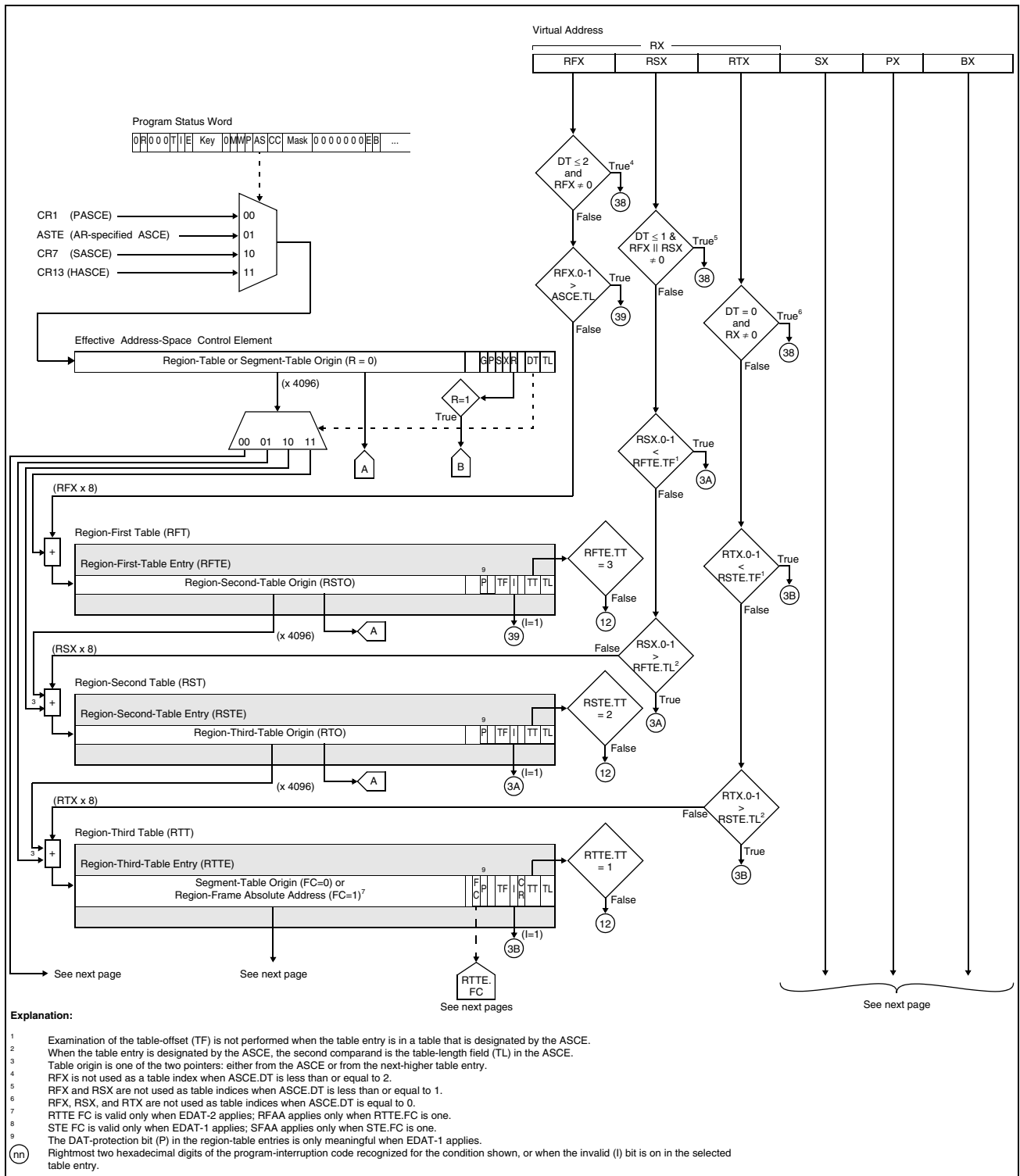
Figure 3-16. Translation Process (Part 1 of 3)
