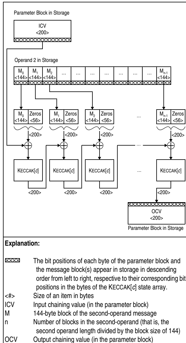
Figure 7-221. KIMD-SHA3-224 Processing
