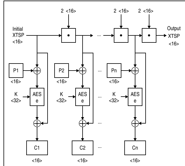
Figure 7-45. KM-XTS-AES-256 Encipher Operation
