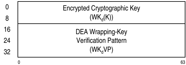
Figure 7-138. Parameter Block for KMCTR Encrypted-TDEA-128
