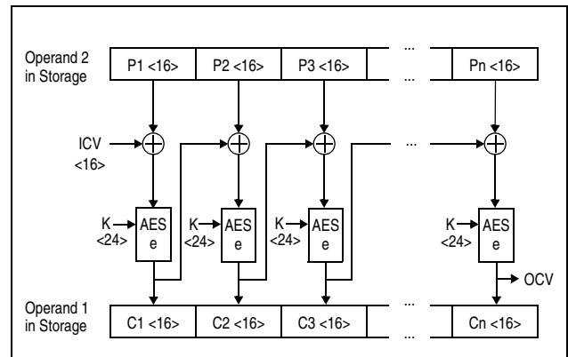
Figure 7-66. KMC AES Encipher Operation Using 192-Bit Key
