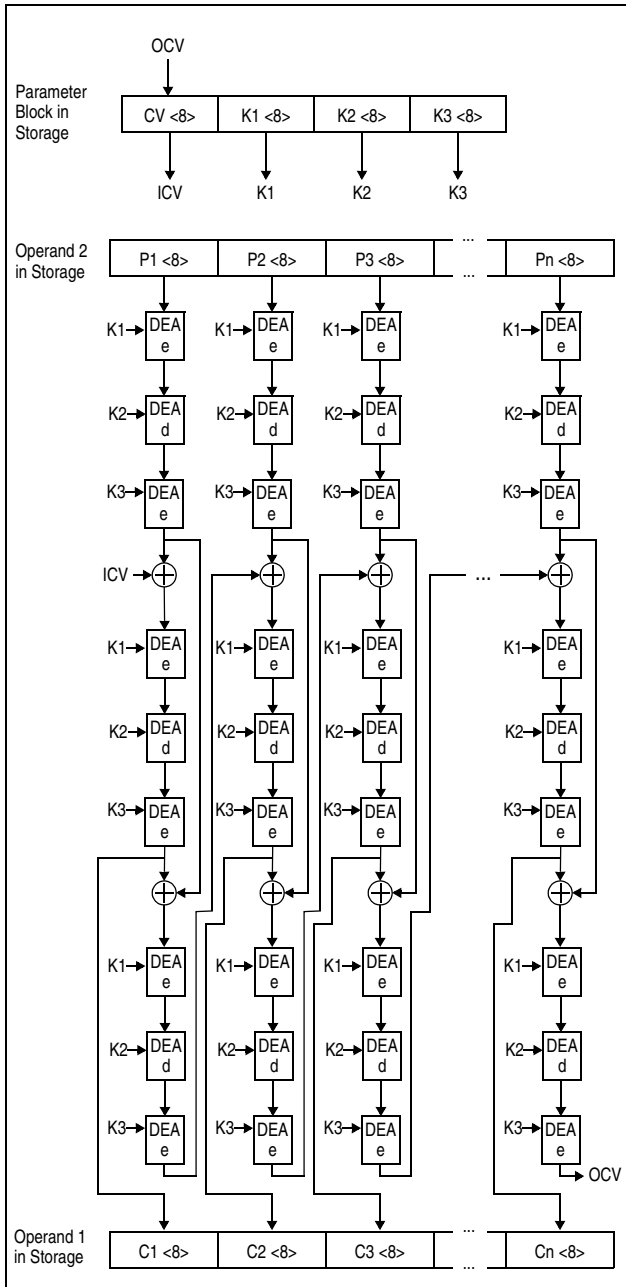
Figure 7-73. KMC-PRNG Operation
