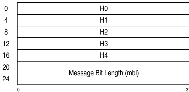
Figure 7-236. Parameter Block for KLMD-SHA-1
