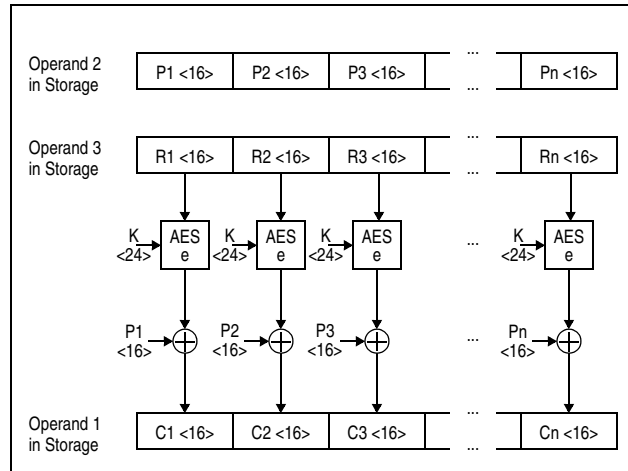
Figure 7-151. KMCTR AES Encipher Operation Using 192-Bit Key
