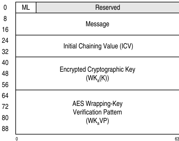
Figure 7-327. Parameter Block for PCC-Compute-Last-Block-CMAC-Using-Encrypted-AES-192
