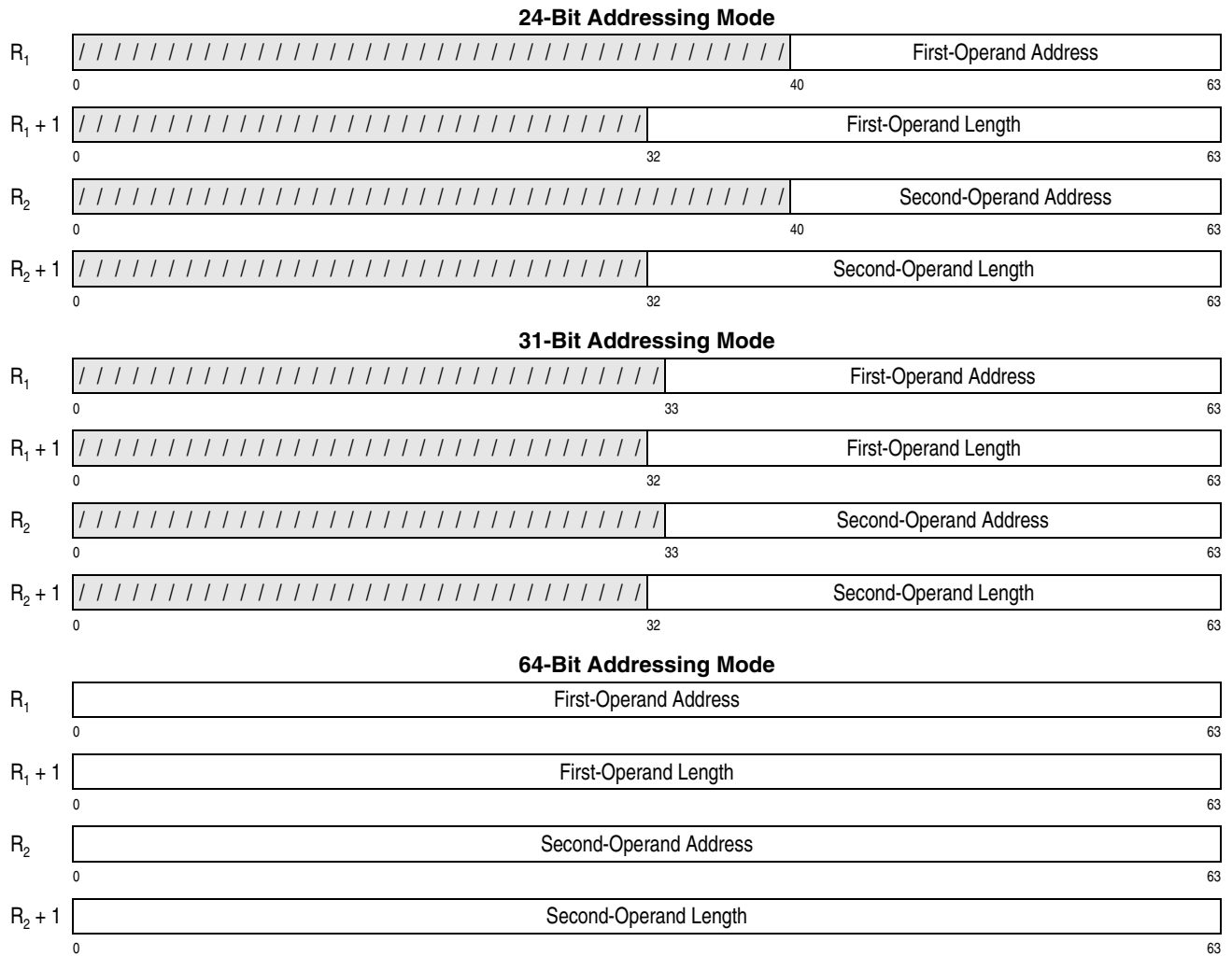
Figure 7-296. Register Contents for CONVERT UTF-32 TO UTF-8
