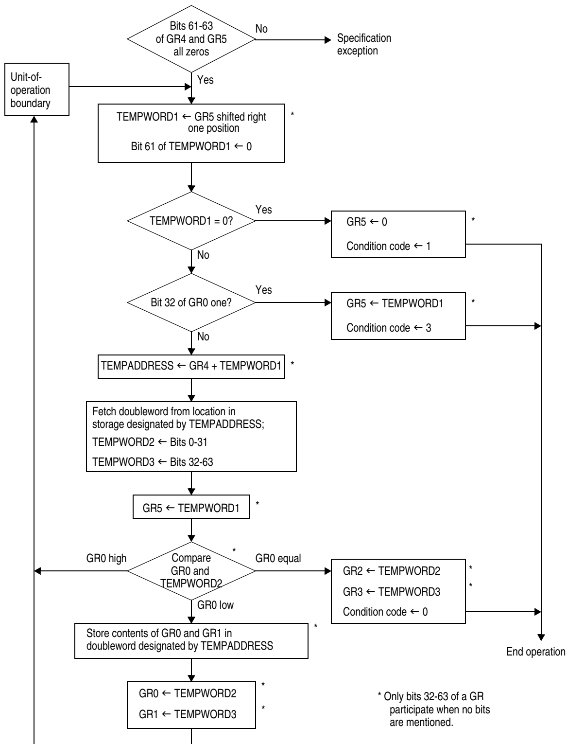
Figure 7-370. Execution of UPDATE TREE in the 24-Bit or 31-Bit Addressing Mode
