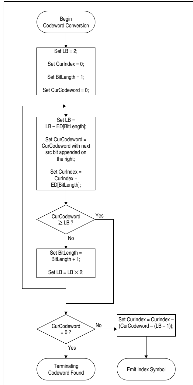
Figure 7-205. Entropy Encoded Expansion
