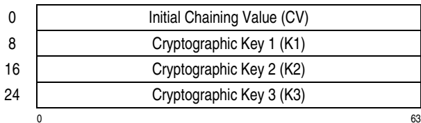
Figure 7-280. Parameter Block for KMAC-TDEA-192
