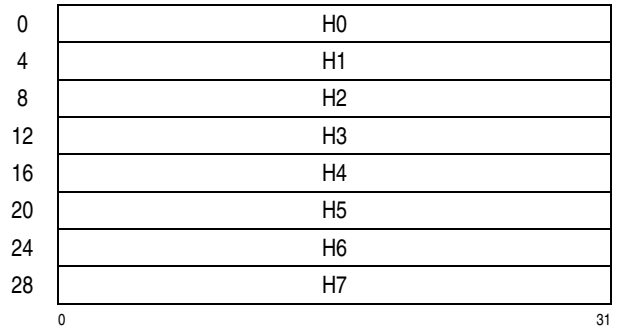
Figure 7-216. Parameter Block for KIMD-SHA-256
