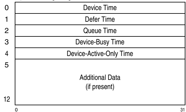
Figure 15-22. I/O-Status Transport-Status Area (TSA)
