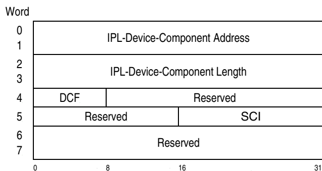
Figure 17-10. IPL-Device-Component Entry
