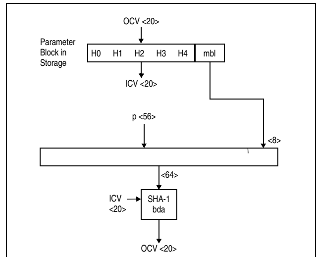
Figure 7-238. KLMD-SHA-1 Empty Block ( L = 0 )
