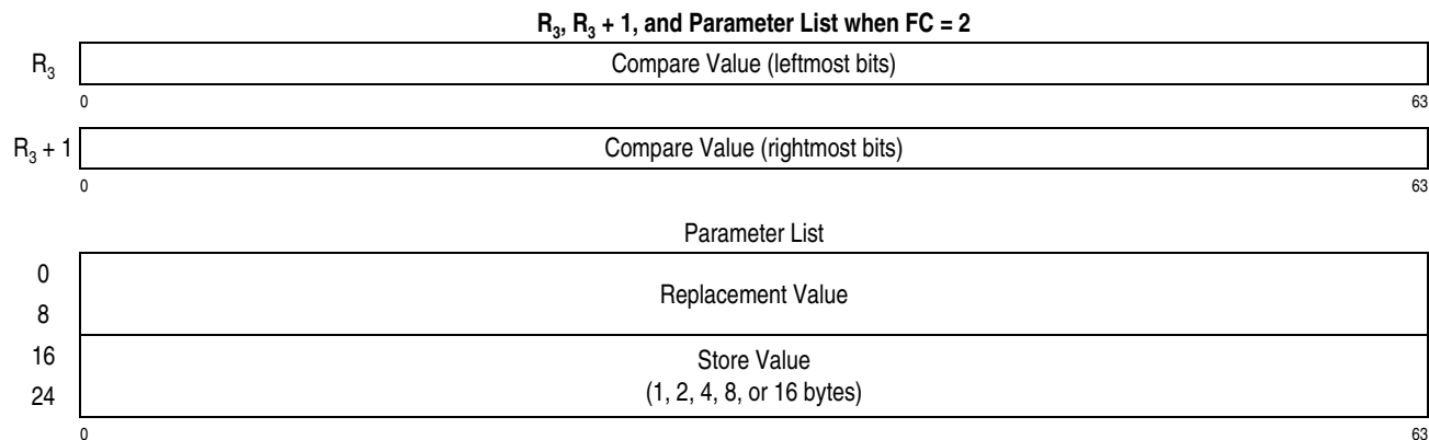
Figure 7-195. Register Contents for COMPARE AND SWAP AND STORE
