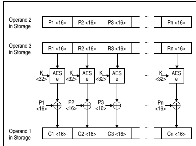
Figure 7-155. KMCTR AES Encipher Operation Using 256-Bit Key
