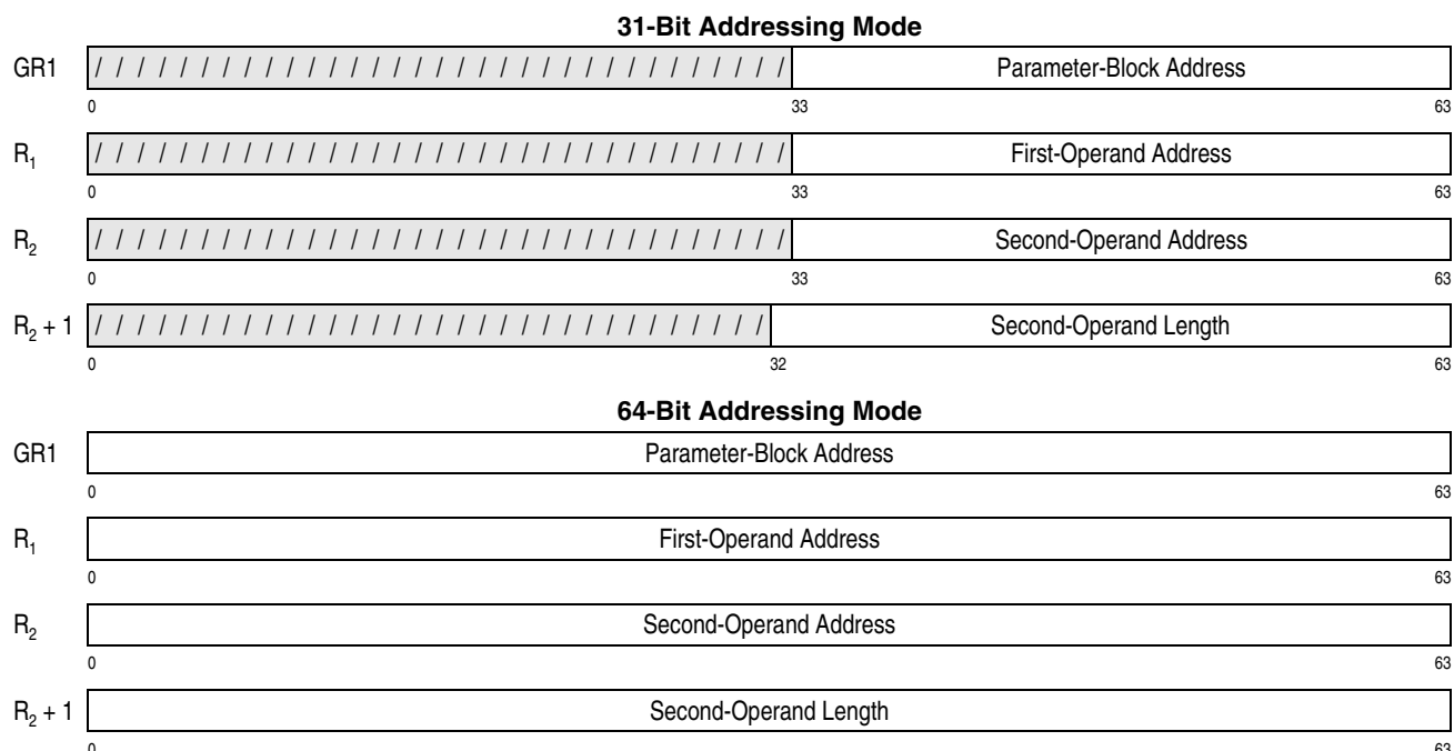
Figure 7-93. General Register Assignment for KMF (Part 2 of 2)
