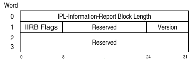
Figure 17-5. IPL-Information-Report BlockHeader
