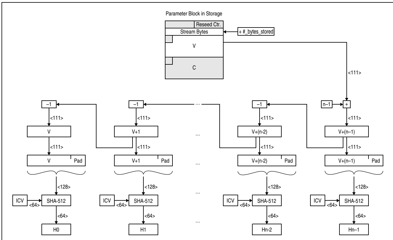
Figure 7-358. PRNO-SHA-512-DRNG Function's Generate Operation Generation of Deterministic Pseudorandom Numbers (Part 1 of 2)
