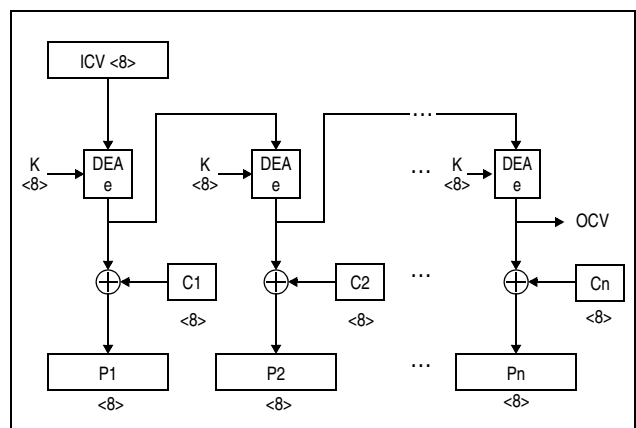
Figure 7-169. KMO-DEA Decipher Operation
