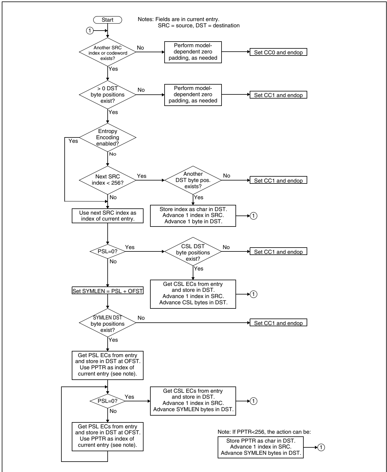
Figure 7-203. Expansion Process
