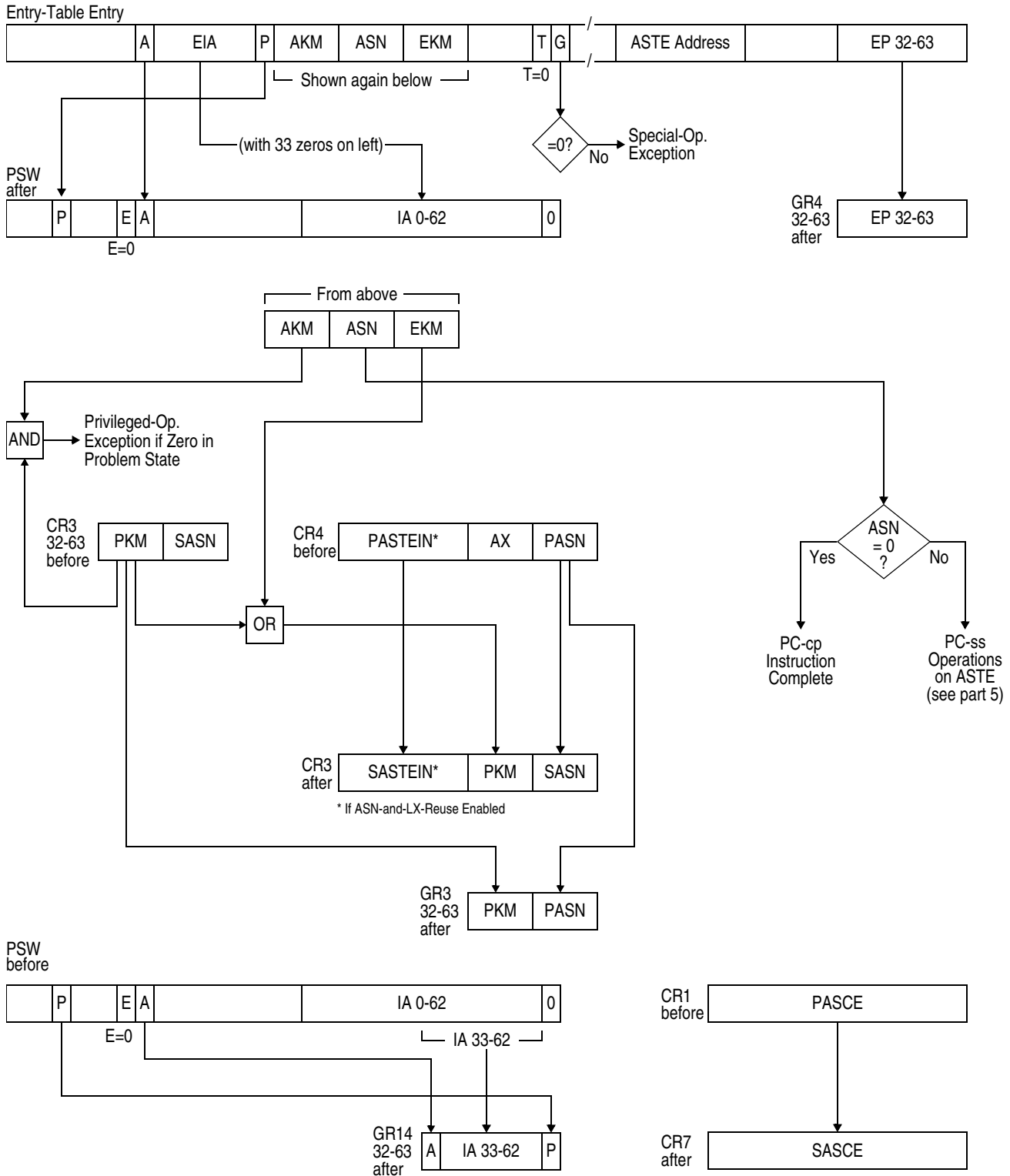
Figure 10-72. Execution of PROGRAM CALL (Part 1 of 5).
