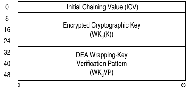
Figure 7-281. Parameter Block for KMAC-Encrypted-TDEA-192
