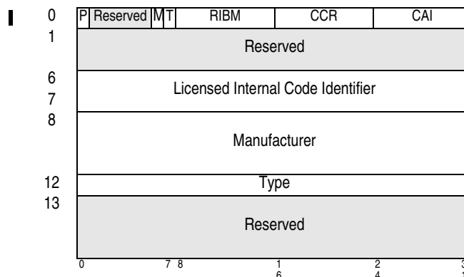
Figure 10-85. Format of the SYSIB 1.1.1 (Part 1 of 2)
