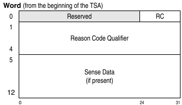
Figure 15-23. Device-Detected-Program-Check Transport-Status Area (TSA)
