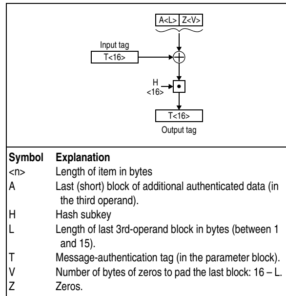
Figure 7-85. GHASH Processing of Last (Short) Block
