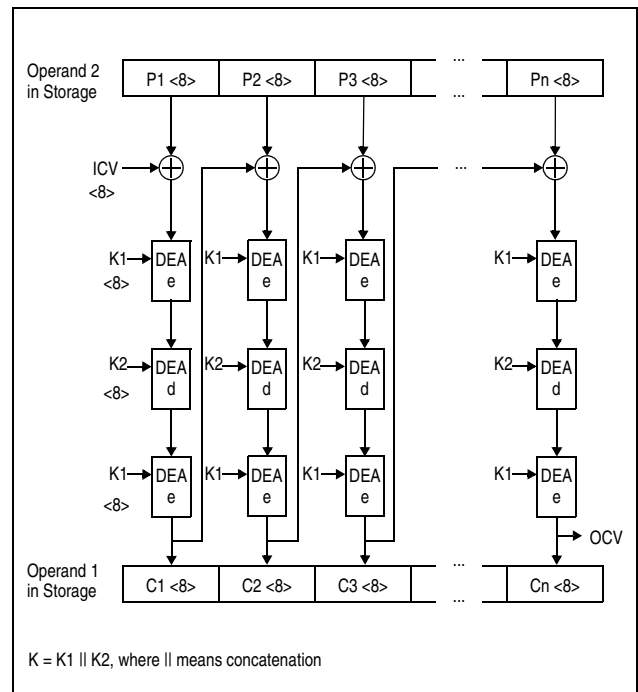
Figure 7-54. KMC TDEA Encipher Operation Using 128-Bit Key
