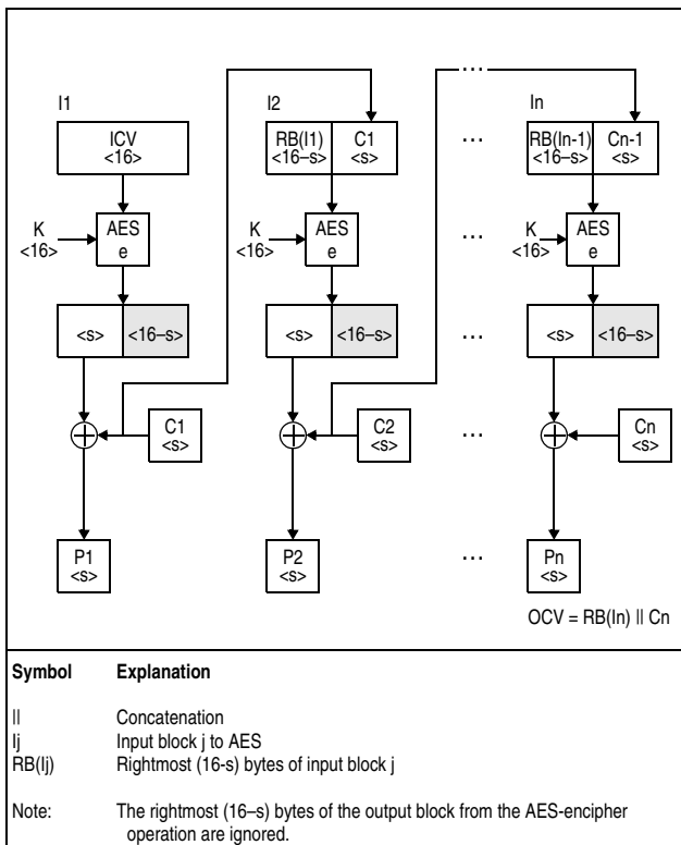
Figure 7-115. KMF-AES-128 Decipher Operation
