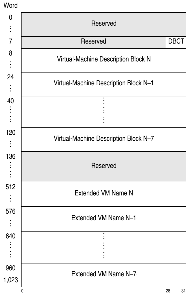
Figure 10-90. Format of the SYSIB 3.2.2
