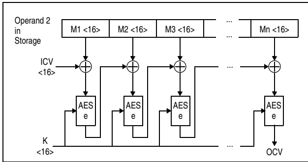
Figure 7-285. KMAC-AES-128
