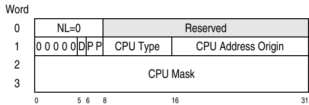
Figure 10-95. CPU-Type Topology-List Entry
