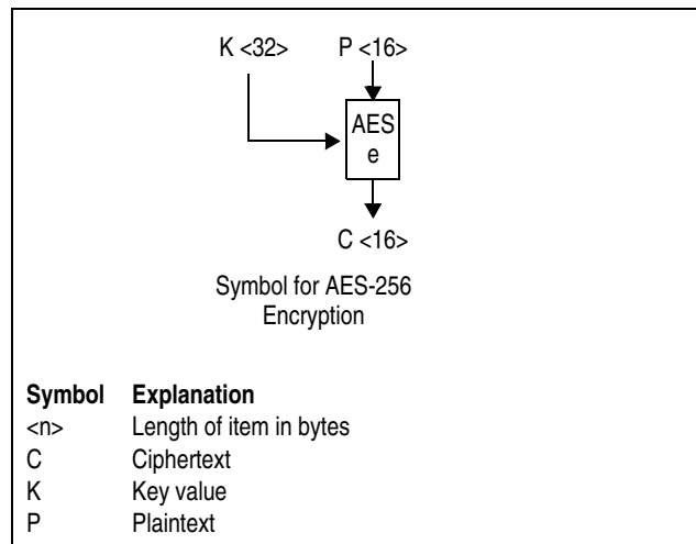
Figure 7-131. Symbols for AES-256 Encryption
