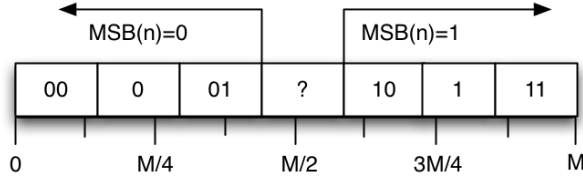
Figure 5: Mapping a random number n \in [M] to 7 buckets and the respective bits of n that are revealed given each bucket.
