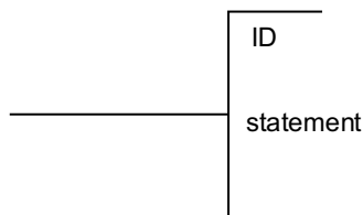
Figure C7.1 - Concrete Syntax for ArgumentReasoning
