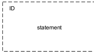
Figure C6.7 - Concrete Syntax for abstract asserted Claim
