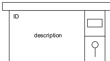
Figure C2 - Concrete Syntax for ArgumentPackageInterface
