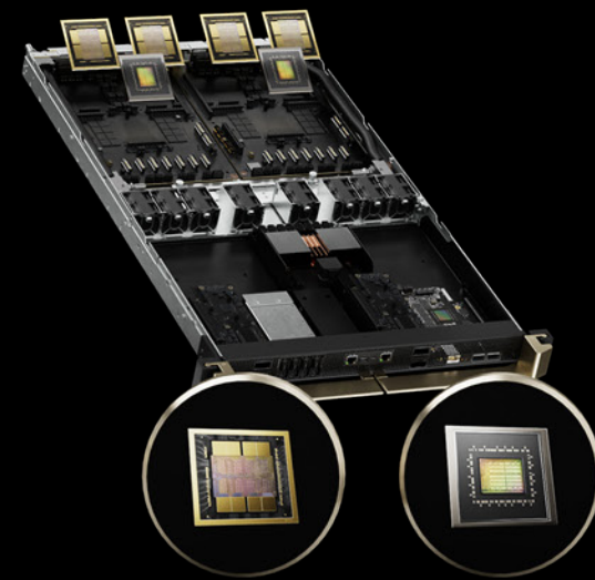
GB200 Superchip Compute Node
