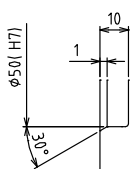
A部詳細図 Enlarged detail A
