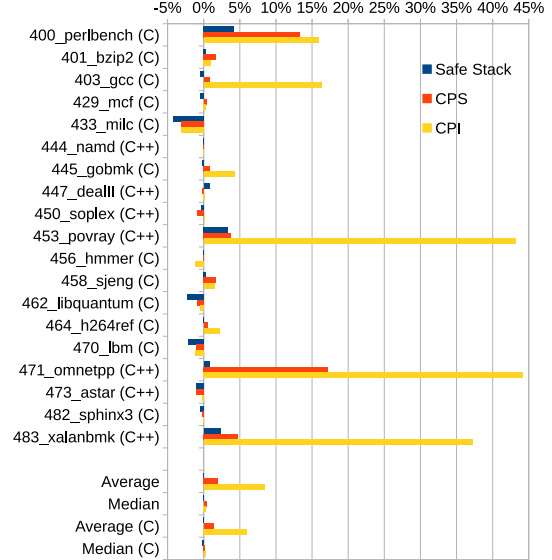
Figure 3: Levee performance for SPEC CPU2006, under three configurations: full CPI, CPS only, and safe stack only.
