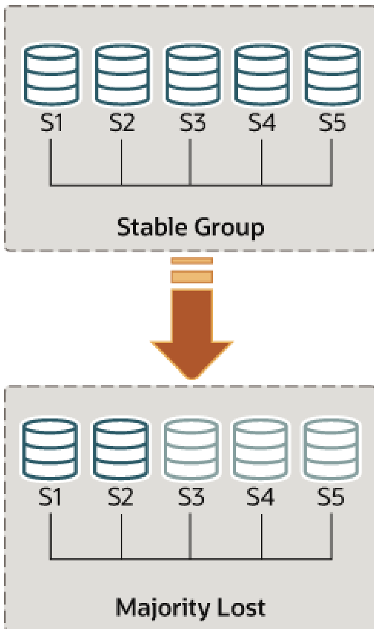
Figure 20.14 Losing Quorum
