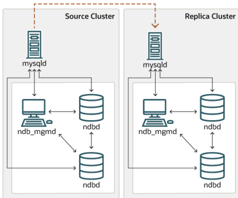
Figure 25.13 Replication Between SQL Nodes Connected Using IPv6
