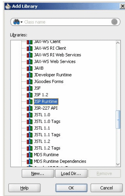
Figure 3–6 Importing Libraries
