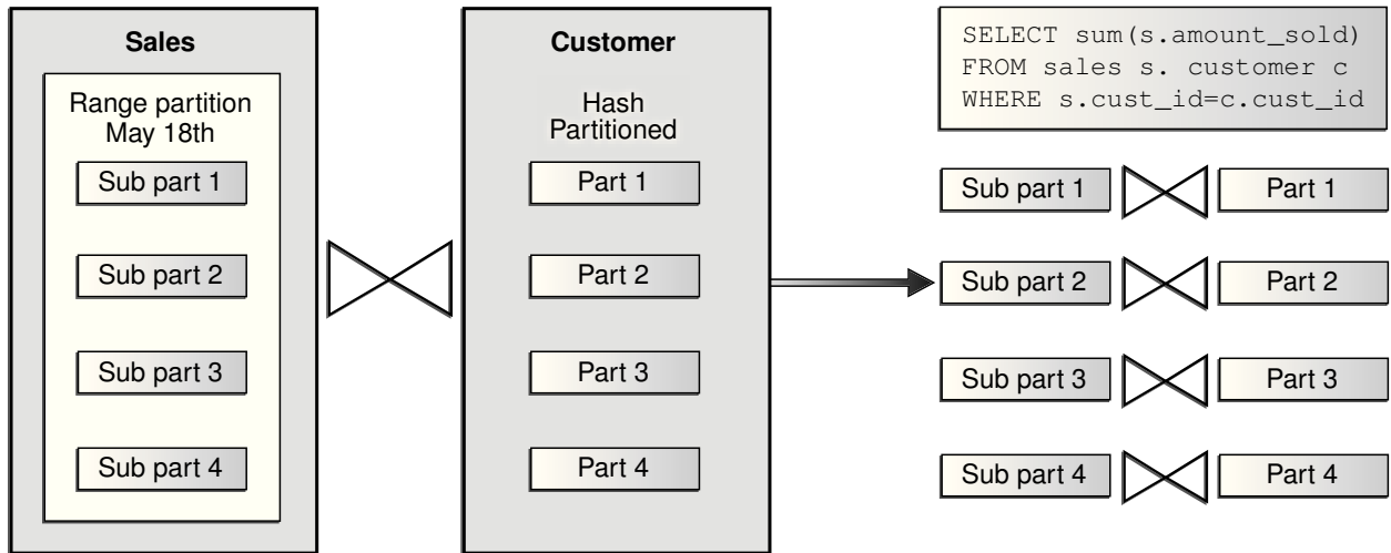
Figure 4-4 Full Partition-Wise Join
