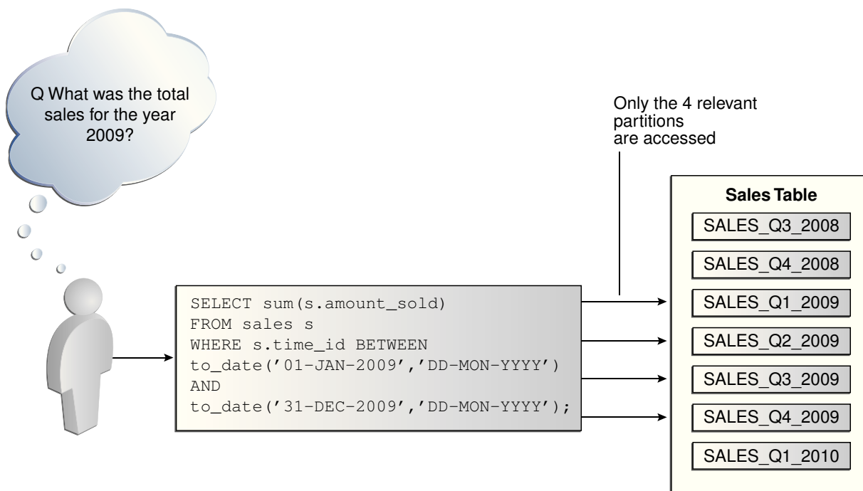
Figure 4-3 Partition Pruning
