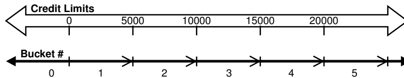
Figure 18-3 Bucket Assignments
