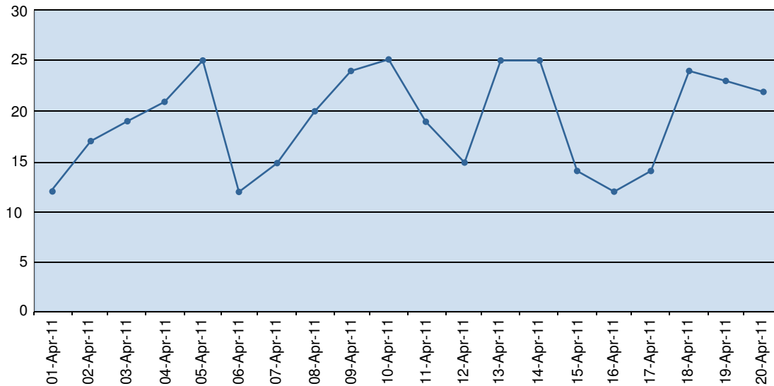
Figure 20-1 Stock Chart
