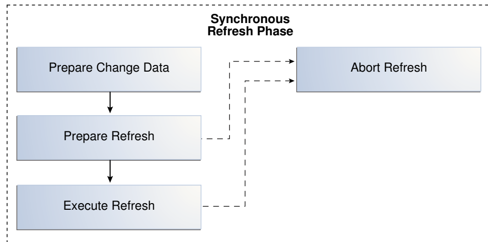
Figure 8-2 Refresh Phase
