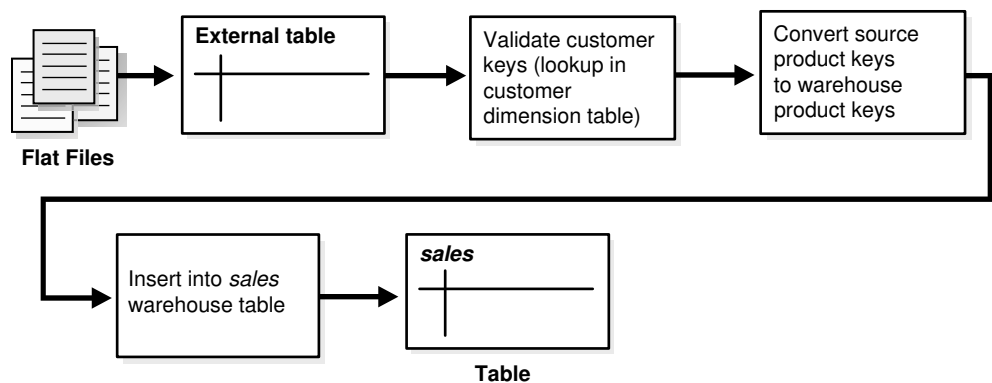
Figure 17-2 Pipelined Data Transformation
