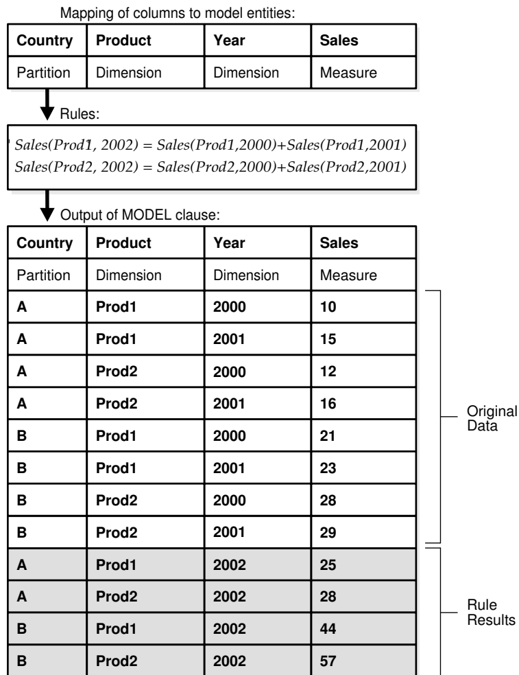
Figure 21-1 Model Elements
