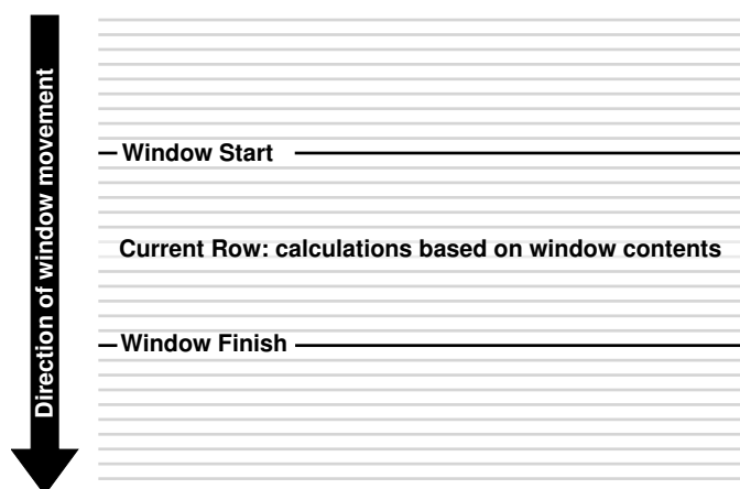
Figure 18-2 Sliding Window Example
