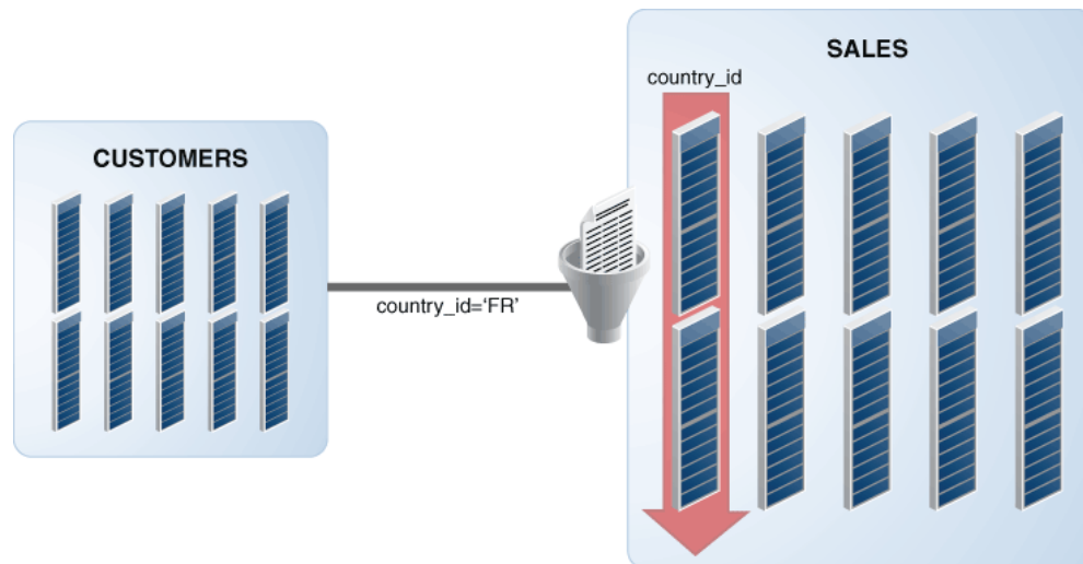
Figure 2-4 Vector Joins Using Oracle In-Memory Column Store
