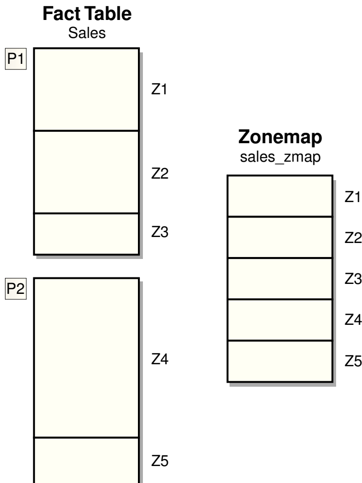
Figure 13-4 Zone Map for a Partitioned Fact Table
