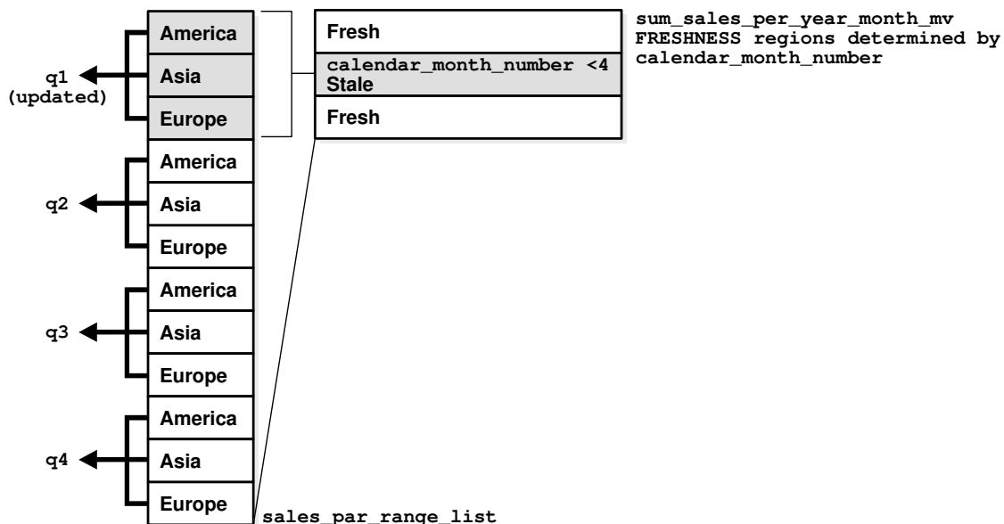
Figure 11-3 PCT Rewrite and Range-List Partitioning
