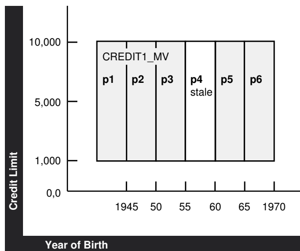
Figure 11-7 PCT and Multiple Materialized View Rewrite
