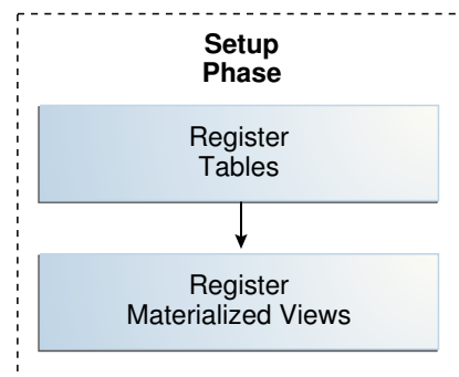
Figure 8-1 Registration Phase
