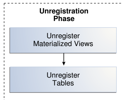
Figure 8-3 Unregistration Phase
