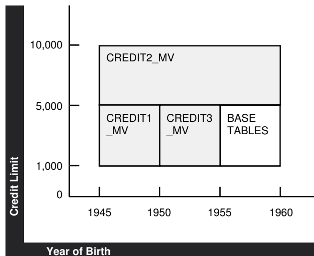
Figure 11-5 Query Rewrite Using Multiple Materialized Views
