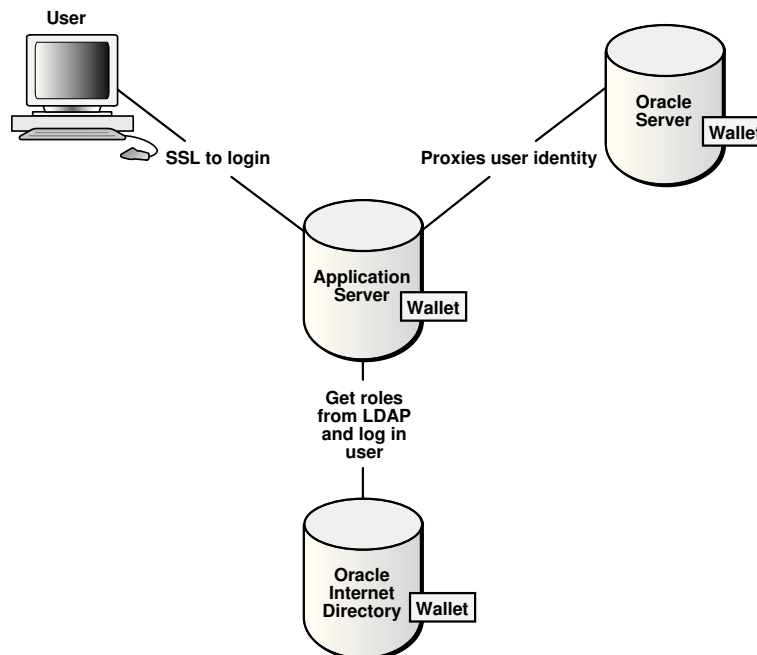
Figure 3-2 Multitier Authentication
