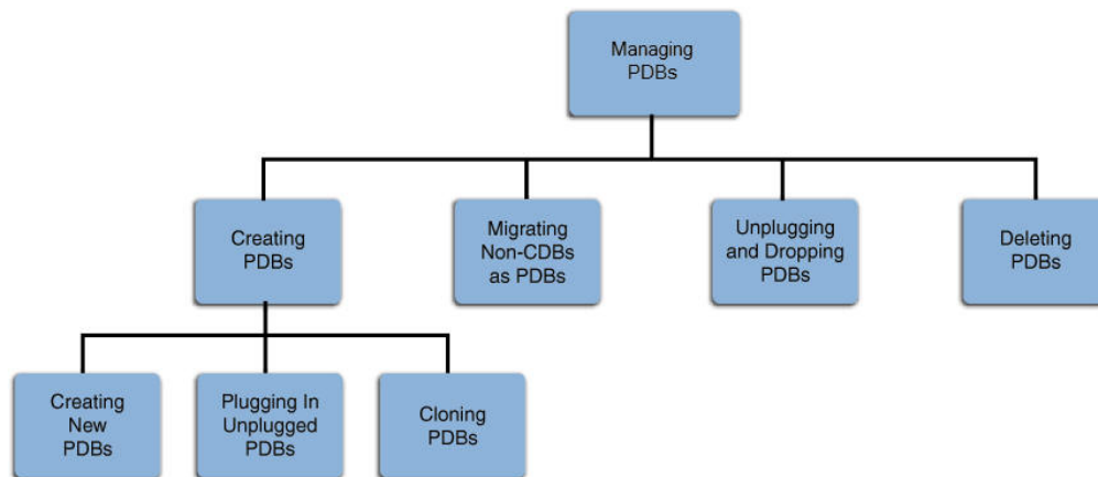
Figure 39-1 Managing PDBs
