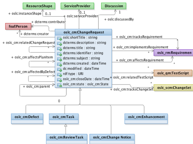
Fig. 1 OSLC Change Management 3.0 Overview
