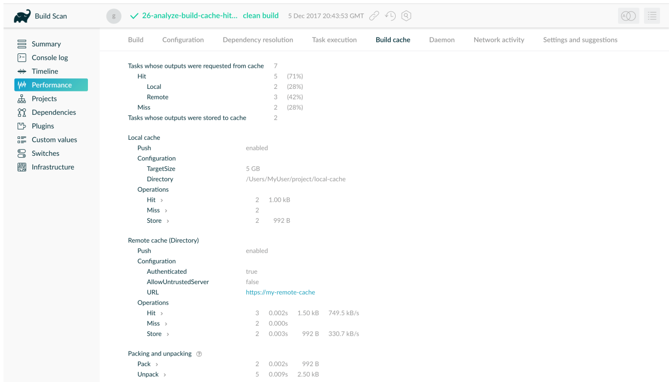
Figure 9. Inspecting the performance of the build cache for a build
