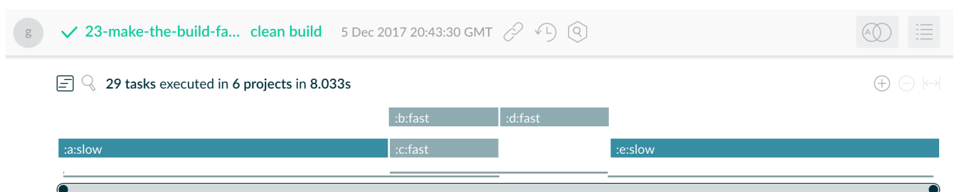
Figure 6. Bottleneck in parallel execution
