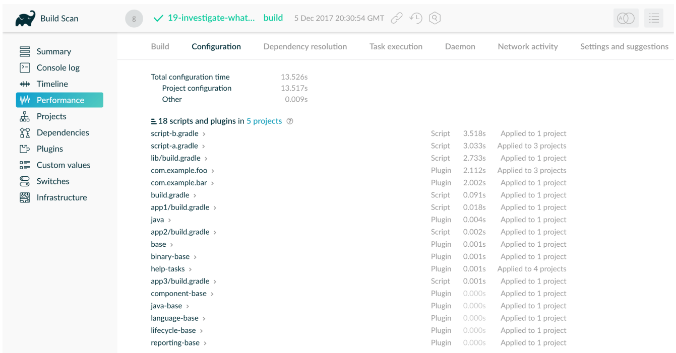
Figure 20. Build scan configuration breakdown
