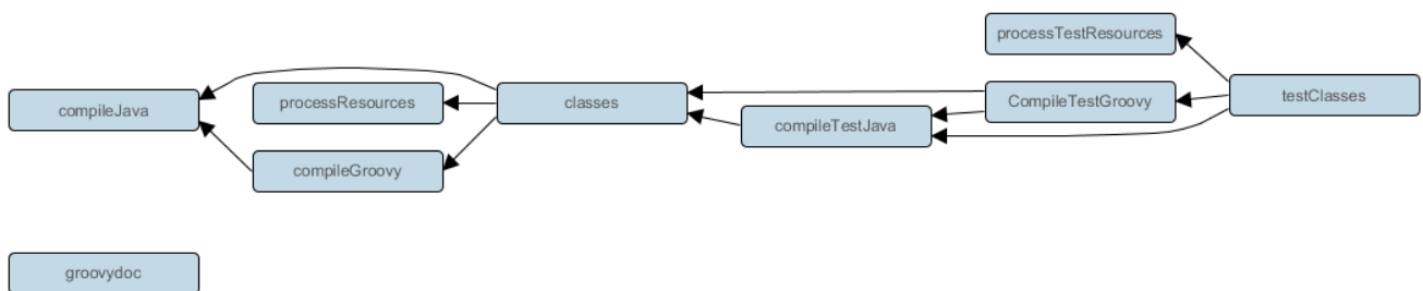
Figure 4. Groovy plugin - tasks
