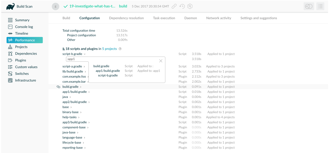
Figure 21. Showing the application of script-b.gradle to the build
