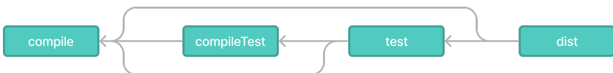
Figure 23. Simple Task Graph
