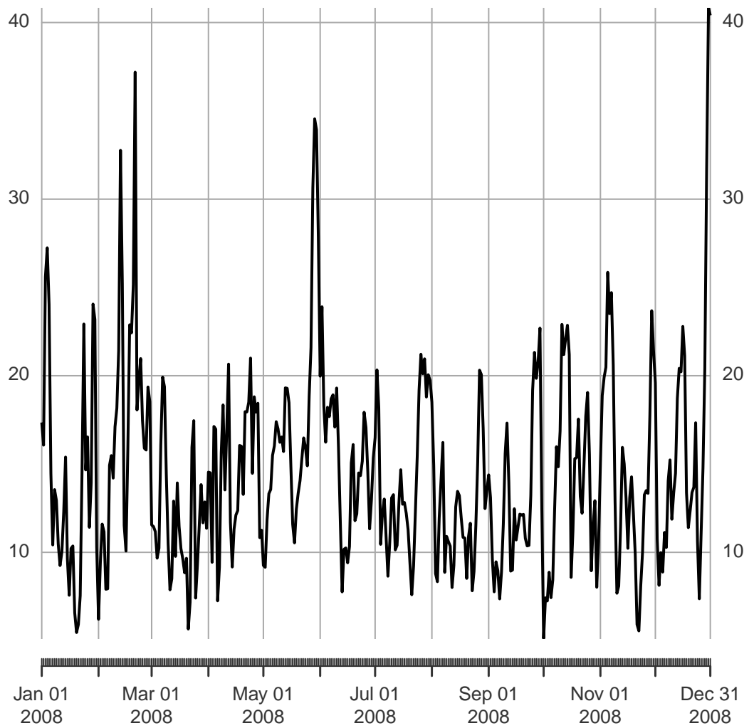
Figure 2: Time series plot of daily rural background PM10, averaged over Germany
