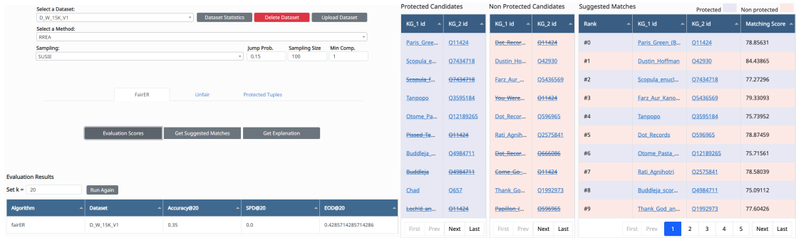
(a) Dataset selection and evaluation results. (b) Explaining the selection of suggested matches. Figure 2: Screenshots from the framework for different menu options, for KG data.
