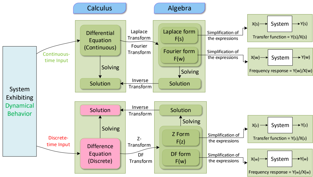
Figure 1: Transform Methods
