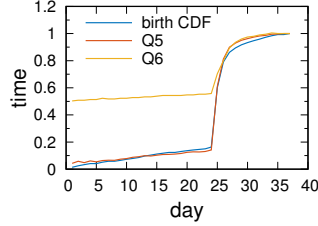
Figure 7: Effect of birth selection
