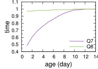
Figure 8: Effect of age selection
