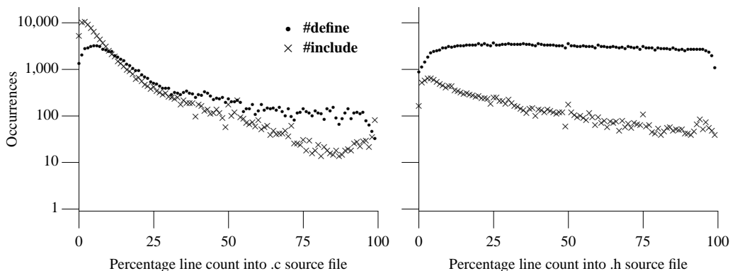
Figure 1854.2: Number of #include and #define directives appearing at a relative location (i.e., 100 \cdot \text{line\_number} / \text{lines\_in\_file} ) in the source. Based on the visible form of .c and .h files.
