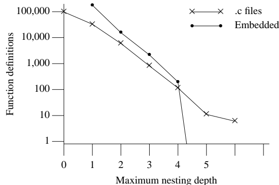
Figure 1763.2: Number of functions containing iteration-statements nested to the given maximum nesting level; for embedded C [397] (whose data was multiplied by a constant to allow comparison) and the visible form of the .c files (zero nesting depth denotes functions not containing any iteration-statements ).
