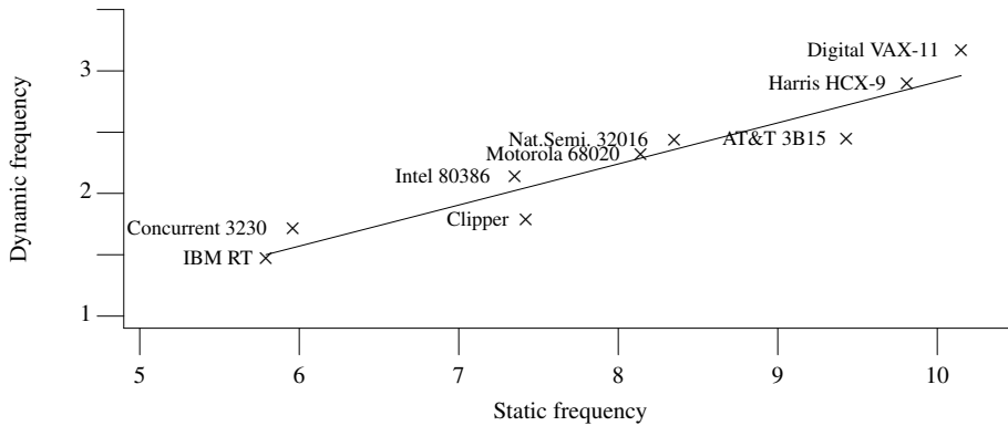
Figure 0.5: Dynamic/static frequency of call instructions. Adapted from Davidson. [330]
