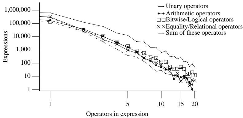
Figure 940.3: Number of expressions containing a given number of various kinds of operator, plus a given number of all of these kinds of operators. The set of unary operators are the unary-operators plus the prefix/postfix forms of ++ and --. The set of arithmetic operators are the binary operators *, /, %, +, -, and the unary operators + and -. Based on the visible form of the .c files.
