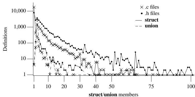
Figure 297.1: Number of structure and union type definitions containing a given number of members (members in any nested definitions are not included in the count of members of the outer definition). Based on the visible form of the .c and .h files.
