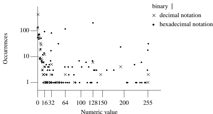
Figure 1244.1: Number of integer-constants having a given value appearing as the right operand of the bitwise-OR operator. Based on the visible form of the .c files.
