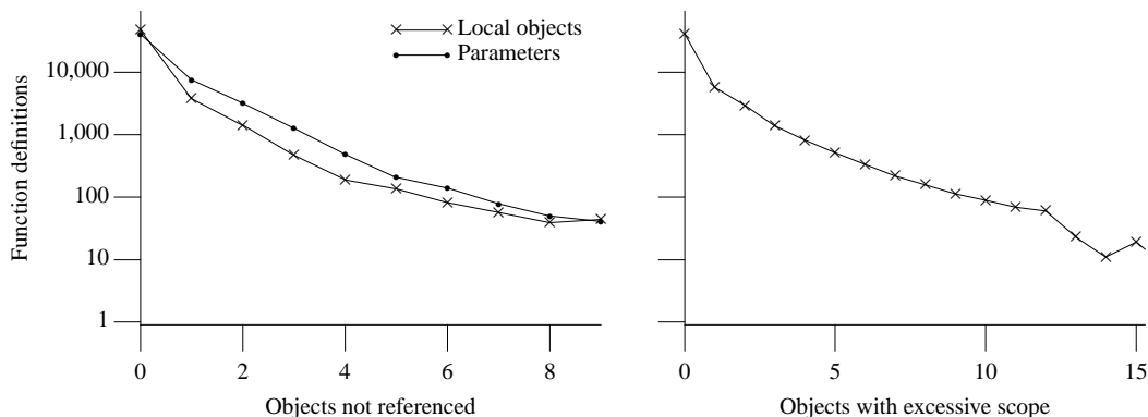
Figure 190.1: Number of parameters or locally defined objects that are not referenced within a function definition (left); number of objects declared in a scope that is wider than that needed for any of the references to them within a function definition (right). Based on the translated form of this book’s benchmark programs.
