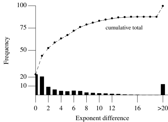
Figure 334.2: Difference in the value of the exponents (in powers of 2) of the two operands of floating-point addition and subtraction operations, obtained by executing the SPEC FP92 benchmarks. Adapted from Oberman. [1041]
