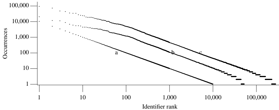
Figure 792.26: Identifier rank (based on frequency of occurrence of identifiers having a particular spelling) plotted against the number of occurrences of the identifier in the visible source of the .c files in (a) PostgreSQL, (b) Mozilla, and (c) Linux 2.4 kernel. Every identifier is represented by a dot. Fitting a power law to each plot using MLE gives an exponent of -2 (within a few percent -2 is the best fit for all of the projects used for the book's measurements, both for all the .c files and all the .h files). Also see Figure 1896.4.
