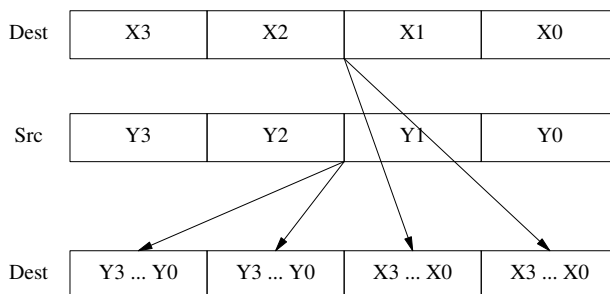
Figure 940.1: The SHUFPS (shuffle packed single-precision floating-point values) instruction, supported by the Intel Pentium processor, [637] places any two of the four packed floating-point values from the destination operand into the two low-order doublewords of the destination operand, and places any two of the four packed floating-point values from the source operand into the two high-order doublewords of the destination operand. By using the same register for the source and destination operands, the SHUFPS instruction can shuffle four single-precision floating-point values into any order.
