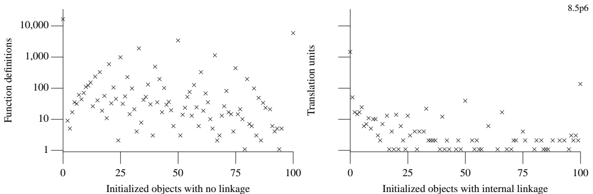
Figure 1652.1: Number of object declarations that include an initializer (as a percentage of all corresponding object declarations), either within function definitions (functions that did not contain any object definitions were not included), or within translation units and having internal linkage (while there are a number of ways of counting objects with external linkage, none seemed appropriate and no usage information is given here). Based on the translated form of this book's benchmark programs.
