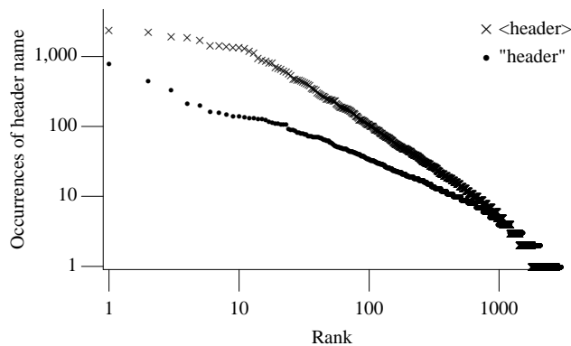
Figure 1896.4: header-name rank (based on character sequences appearing in #include directives) plotted against the number of occurrences of each character sequence. Also see Figure 792.26. Fitting a power law using MLE for <header-name> and "header-name" gives respective an exponent of -2.26, x_{min} = 8 , and -1.8, x_{min} = 9 . Based on the visible form of the .c files.
