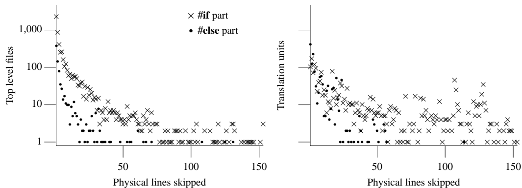
Figure 1899.1: Number of top-level source files (i.e., the contents of any included files are not counted) and (right) complete translation units (including the contents of any files #included more than once) having a given number of lines skipped during translation of this book's benchmark programs.
