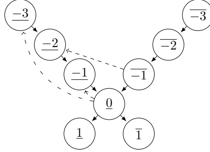
Fig. 1. A fragment of the frame \mathcal{X} (circles and solid arrows). Consider a formula \Phi = yRw \wedge wRv \wedge xRv \Rightarrow xRy that forces edge (-1, -2) . When applied to x = w = \underline{0} , y = \underline{-1} and v = \underline{1} , it forces edge (\underline{0}, \underline{-1}) . Then, applied to x = \underline{0} , v = \underline{-1} , w = \underline{-2} and y = \underline{-3} it forces long edge (\underline{0}, \underline{-3}) .
