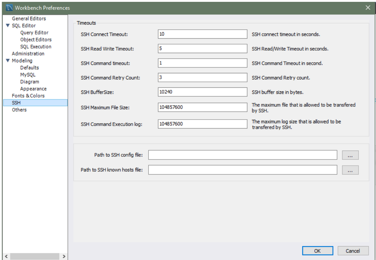
Figure 3.17 Preferences: SSH
