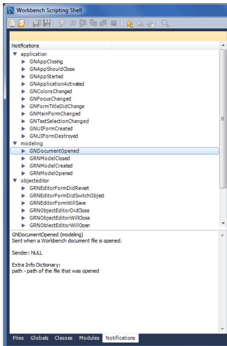
Figure C.7 The Workbench Scripting Shell Tab: Notifications
