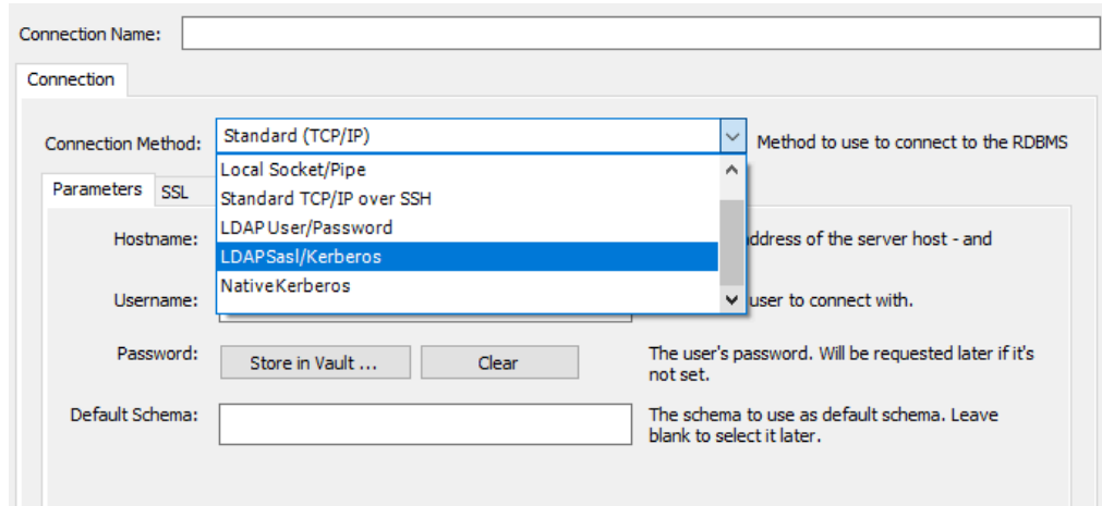
Figure 5.16 Manage Server Connections - LDAP and Kerberos Authentication
