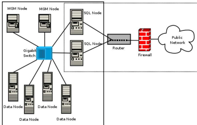
Figure 17.7 MySQL Cluster with Hardware Firewall
