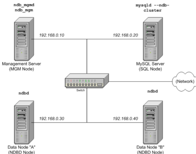
Figure 17.4 MySQL Cluster Multi-Computer Setup
