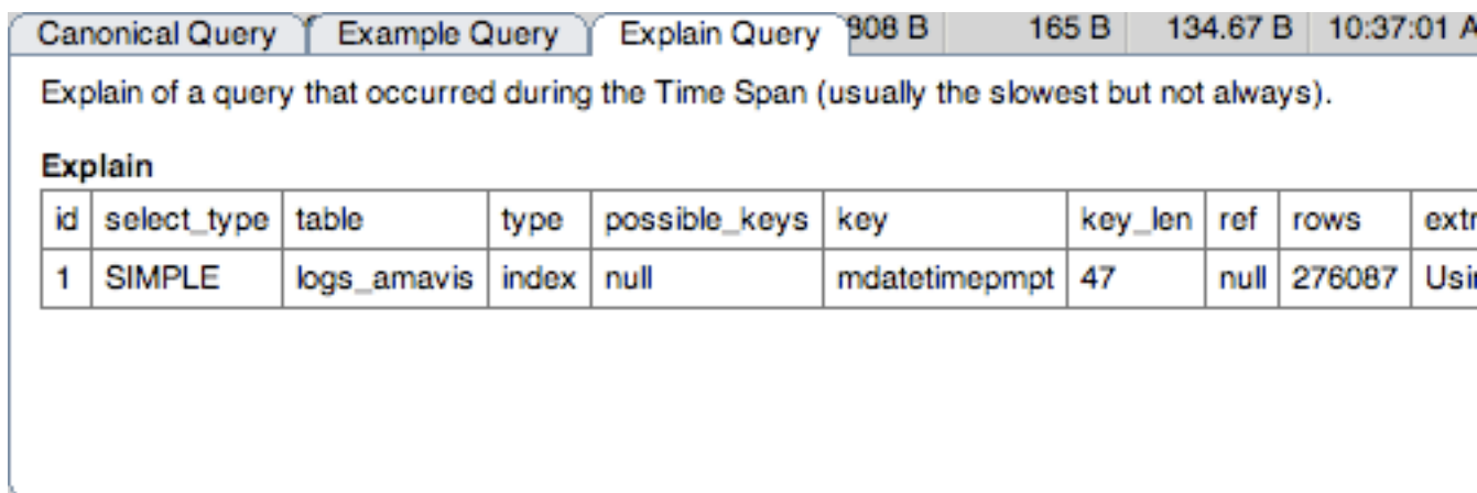
Figure 8.6 MySQL Enterprise Monitor User Interface: Explain Query Tab for a Query
