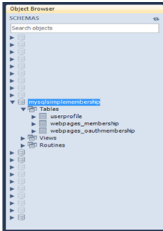
Figure 4.9 Simple Membership: Generated Schema and Tables
