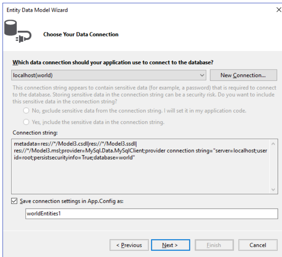
Figure 4.12 Entity Data Model Wizard - Connection
